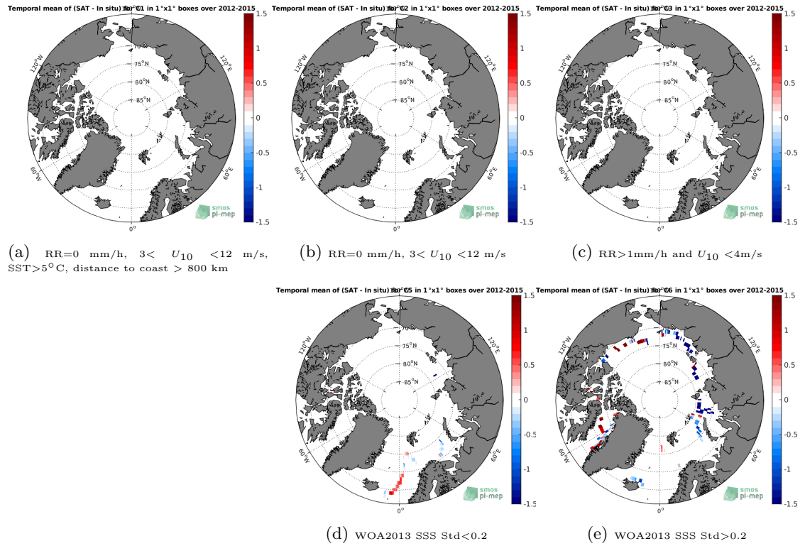
Figure 12: Temporal mean gridded over spatial boxes of size 1^\circ \times 1^\circ of \Delta SSS (SMOS-L3-CATDS-CECOS-LOCEAN-V4-9DAYS-25KM - TSG-GOSUD-Sailing-ship) for 5 different subdatasets corresponding to:RR=0 mm/h, 3 < U_{10} < 12 m/s, SST >5^\circ\text{C} , distance to coast > 800 km (a), RR=0 mm/h, 3 < U_{10} < 12 m/s (b), RR >1 mm/h and U_{10} < 4 m/s (c), WOA2013 SSS Std <0.2 (d), WOA2013 SSS Std >0.2 (e).
