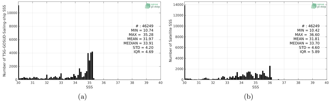
Figure 2: Histograms of SSS from TSG-GOSUD-Sailing-ship (a) and SMOS-L3-CATDS-CECOS-LOCEAN-V4-9DAYS-25KM (b) considering all match-up pairs per bins of 0.1 over the Arctic Ocean Pi-MEP region and for the full satellite product period.
