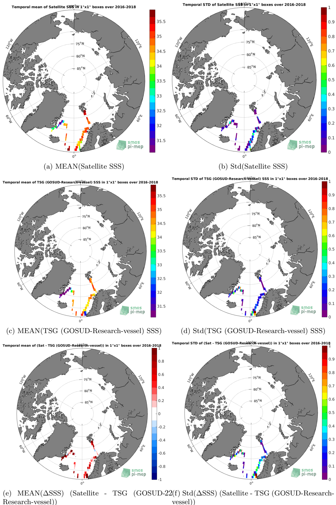
Figure 6: Temporal mean (left) and Std (right) of SSS from SMOS SSS L3 v4 - 9 Days (CATDS-CECOS-LOCEAN) (top), TSG (GOSUD-Research-vessel) (middle), and of \Delta SSS (Satellite - TSG (GOSUD-Research-vessel)). Only match-up pairs are used to generate these maps.
