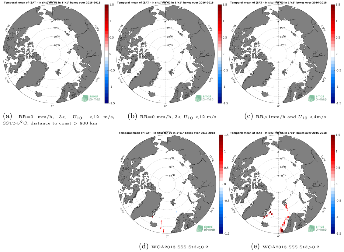
Figure 12: Temporal mean gridded over spatial boxes of size 1^\circ \times 1^\circ of \Delta SSS (SMOS SSS L3 v4 - 9 Days (CATDS-CECOS-LOCEAN) - TSG (GOSUD-Research-vessel)) for 5 different subdatasets corresponding to: RR=0 mm/h, 3 < U_{10} < 12 m/s, SST>5°C, distance to coast > 800 km (a), RR=0 mm/h, 3 < U_{10} < 12 m/s (b), RR>1mm/h and U_{10} < 4 m/s (c), WOA2013 SSS Std<0.2 (d), WOA2013 SSS Std>0.2 (e).
