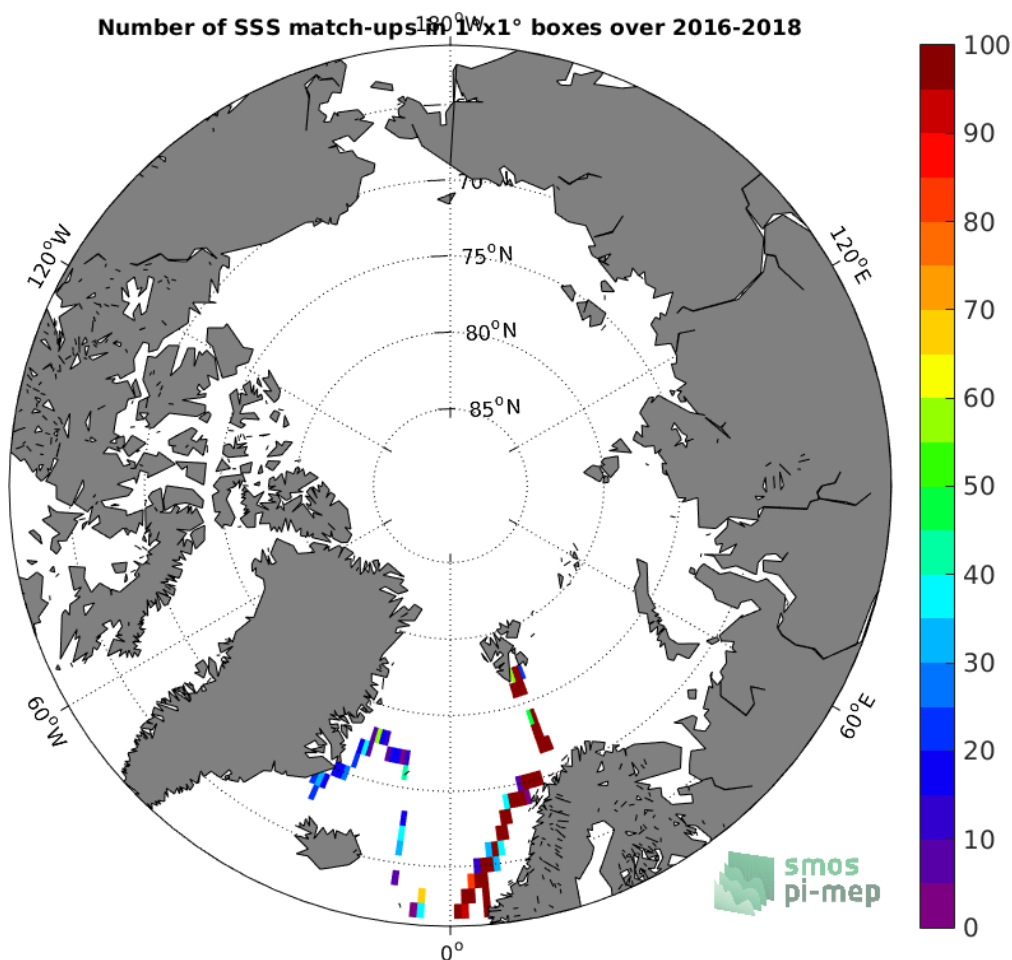
Figure 4: Number of SSS match-ups between TSG (GOSUD-Research-vessel) SSS and the SMOS SSS L3 v4 - 9 Days (CATDS-CECOS-LOCEAN) SSS product for the Arctic Ocean Pi-MEP region over 1°x1° boxes and for the full satellite product period.
