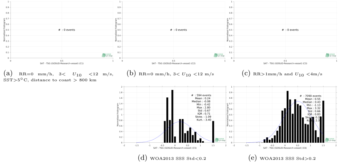
Figure 13: Normalized histogram of \Delta\text{SSS} (SMOS SSS L3 v4 - 9 Days (CATDS-CECOS-LOCEAN) - TSG (GOSUD-Research-vessel)) for 5 different subdatasets corresponding to: RR=0 mm/h, 3 < U_{10} < 12 m/s, SST > 5^\circ\text{C} , distance to coast > 800 km (a), RR=0 mm/h, 3 < U_{10} < 12 m/s (b), RR > 1\text{mm/h} and U_{10} < 4\text{m/s} (c), WOA2013 SSS Std<0.2 (d), WOA2013 SSS Std>0.2 (e).
