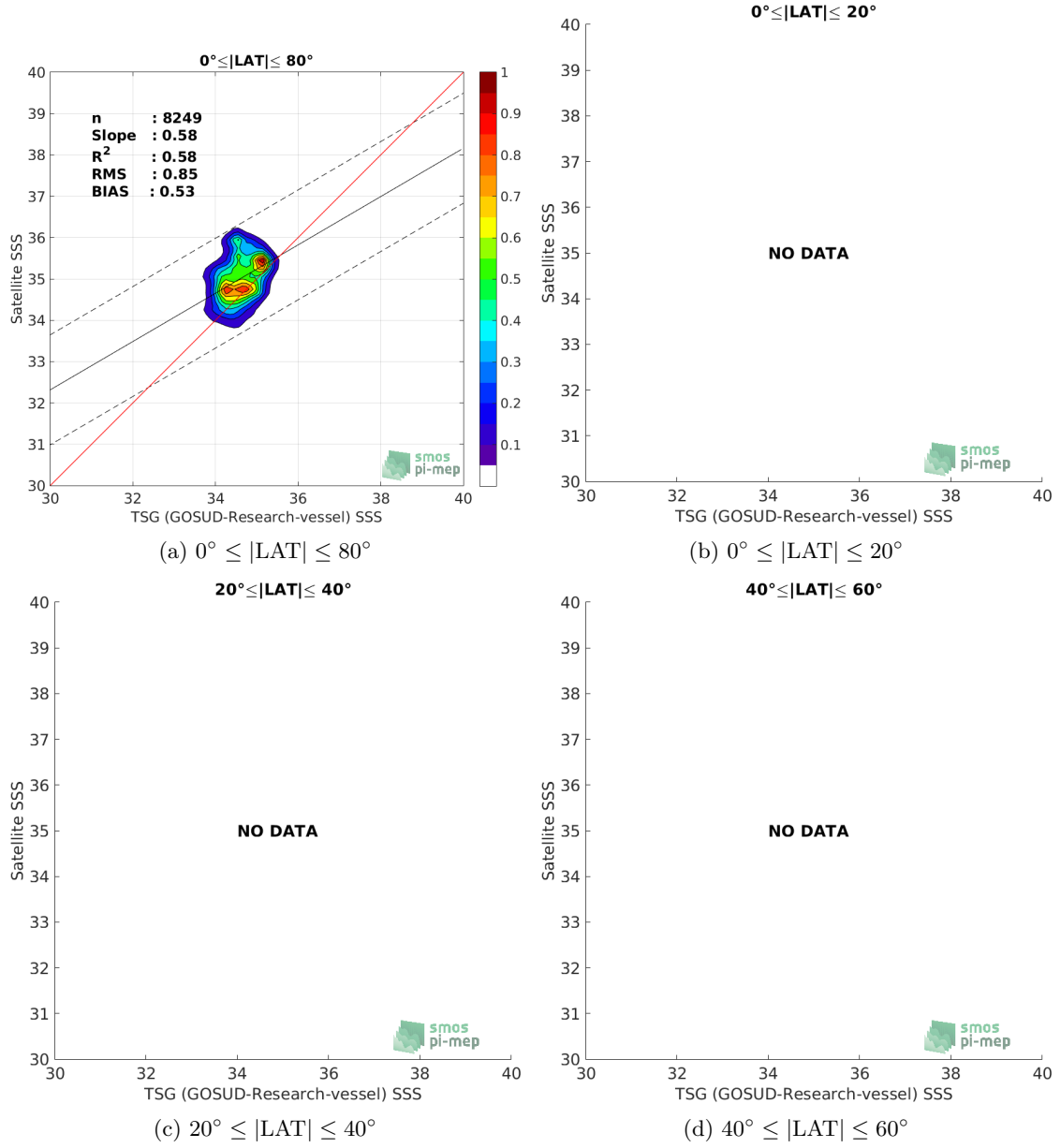
Figure 9: Contour maps of the concentration of SMOS SSS L3 v4 - 9 Days (CATDS-CECOS-LOCEAN) SSS (y-axis) versus TSG (GOSUD-Research-vessel) SSS (x-axis) at match-up pairs for different latitude bands. For each plot, the red line shows x=y . The black thin and dashed lines indicate a linear fit through the data cloud and the \pm 95\% confidence levels, respectively. The number match-up pairs n , the slope and R^2 coefficient of the linear fit, the root mean square (RMS) and the mean bias between satellite and in situ data are indicated for each latitude band in each plots.
