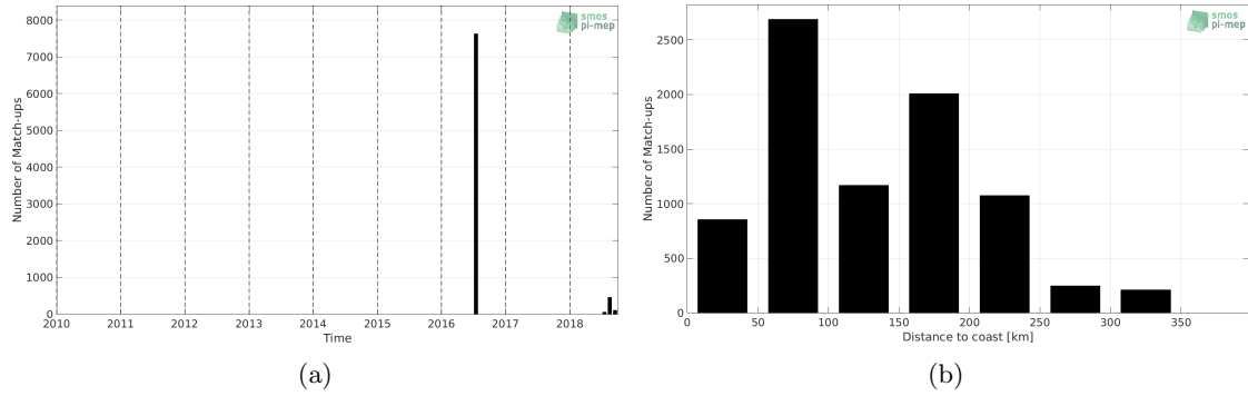
Figure 1: Number of match-ups between TSG (GOSUD-Research-vessel) and SMOS SSS L3 v4 - 9 Days (CATDS-CECOS-LOCEAN) SSS as a function of time (a) and as function of the distance to coast (b) over the Arctic Ocean Pi-MEP region and for the full satellite product period.
