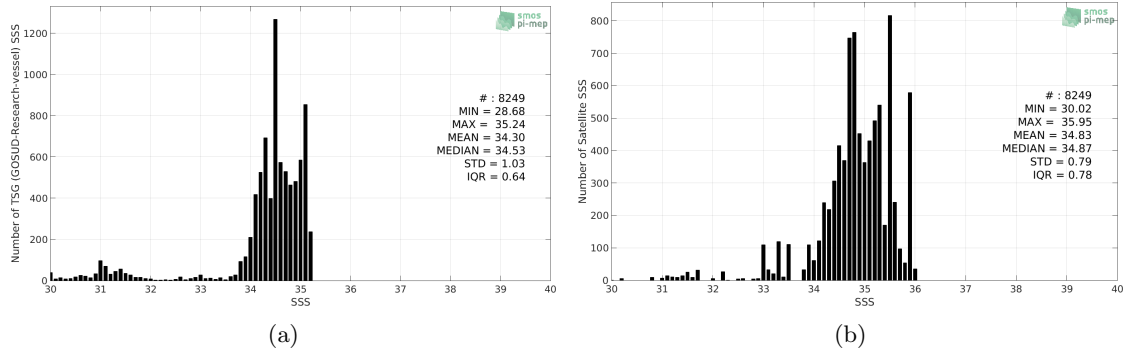
Figure 2: Histograms of SSS from TSG (GOSUD-Research-vessel) (a) and SMOS SSS L3 v4 - 9 Days (CATDS-CECOS-LOCEAN) (b) considering all match-up pairs per bins of 0.1 over the Arctic Ocean Pi-MEP region and for the full satellite product period.
