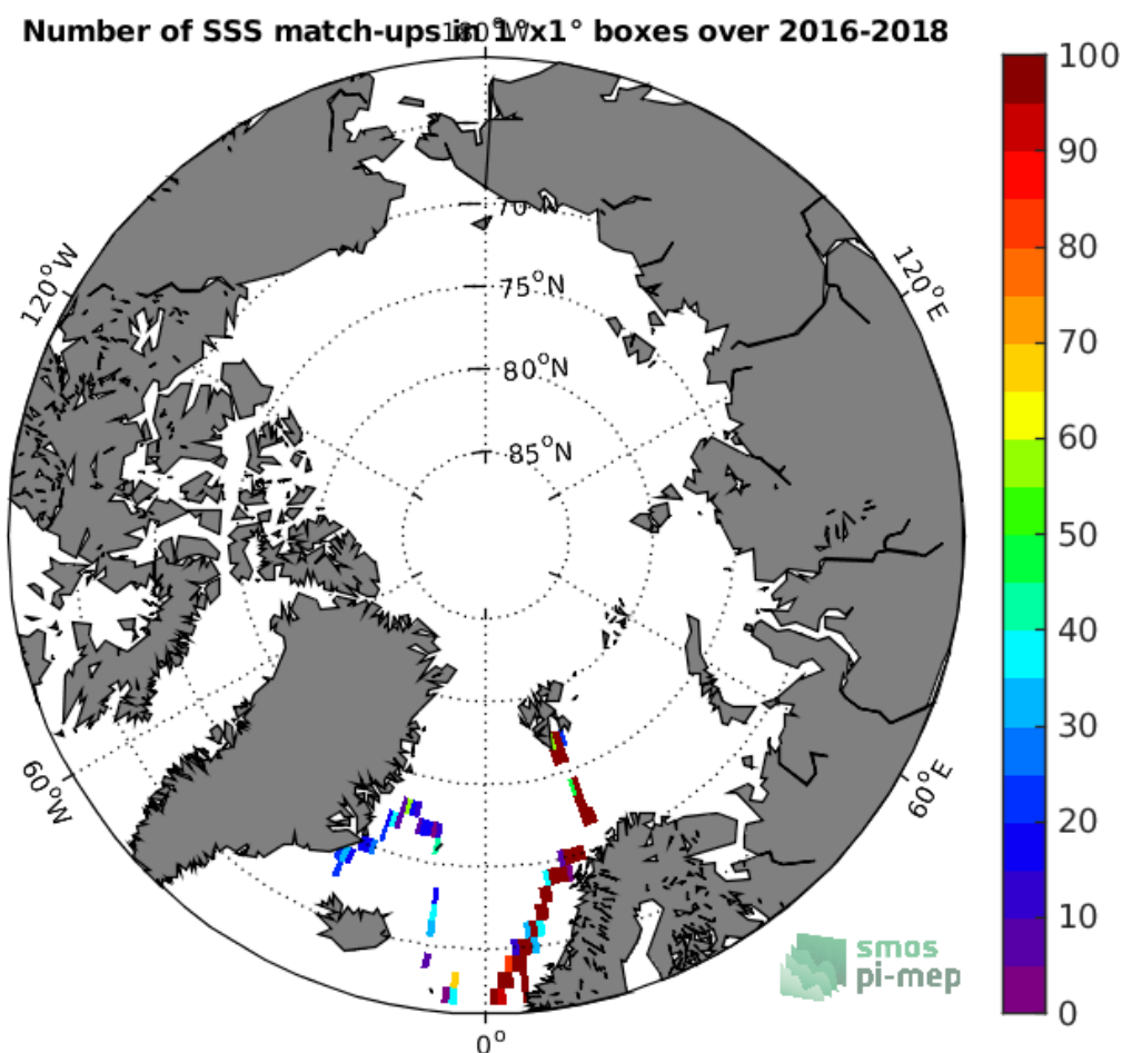
Figure 4: Number of SSS match-ups between TSG-GOSUD-Research-vessel SSS and the SMOS-L3-CATDS-CECOS-LOCEAN-V4-9DAYS-25KM SSS product for the Arctic Ocean Pi-MEP region over 1°x1° boxes and for the full satellite product period.
