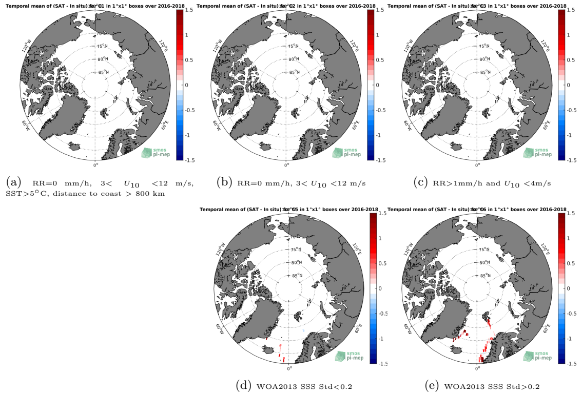
Figure 12: Temporal mean gridded over spatial boxes of size 1^\circ \times 1^\circ of \Delta SSS (SMOS-L3-CATDS-CECOS-LOCEAN-V4-9DAYS-25KM - TSG-GOSUD-Research-vessel) for 5 different subdatasets corresponding to:RR=0 mm/h, 3 < U_{10} < 12 m/s, SST>5°C, distance to coast > 800 km (a), RR=0 mm/h, 3 < U_{10} < 12 m/s (b), RR>1mm/h and U_{10} < 4 m/s (c), WOA2013 SSS Std<0.2 (d), WOA2013 SSS Std>0.2 (e).
