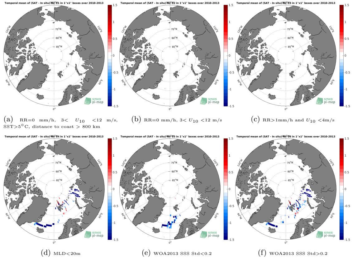
Figure 12: Temporal mean gridded over spatial boxes of size 1^{\circ}\times 1^{\circ} of \Delta\text{SSS} (SMOS SSS L3 v4 - 9 Days (CATDS-CECOS-LOCEAN) - Sea mammals) for 6 different subdatasets corresponding to: RR=0 mm/h, 3 < U_{10} < 12 m/s, SST >5^{\circ}\text{C} , distance to coast > 800 km (a), RR=0 mm/h, 3 < U_{10} < 12 m/s (b), RR >1\text{mm/h} and U_{10} < 4\text{m/s} (c), MLD <20\text{m} (d), WOA2013 SSS Std <0.2 (e), WOA2013 SSS Std >0.2 (f).
