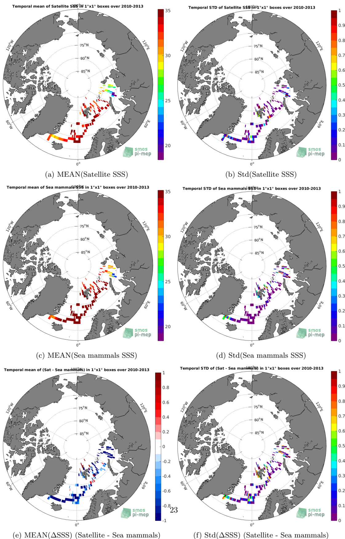
Figure 6: Temporal mean (left) and Std (right) of SSS from SMOS SSS L3 v4 - 9 Days (CATDS-CECOS-LOCEAN) (top), Sea mammals (middle), and of \Delta SSS (Satellite - Sea mammals). Only match-up pairs are used to generate these maps.
