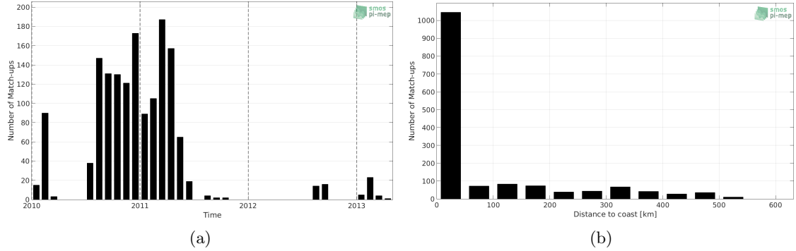
Figure 1: Number of match-ups between Sea mammals and SMOS SSS L3 v4 - 9 Days (CATDS-CECOS-LOCEAN) SSS as a function of time (a) and as function of the distance to coast (b) over the Arctic Ocean Pi-MEP region and for the full satellite product period.
