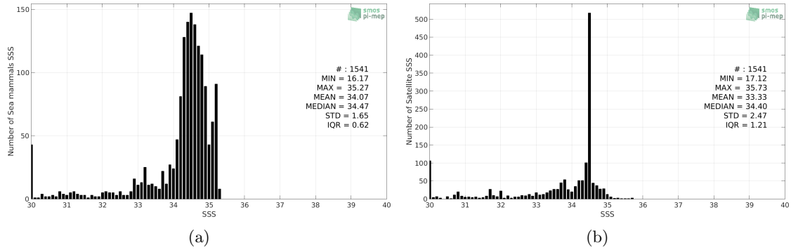
Figure 2: Histograms of SSS from Sea mammals (a) and SMOS SSS L3 v4 - 9 Days (CATDS-CECOS-LOCEAN) (b) considering all match-up pairs per bins of 0.1 over the Arctic Ocean Pi-MEP region and for the full satellite product period.
