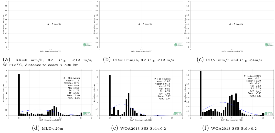
Figure 13: Normalized histogram of \Delta\text{SSS} (SMOS SSS L3 v4 - 9 Days (CATDS-CECOS-LOCEAN) - Sea mammals) for 6 different subdatasets corresponding to: RR=0 mm/h, 3 < U_{10} < 12 m/s, SST > 5^\circ\text{C} , distance to coast > 800 km (a), RR=0 mm/h, 3 < U_{10} < 12 m/s (b), RR > 1 mm/h and U_{10} < 4 m/s (c), MLD < 20 m (d), WOA2013 SSS Std < 0.2 (e), WOA2013 SSS Std > 0.2 (f).
