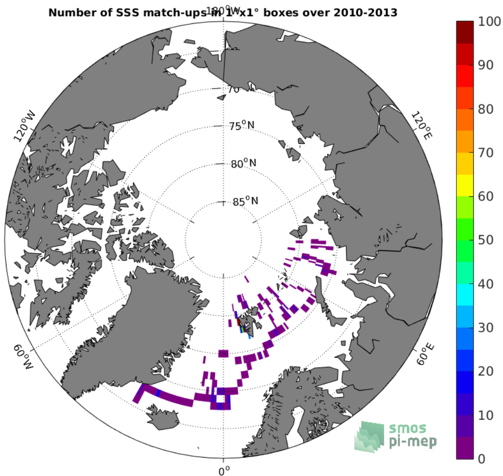
Figure 4: Number of SSS match-ups between Sea mammals SSS and the SMOS SSS L3 v4 - 9 Days (CATDS-CECOS-LOCEAN) SSS product for the Arctic Ocean Pi-MEP region over 1°x1° boxes and for the full satellite product period.
