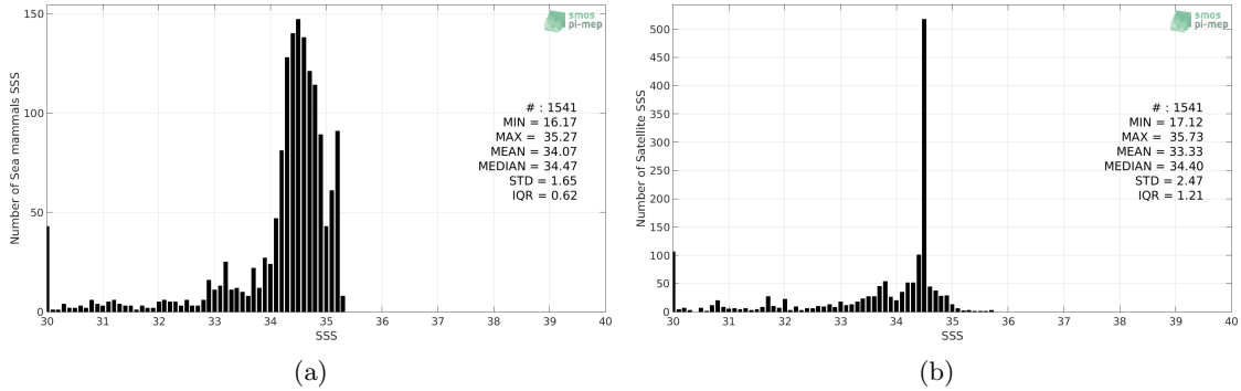
Figure 2: Histograms of SSS from Sea mammals (a) and SMOS-L3-CATDS-CECOS-LOCEAN-V4-9DAYS-25KM (b) considering all match-up pairs per bins of 0.1 over the Arctic Ocean Pi-MEP region and for the full satellite product period.
