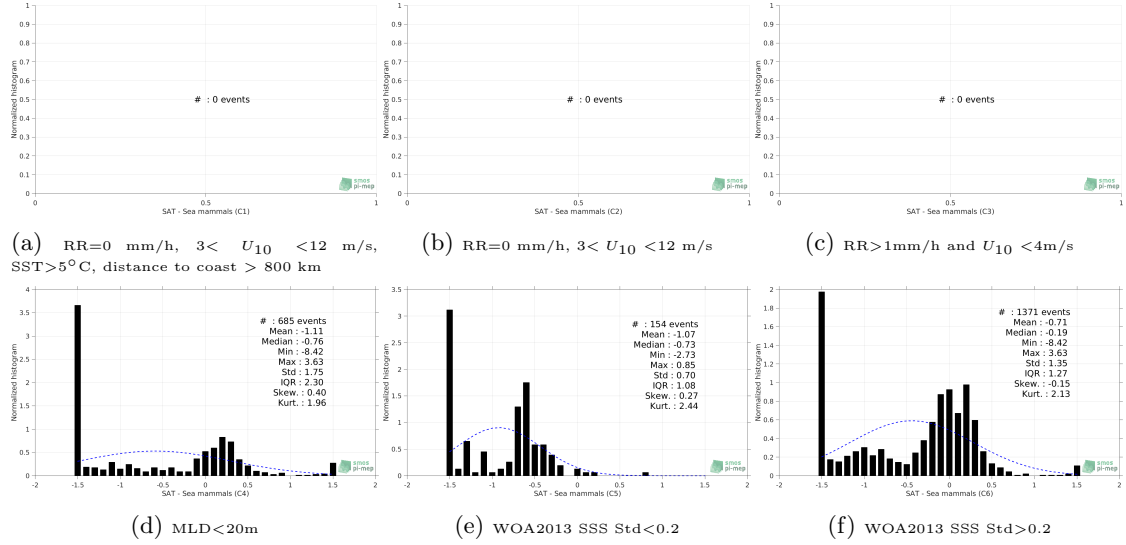
Figure 13: Normalized histogram of \Delta\text{SSS} (SMOS-L3-CATDS-CECOS-LOCEAN-V4-9DAYS-25KM - Sea mammals) for 6 different subdatasets corresponding to: RR=0 mm/h, 3 < U_{10} < 12 m/s, SST > 5^{\circ}\text{C} , distance to coast > 800 km (a), RR=0 mm/h, 3 < U_{10} < 12 m/s (b), RR > 1\text{mm/h} and U_{10} < 4\text{m/s} (c), MLD < 20\text{m} (d), WOA2013 SSS Std < 0.2 (e), WOA2013 SSS Std > 0.2 (f).
