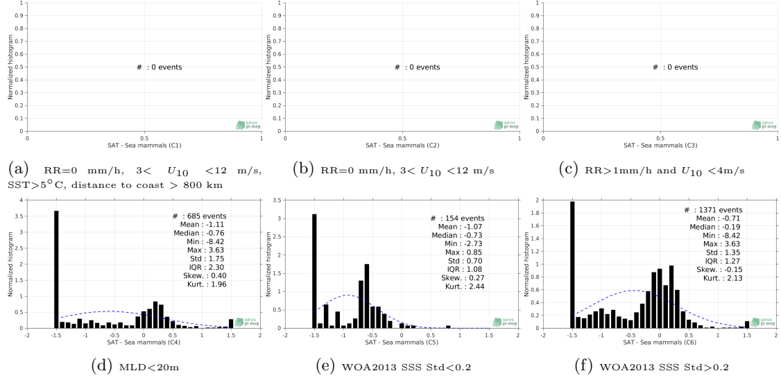
Figure 13: Normalized histogram of \Delta\text{SSS} (SMOS-L3-CATDS-CECOS-LOCEAN-V4-9DAYS-25KM - Sea mammals) for 6 different subdatasets corresponding to: RR=0 mm/h, 3 < U_{10} < 12 m/s, SST > 5^{\circ}\text{C} , distance to coast > 800 km (a), RR=0 mm/h, 3 < U_{10} < 12 m/s (b), RR > 1\text{mm/h} and U_{10} < 4\text{m/s} (c), MLD < 20\text{m} (d), WOA2013 SSS Std < 0.2 (e), WOA2013 SSS Std > 0.2 (f).
