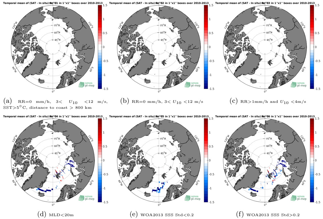
Figure 12: Temporal mean gridded over spatial boxes of size 1^\circ \times 1^\circ of \Delta SSS (SMOS-L3-CATDS-CECOS-LOCEAN-V4-9DAYS-25KM - Sea mammals) for 6 different subdatasets corresponding to: RR=0 mm/h, 3 < U_{10} < 12 m/s, SST >5^\circ\text{C} , distance to coast > 800 km (a), RR=0 mm/h, 3 < U_{10} < 12 m/s (b), RR >1 mm/h and U_{10} < 4 m/s (c),MLD <20 m (d),WOA2013 SSS Std <0.2 (e),WOA2013 SSS Std >0.2 (f).
