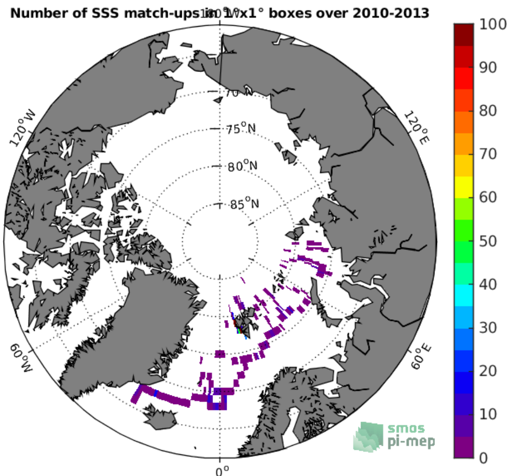
Figure 4: Number of SSS match-ups between Sea mammals SSS and the SMOS-L3-CATDS-CECOS-LOCEAN-V4-9DAYS-25KM SSS product for the Arctic Ocean Pi-MEP region over 1°x1° boxes and for the full satellite product period.
