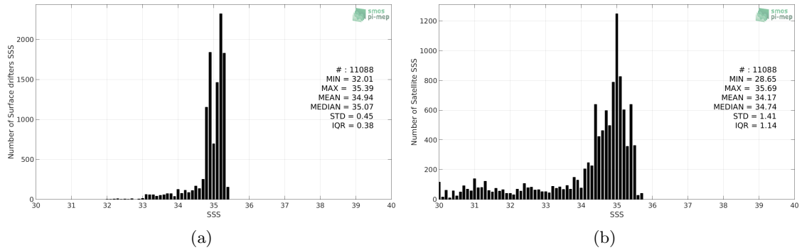
Figure 2: Histograms of SSS from Surface drifters (a) and SMOS SSS L3 v4 - 9 Days (CATDS-CECOS-LOCEAN) (b) considering all match-up pairs per bins of 0.1 over the Arctic Ocean Pi-MEP region and for the full satellite product period.
