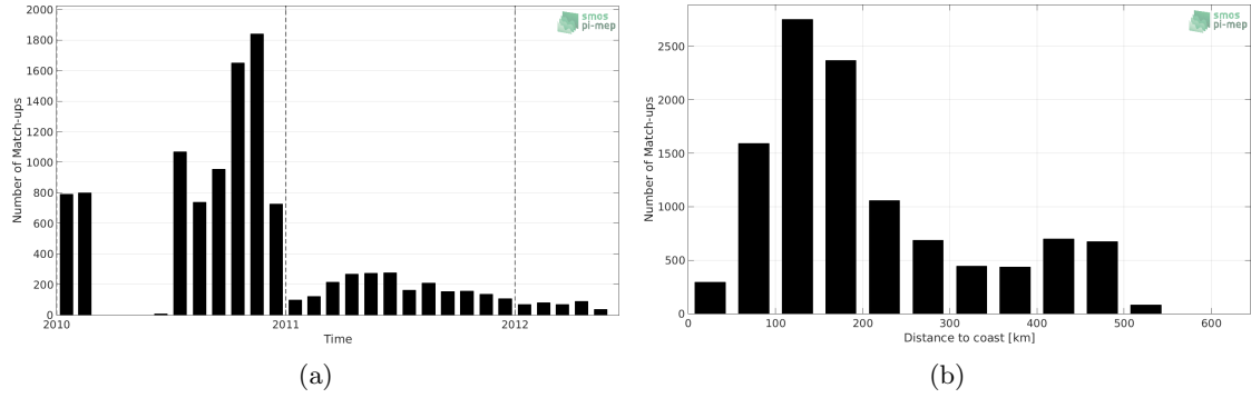
Figure 1: Number of match-ups between Surface drifters and SMOS SSS L3 v4 - 9 Days (CATDS-CECOS-LOCEAN) SSS as a function of time (a) and as function of the distance to coast (b) over the Arctic Ocean Pi-MEP region and for the full satellite product period.
