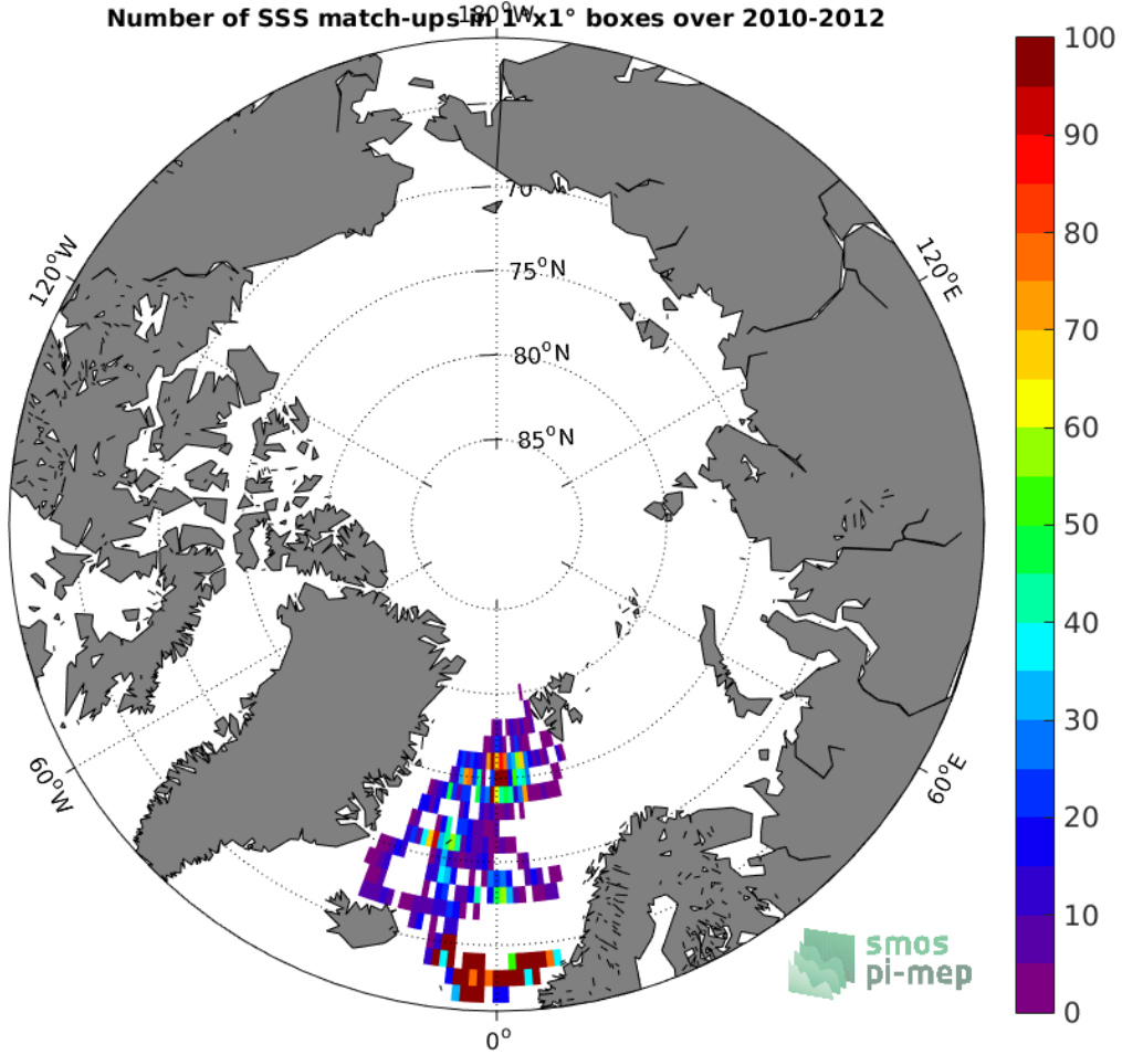
Figure 3: Number of SSS match-ups between Surface drifters SSS and the SMOS SSS L3 v4 - 9 Days (CATDS-CECOS-LOCEAN) SSS product for the Arctic Ocean Pi-MEP region over 1°x1° boxes and for the full satellite product period.
