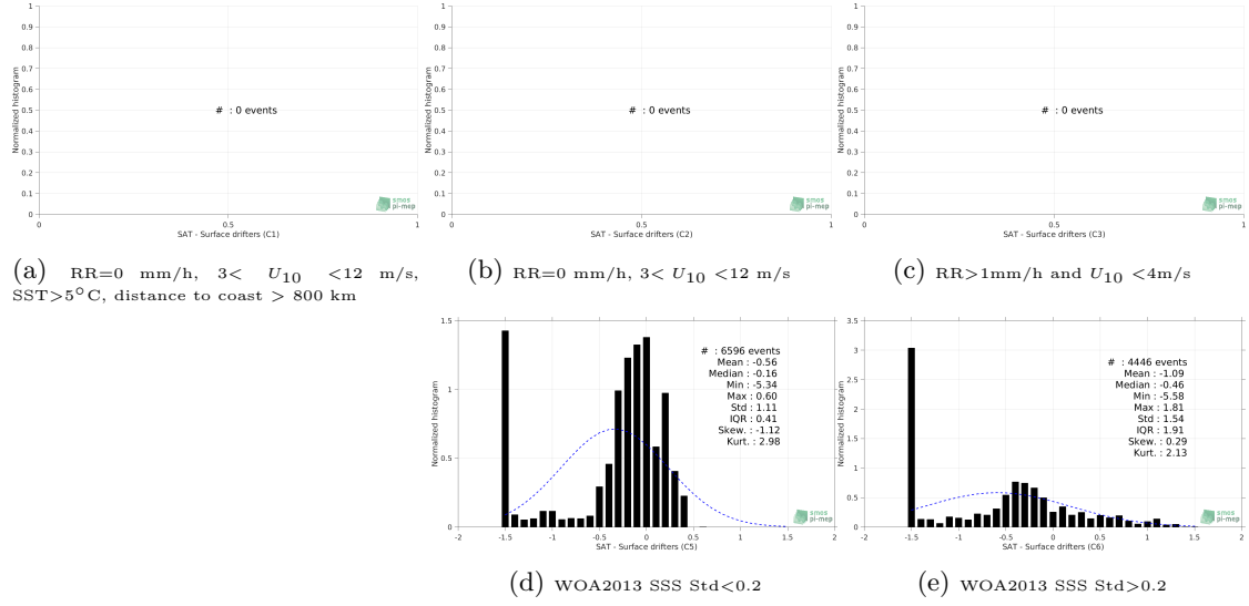
Figure 12: Normalized histogram of \Delta\text{SSS} (SMOS SSS L3 v4 - 9 Days (CATDS-CECOS-LOCEAN) - Surface drifters) for 5 different subdatasets corresponding to: RR=0 mm/h, 3 < U_{10} < 12 m/s, SST > 5^\circ\text{C} , distance to coast > 800 km (a), RR=0 mm/h, 3 < U_{10} < 12 m/s (b), RR > 1\text{mm/h} and U_{10} < 4\text{m/s} (c), WOA2013 SSS Std<0.2 (d), WOA2013 SSS Std>0.2 (e).
