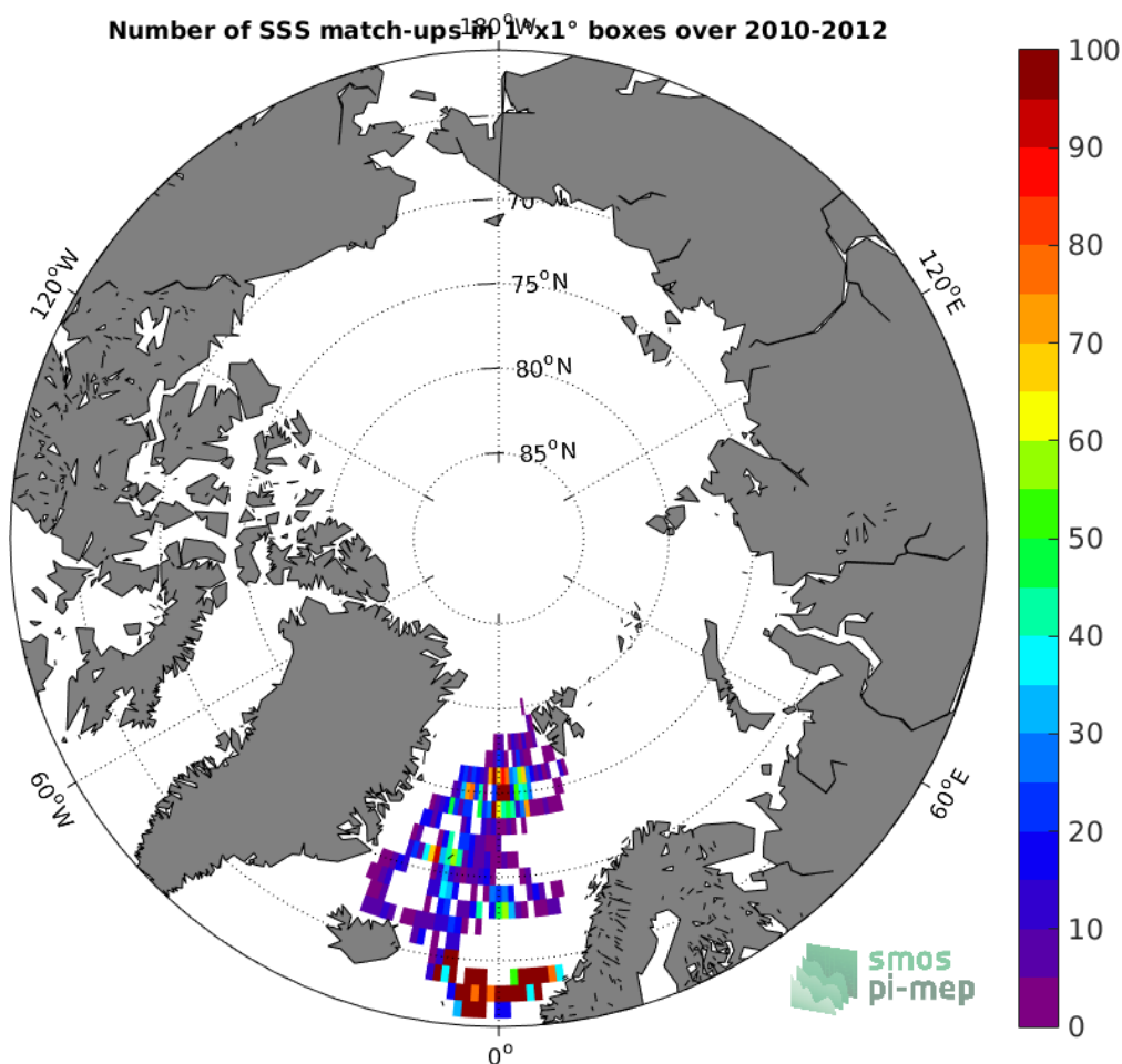
Figure 3: Number of SSS match-ups between Surface drifters SSS and the SMOS-L3-CATDS-CECOS-LOCEAN-V4-9DAYS-25KM SSS product for the Arctic Ocean Pi-MEP region over 1^\circ \times 1^\circ boxes and for the full satellite product period.
