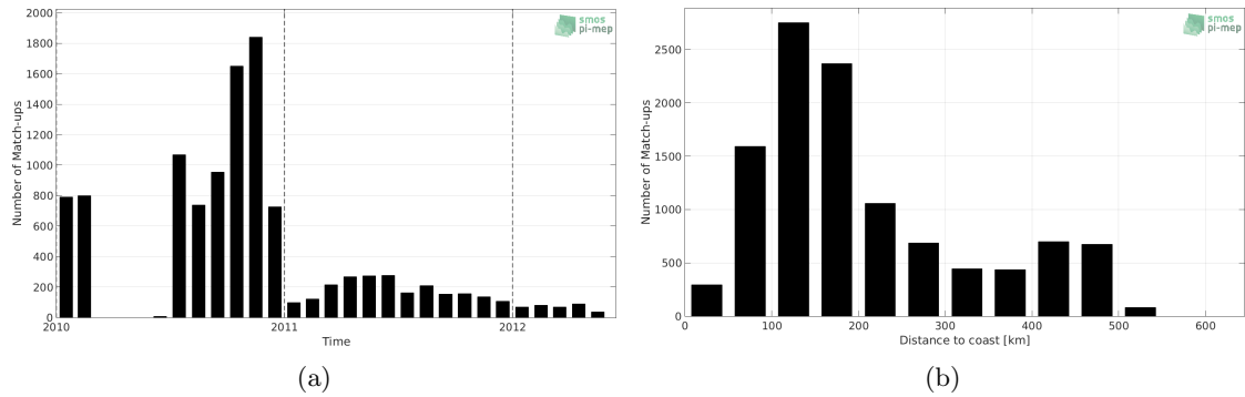
Figure 1: Number of match-ups between Surface drifters and SMOS-L3-CATDS-CECOS-LOCEAN-V4-9DAYS-25KM SSS as a function of time (a) and as function of the distance to coast (b) over the Arctic Ocean Pi-MEP region and for the full satellite product period.
