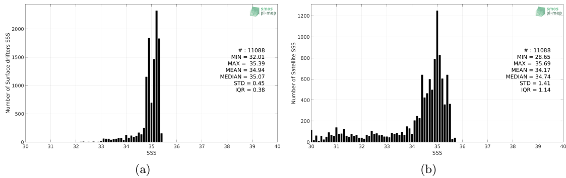
Figure 2: Histograms of SSS from Surface drifters (a) and SMOS-L3-CATDS-CECOS-LOCEAN-V4-9DAYS-25KM (b) considering all match-up pairs per bins of 0.1 over the Arctic Ocean Pi-MEP region and for the full satellite product period.
