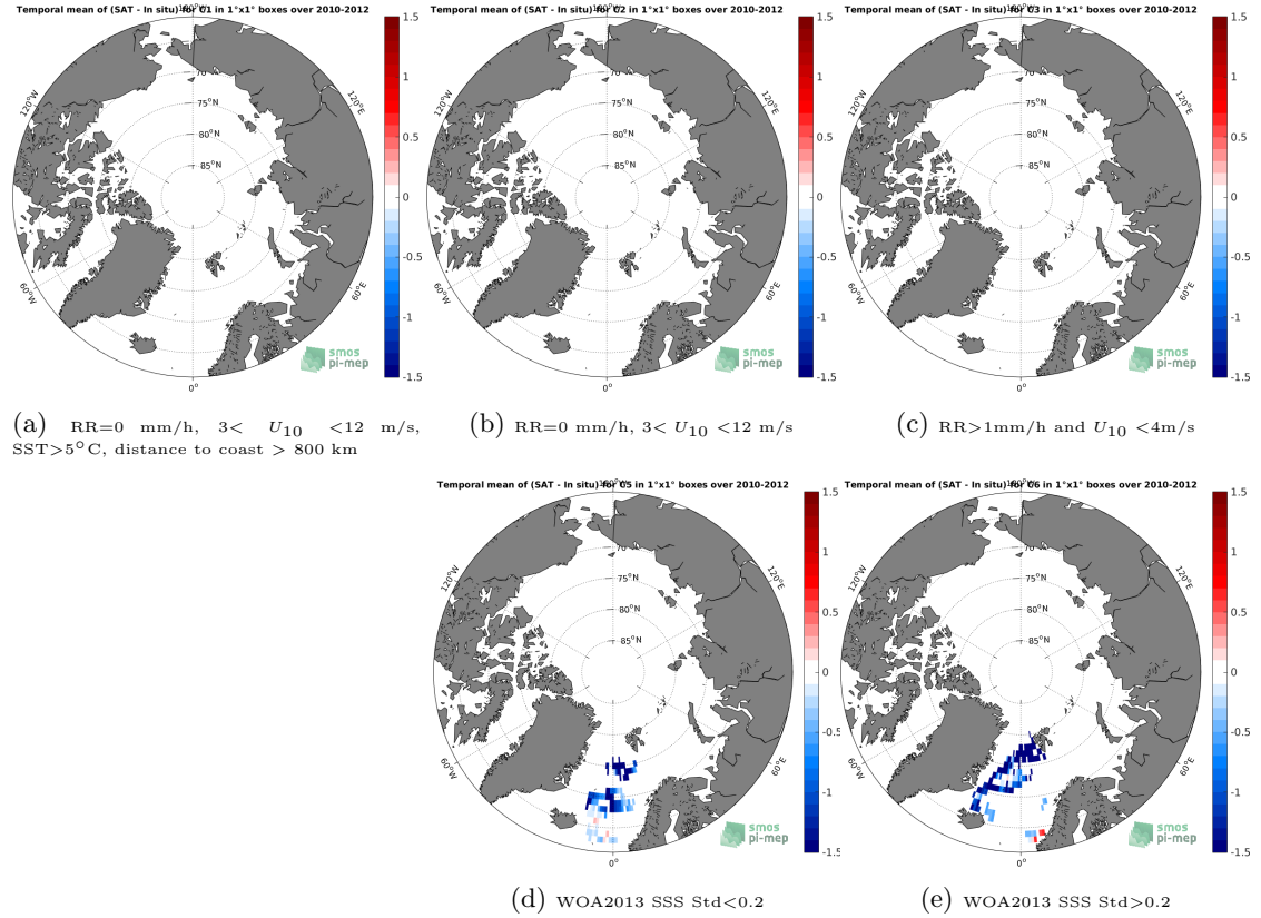
Figure 11: Temporal mean gridded over spatial boxes of size 1^{\circ}\times 1^{\circ} of \Delta\text{SSS} (SMOS-L3-CATDS-CECOS-LOCEAN-V4-9DAYS-25KM - Surface drifters) for 5 different subdatasets corresponding to: \text{RR}=0 mm/h, 3 < U_{10} < 12 m/s, \text{SST} > 5^{\circ}\text{C} , distance to coast > 800 km (a), \text{RR}=0 mm/h, 3 < U_{10} < 12 m/s (b), \text{RR} > 1 mm/h and U_{10} < 4 m/s (c), WOA2013 SSS Std < 0.2 (d), WOA2013 SSS Std > 0.2 (e).
