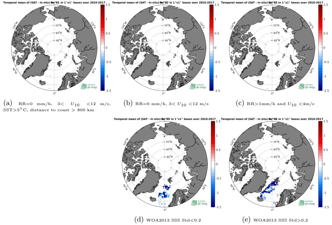
Figure 11: Temporal mean gridded over spatial boxes of size 1^\circ \times 1^\circ of \Delta SSS (SMOS-L3-CATDS-CECOS-LOCEAN-V4-9DAYS-25KM - Surface drifters) for 5 different subdatasets corresponding to: RR=0 mm/h, 3 < U_{10} < 12 m/s, SST >5^\circ C, distance to coast > 800 km (a), RR=0 mm/h, 3 < U_{10} < 12 m/s (b), RR >1 mm/h and U_{10} < 4 m/s (c), WOA2013 SSS Std <0.2 (d), WOA2013 SSS Std >0.2 (e).
