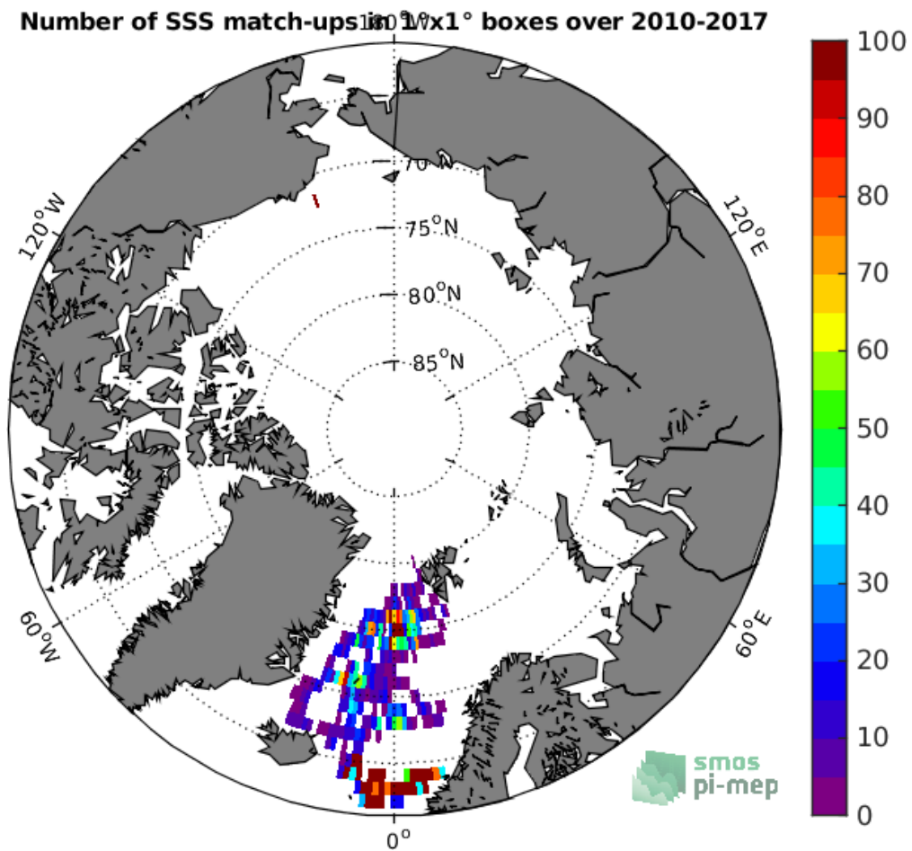
Figure 3: Number of SSS match-ups between Surface drifters SSS and the SMOS-L3-CATDS-CECOS-LOCEAN-V4-9DAYS-25KM SSS product for the Arctic Ocean Pi-MEP region over 1°x1° boxes and for the full satellite product period.
