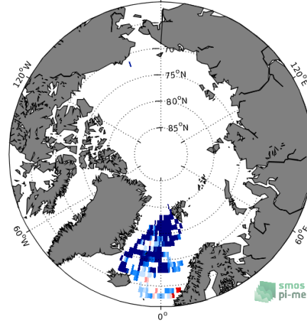
(e) MEAN( \Delta SSS) (Satellite - Surface drifters)
