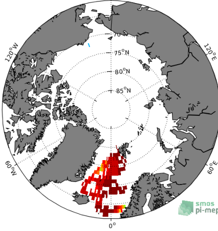
(c) MEAN(Surface drifters SSS)
