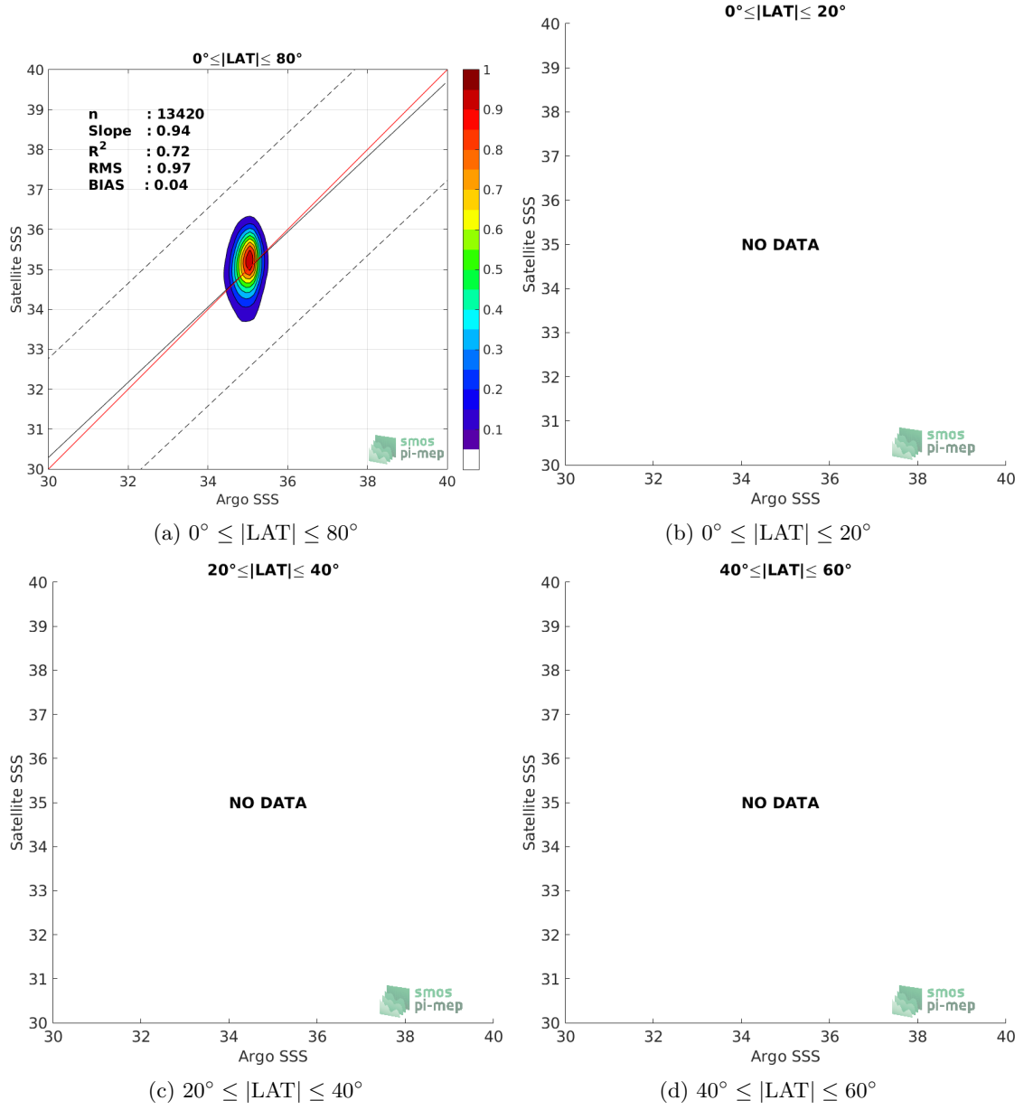
Figure 9: Contour maps of the concentration of SMOS SSS L3 v4 - 9 Days (CATDS-CECOS-LOCEAN) SSS (y-axis) versus Argo SSS (x-axis) at match-up pairs for different latitude bands. For each plot, the red line shows x=y . The black thin and dashed lines indicate a linear fit through the data cloud and the \pm 95\% confidence levels, respectively. The number match-up pairs n , the slope and R^2 coefficient of the linear fit, the root mean square (RMS) and the mean bias between satellite and in situ data are indicated for each latitude band in each plots.
