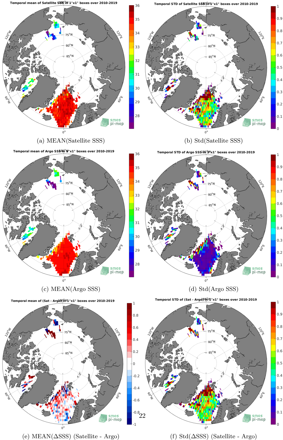
Figure 6: Temporal mean (left) and Std (right) of SSS from SMOS SSS L3 v4 - 9 Days (CATDS-CECOS-LOCEAN) (top), Argo (middle), and of \Delta SSS (Satellite - Argo). Only match-up pairs are used to generate these maps.
