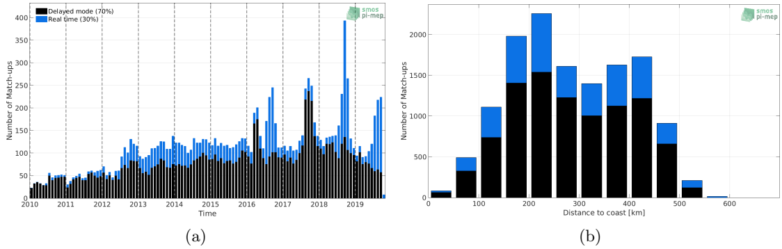
Figure 1: Number of match-ups between Argo and SMOS SSS L3 v4 - 9 Days (CATDS-CECOS-LOCEAN) SSS as a function of time (a) and as function of the distance to coast (b) over the Arctic Ocean Pi-MEP region and for the full satellite product period.
