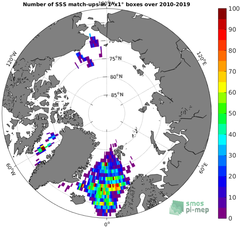
Figure 4: Number of SSS match-ups between Argo SSS and the SMOS SSS L3 v4 - 9 Days (CATDS-CECOS-LOCEAN) SSS product for the Arctic Ocean Pi-MEP region over 1°x1° boxes and for the full satellite product period.
