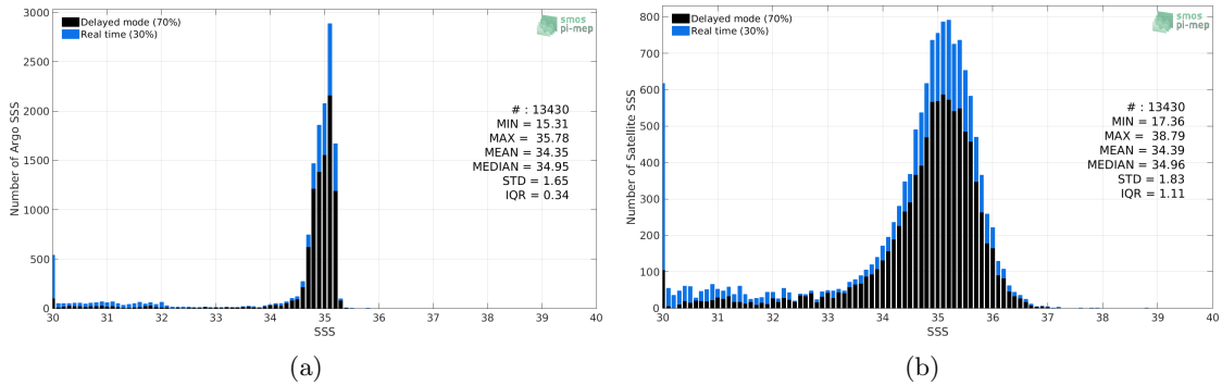
Figure 2: Histograms of SSS from Argo (a) and SMOS SSS L3 v4 - 9 Days (CATDS-CECOS-LOCEAN) (b) considering all match-up pairs per bins of 0.1 over the Arctic Ocean Pi-MEP region and for the full satellite product period.
