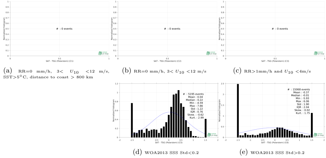
Figure 13: Normalized histogram of \Delta\text{SSS} (SMOS SSS L3 v4 - 18 Days (CATDS-CECOS-LOCEAN) - TSG (Polarstern)) for 5 different subdatasets corresponding to: RR=0 mm/h, 3 < U_{10} < 12 m/s, SST > 5^\circ\text{C} , distance to coast > 800 km (a), RR=0 mm/h, 3 < U_{10} < 12 m/s (b), RR > 1 mm/h and U_{10} < 4 m/s (c), WOA2013 SSS Std < 0.2 (d), WOA2013 SSS Std > 0.2 (e).
