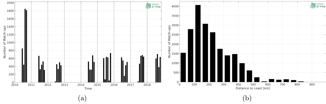
Figure 1: Number of match-ups between TSG (Polarstern) and SMOS SSS L3 v4 - 18 Days (CATDS-CECOS-LOCEAN) SSS as a function of time (a) and as function of the distance to coast (b) over the Arctic Ocean Pi-MEP region and for the full satellite product period.
