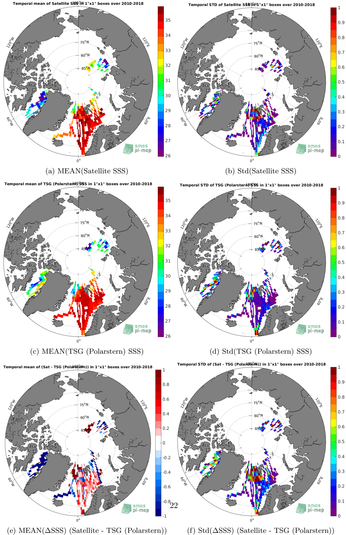
Figure 6: Temporal mean (left) and Std (right) of SSS from SMOS SSS L3 v4 - 18 Days (CATDS-CECOS-LOCEAN) (top), TSG (Polarstern) (middle), and of \Delta SSS (Satellite - TSG (Polarstern)). Only match-up pairs are used to generate these maps.
