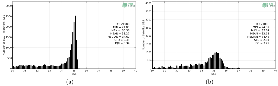
Figure 2: Histograms of SSS from TSG (Polarstern) (a) and SMOS SSS L3 v4 - 18 Days (CATDS-CECOS-LOCEAN) (b) considering all match-up pairs per bins of 0.1 over the Arctic Ocean Pi-MEP region and for the full satellite product period.
