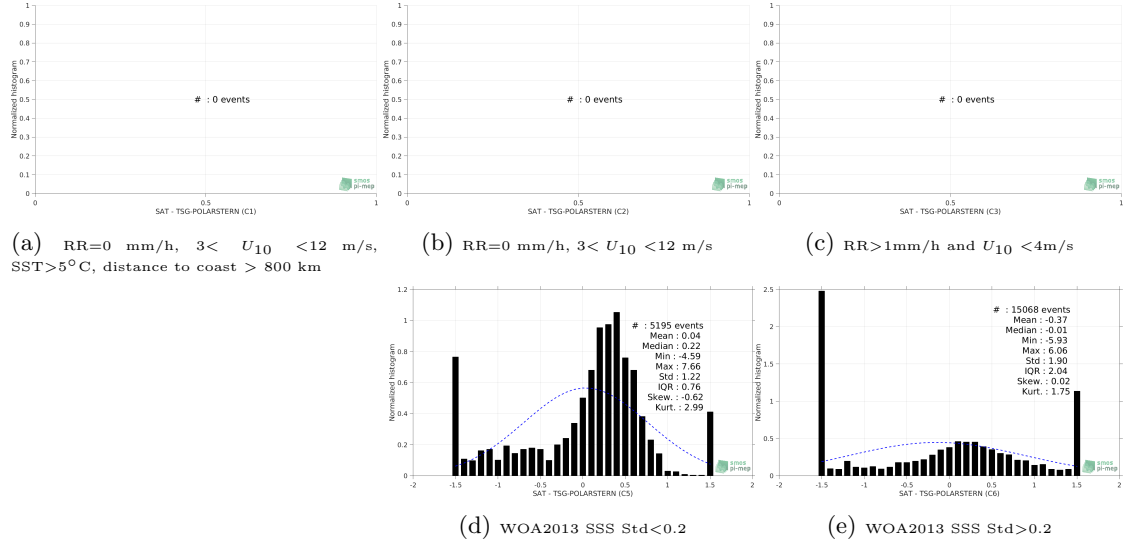
Figure 13: Normalized histogram of \Delta\text{SSS} (SMOS-L3-CATDS-CECOS-LOCEAN-V4-18DAYS-25KM - TSG-POLARSTERN) for 5 different subdatasets corresponding to: RR=0 mm/h, 3 < U_{10} < 12 m/s, SST > 5^\circ\text{C} , distance to coast > 800 km (a), RR=0 mm/h, 3 < U_{10} < 12 m/s (b), RR > 1\text{mm/h} and U_{10} < 4\text{m/s} (c), WOA2013 SSS Std < 0.2 (d), WOA2013 SSS Std > 0.2 (e).
