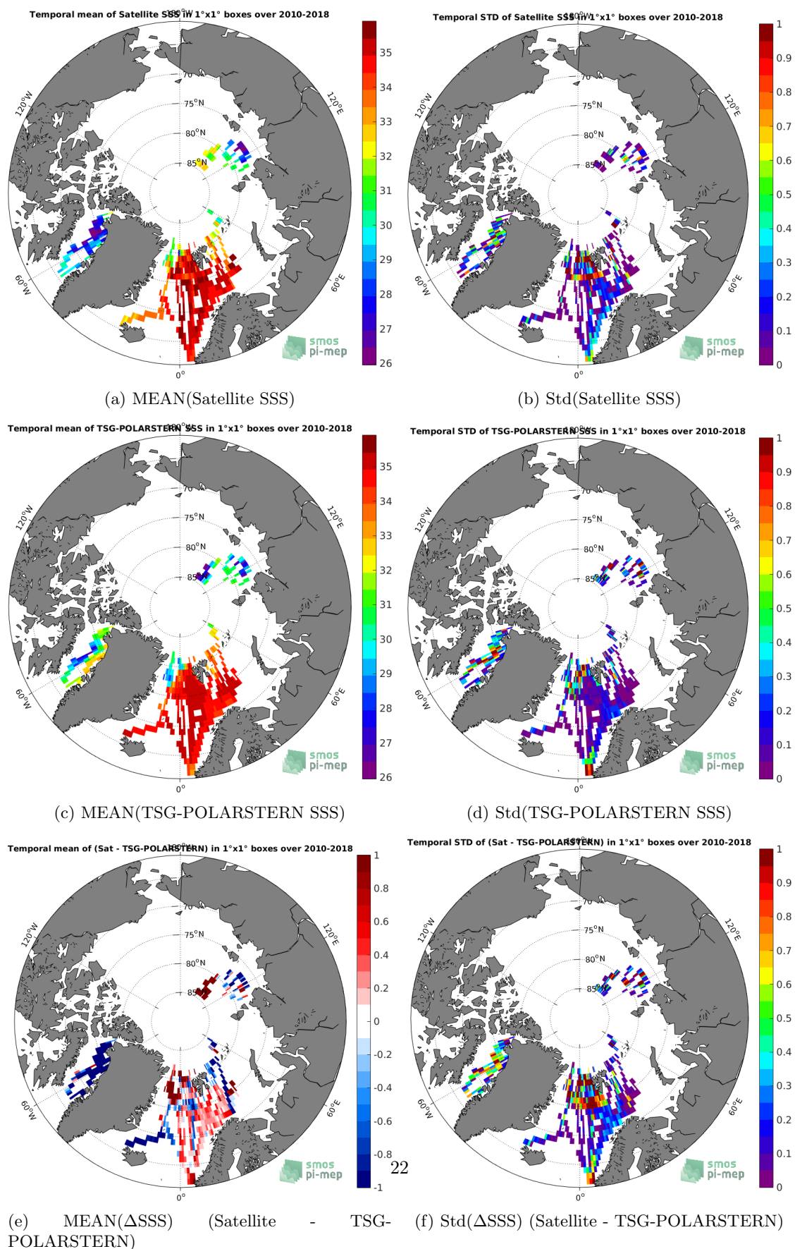
Figure 6: Temporal mean (left) and Std (right) of SSS from SMOS-L3-CATDS-CECOS-LOCEAN-V4-18DAYS-25KM (top), TSG-POLARSTERN (middle), and of \Delta SSS (Satellite - TSG-POLARSTERN). Only match-up pairs are used to generate these maps.
