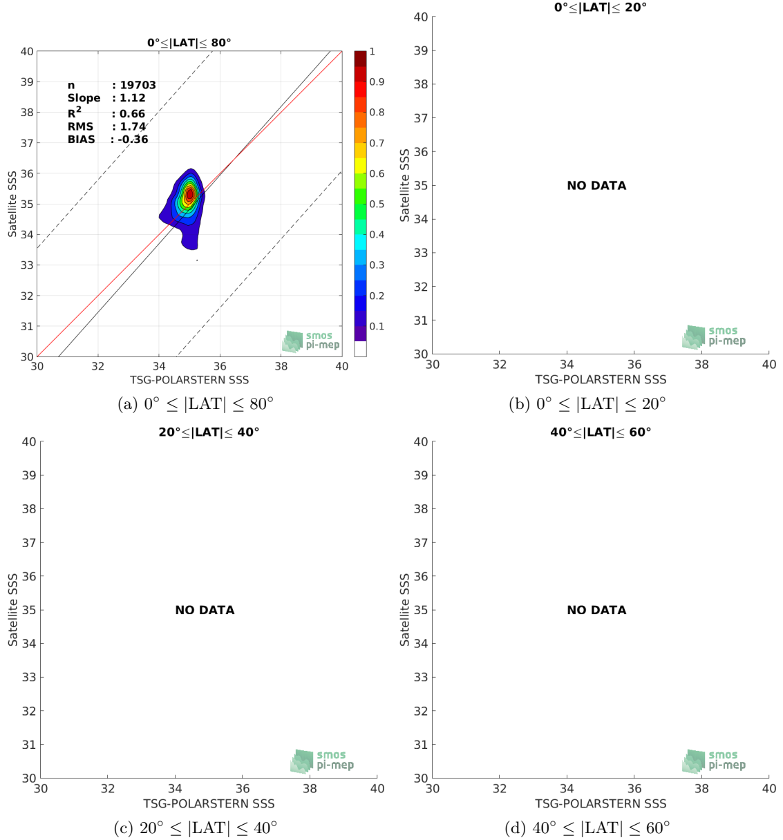
Figure 9: Contour maps of the concentration of SMOS-L3-CATDS-CECOS-LOCEAN-V4-18DAYS-25KM SSS (y-axis) versus TSG-POLARSTERN SSS (x-axis) at match-up pairs for different latitude bands. For each plot, the red line shows x=y . The black thin and dashed lines indicate a linear fit through the data cloud and the \pm 95\% confidence levels, respectively. The number match-up pairs n , the slope and R^2 coefficient of the linear fit, the root mean square (RMS) and the mean bias between satellite and in situ data are indicated for each latitude band in each plots.
