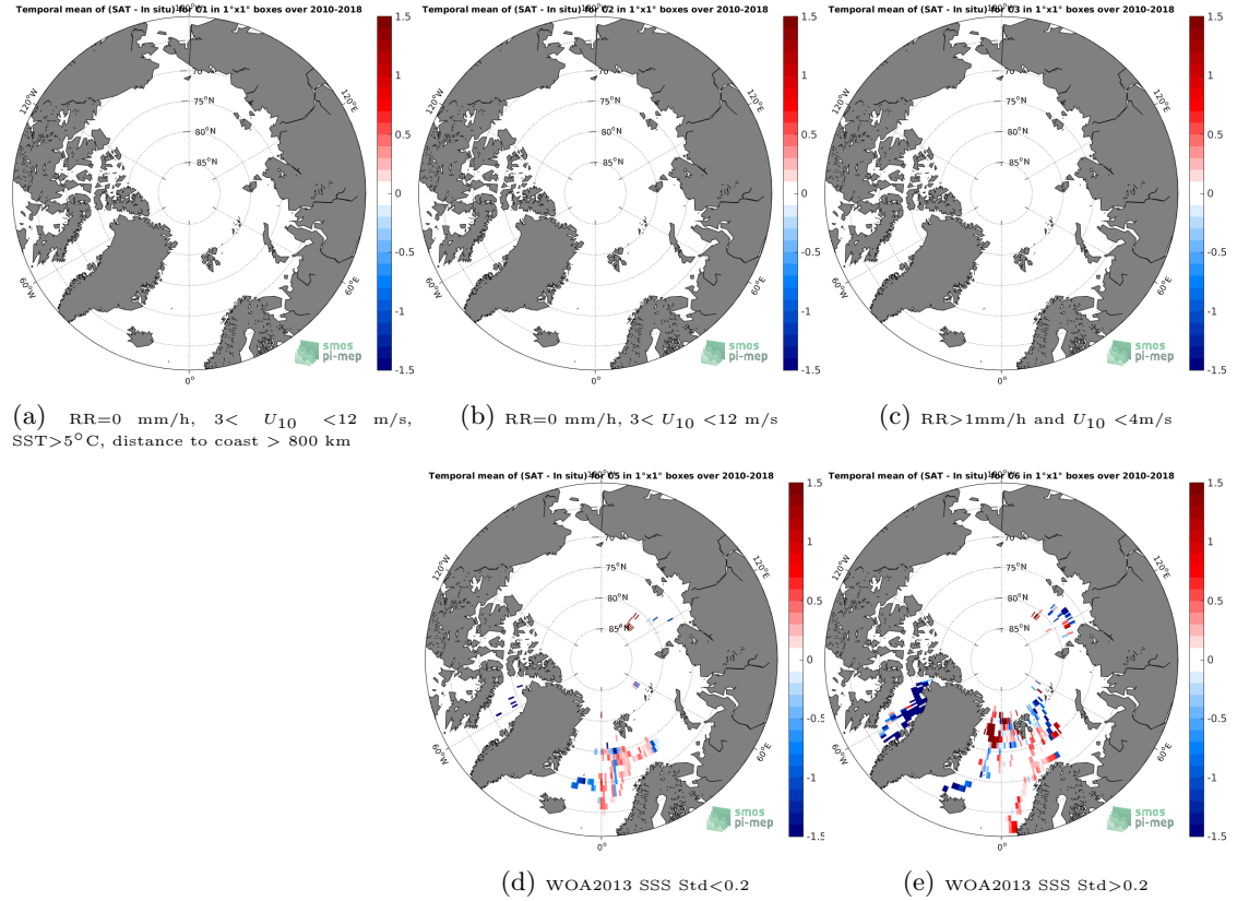
Figure 12: Temporal mean gridded over spatial boxes of size 1^{\circ}\times 1^{\circ} of \Delta\text{SSS} (SMOS-L3-CATDS-CECOS-LOCEAN-V4-18DAYS-25KM - TSG-POLARSTERN) for 5 different subdatasets corresponding to: RR=0 mm/h, 3 < U_{10} < 12 m/s, SST > 5^{\circ}\text{C} , distance to coast > 800 km (a), RR=0 mm/h, 3 < U_{10} < 12 m/s (b), RR > 1 mm/h and U_{10} < 4 m/s (c), WOA2013 SSS Std < 0.2 (d), WOA2013 SSS Std > 0.2 (e).
