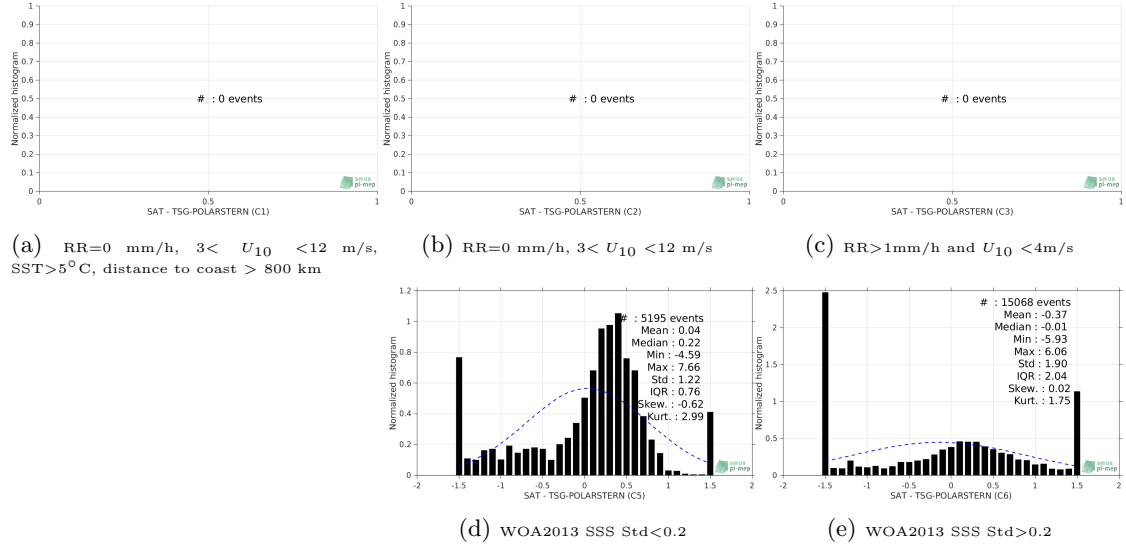
Figure 13: Normalized histogram of \Delta\text{SSS} (SMOS-L3-CATDS-CECOS-LOCEAN-V4-18DAYS-25KM - TSG-POLARSTERN) for 5 different subdatasets corresponding to: RR=0 mm/h, 3 < U_{10} < 12 m/s, SST > 5^{\circ}\text{C} , distance to coast > 800 km (a), RR=0 mm/h, 3 < U_{10} < 12 m/s (b), RR > 1\text{mm/h} and U_{10} < 4\text{m/s} (c), WOA2013 SSS Std < 0.2 (d), WOA2013 SSS Std > 0.2 (e).
