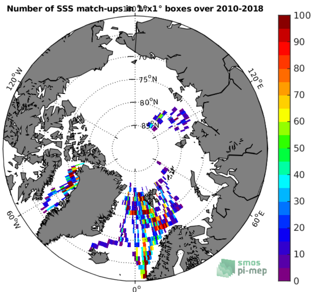
Figure 4: Number of SSS match-ups between TSG-POLARSTERN SSS and the SMOS-L3-CATDS-CECOS-LOCEAN-V4-18DAYS-25KM SSS product for the Arctic Ocean Pi-MEP region over 1°x1° boxes and for the full satellite product period.
