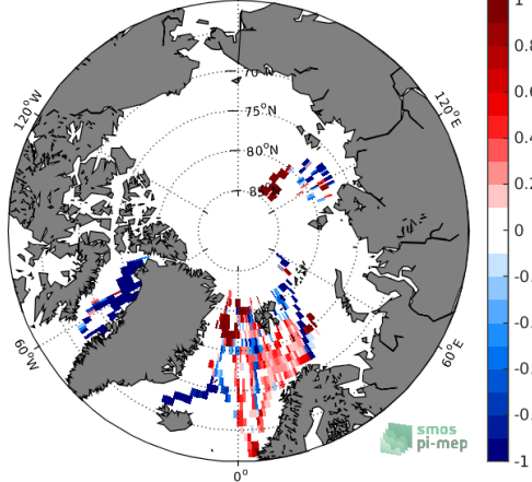
(e) MEAN( \Delta SSS) (Satellite - TSG-POLARSTERN)
