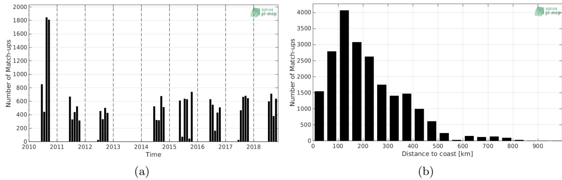
Figure 1: Number of match-ups between TSG-POLARSTERN and SMOS-L3-CATDS-CECOS-LOCEAN-V4-18DAYS-25KM SSS as a function of time (a) and as function of the distance to coast (b) over the Arctic Ocean Pi-MEP region and for the full satellite product period.
