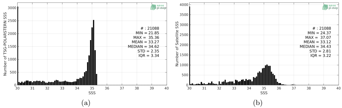
Figure 2: Histograms of SSS from TSG-POLARSTERN (a) and SMOS-L3-CATDS-CECOS-LOCEAN-V4-18DAYS-25KM (b) considering all match-up pairs per bins of 0.1 over the Arctic Ocean Pi-MEP region and for the full satellite product period.
