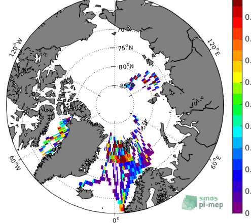
(f) Std( \Delta SSS) (Satellite - TSG-POLARSTERN)
