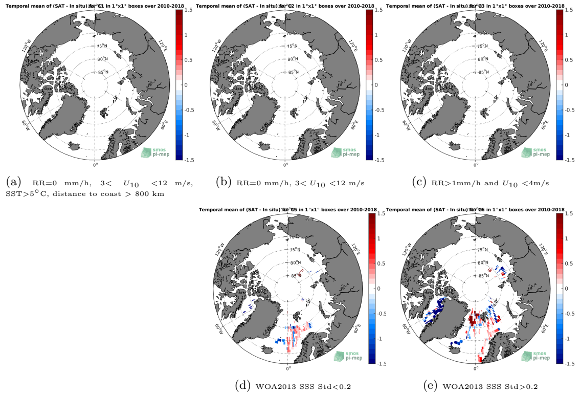
Figure 12: Temporal mean gridded over spatial boxes of size 1^\circ \times 1^\circ of \Delta SSS (SMOS-L3-CATDS-CECOS-LOCEAN-V4-18DAYS-25KM - TSG-POLARSTERN) for 5 different subdatasets corresponding to:RR=0 mm/h, 3 < U_{10} < 12 m/s, SST >5^\circ\text{C} , distance to coast > 800 km (a), RR=0 mm/h, 3 < U_{10} < 12 m/s (b), RR >1 mm/h and U_{10} < 4 m/s (c), WOA2013 SSS Std <0.2 (d), WOA2013 SSS Std >0.2 (e).
