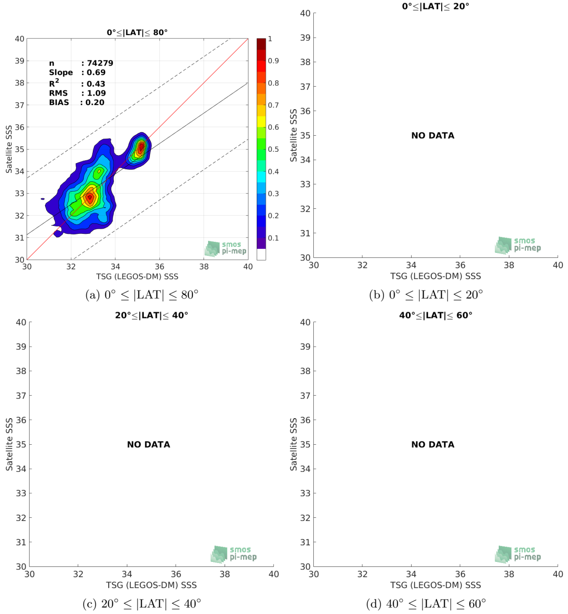
Figure 9: Contour maps of the concentration of SMOS SSS L3 v4 - 18 Days (CATDS-CECOS-LOCEAN) SSS (y-axis) versus TSG (LEGOS-DM) SSS (x-axis) at match-up pairs for different latitude bands. For each plot, the red line shows x=y . The black thin and dashed lines indicate a linear fit through the data cloud and the \pm 95\% confidence levels, respectively. The number match-up pairs n , the slope and R^2 coefficient of the linear fit, the root mean square (RMS) and the mean bias between satellite and in situ data are indicated for each latitude band in each plots.
