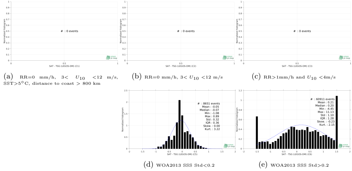
Figure 13: Normalized histogram of \Delta\text{SSS} (SMOS SSS L3 v4 - 18 Days (CATDS-CECOS-LOCEAN) - TSG (LEGOS-DM)) for 5 different subdatasets corresponding to: RR=0 mm/h, 3 < U_{10} < 12 m/s, SST > 5^{\circ}\text{C} , distance to coast > 800 km (a), RR=0 mm/h, 3 < U_{10} < 12 m/s (b), RR > 1\text{mm/h} and U_{10} < 4\text{m/s} (c), WOA2013 SSS Std<0.2 (d), WOA2013 SSS Std>0.2 (e).
