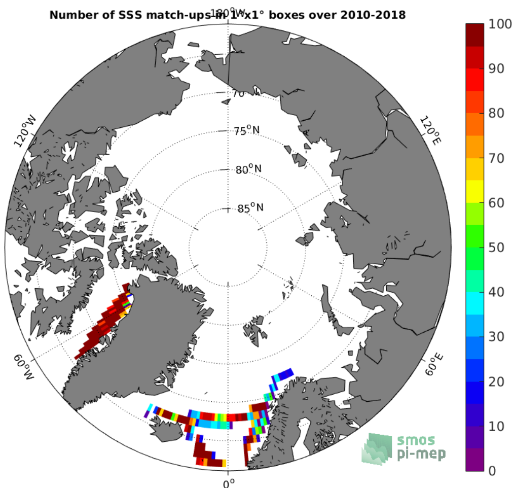
Figure 4: Number of SSS match-ups between TSG-LEGOS-DM SSS and the SMOS-L3-CATDS-CECOS-LOCEAN-V4-18DAYS-25KM SSS product for the Arctic Ocean Pi-MEP region over 1^\circ \times 1^\circ boxes and for the full satellite product period.
