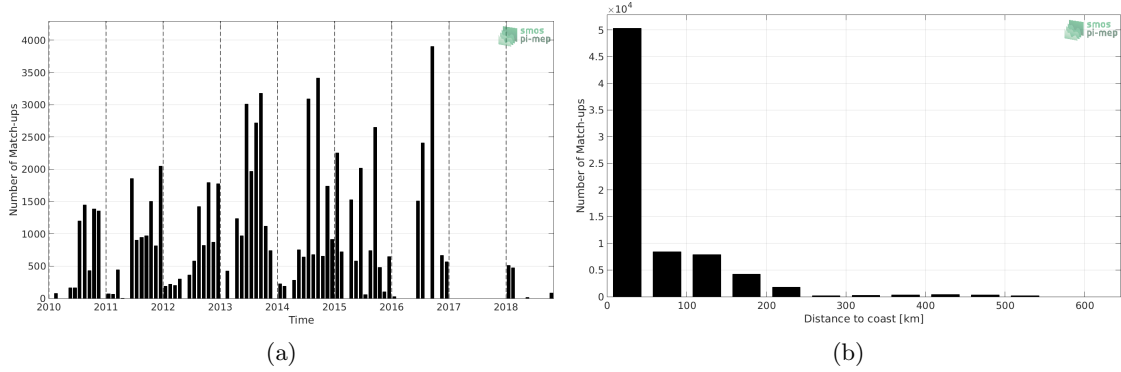
Figure 1: Number of match-ups between TSG-LEGOS-DM and SMOS-L3-CATDS-CECOS-LOCEAN-V4-18DAYS-25KM SSS as a function of time (a) and as function of the distance to coast (b) over the Arctic Ocean Pi-MEP region and for the full satellite product period.
