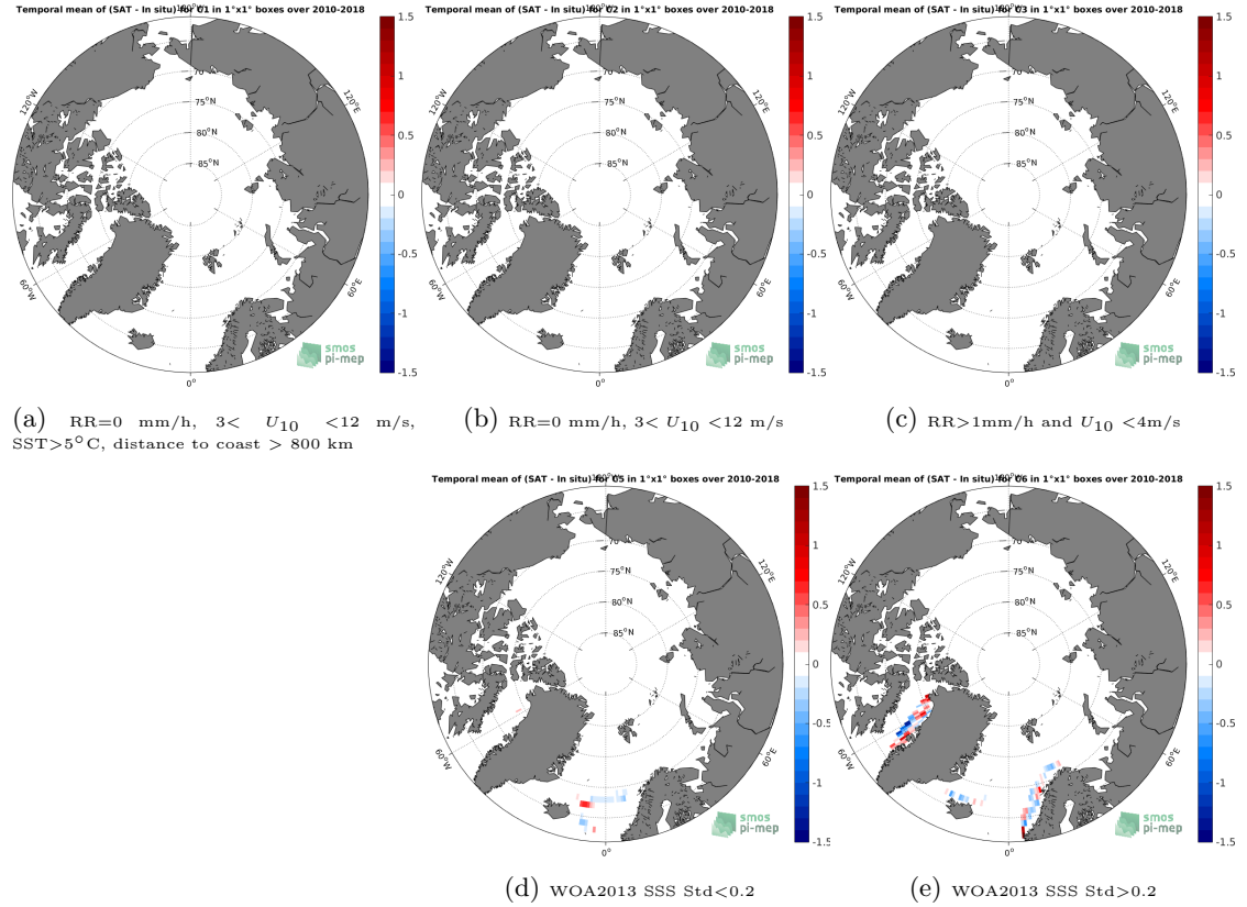
Figure 12: Temporal mean gridded over spatial boxes of size 1^{\circ}\times 1^{\circ} of \Delta\text{SSS} (SMOS-L3-CATDS-CECOS-LOCEAN-V4-18DAYS-25KM - TSG-LEGOS-DM) for 5 different subdatasets corresponding to: \text{RR}=0 mm/h, 3 < U_{10} < 12 m/s, \text{SST} > 5^{\circ}\text{C} , distance to coast > 800 km (a), \text{RR}=0 mm/h, 3 < U_{10} < 12 m/s (b), \text{RR} > 1 mm/h and U_{10} < 4 m/s (c), WOA2013 SSS Std < 0.2 (d), WOA2013 SSS Std > 0.2 (e).
