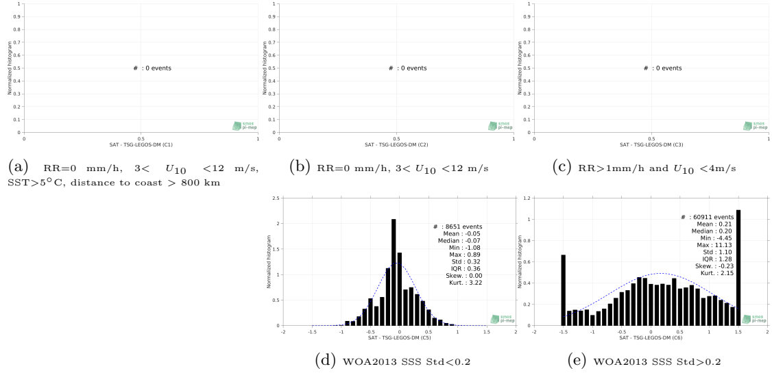
Figure 13: Normalized histogram of \Delta\text{SSS} (SMOS-L3-CATDS-CECOS-LOCEAN-V4-18DAYS-25KM - TSG-LEGOS-DM) for 5 different subdatasets corresponding to: RR=0 mm/h, 3 < U_{10} < 12 m/s, SST >5^{\circ}\text{C} , distance to coast > 800 km (a), RR=0 mm/h, 3 < U_{10} < 12 m/s (b), RR>1\text{mm/h} and U_{10} < 4\text{m/s} (c), WOA2013 SSS Std <0.2 (d), WOA2013 SSS Std >0.2 (e).
