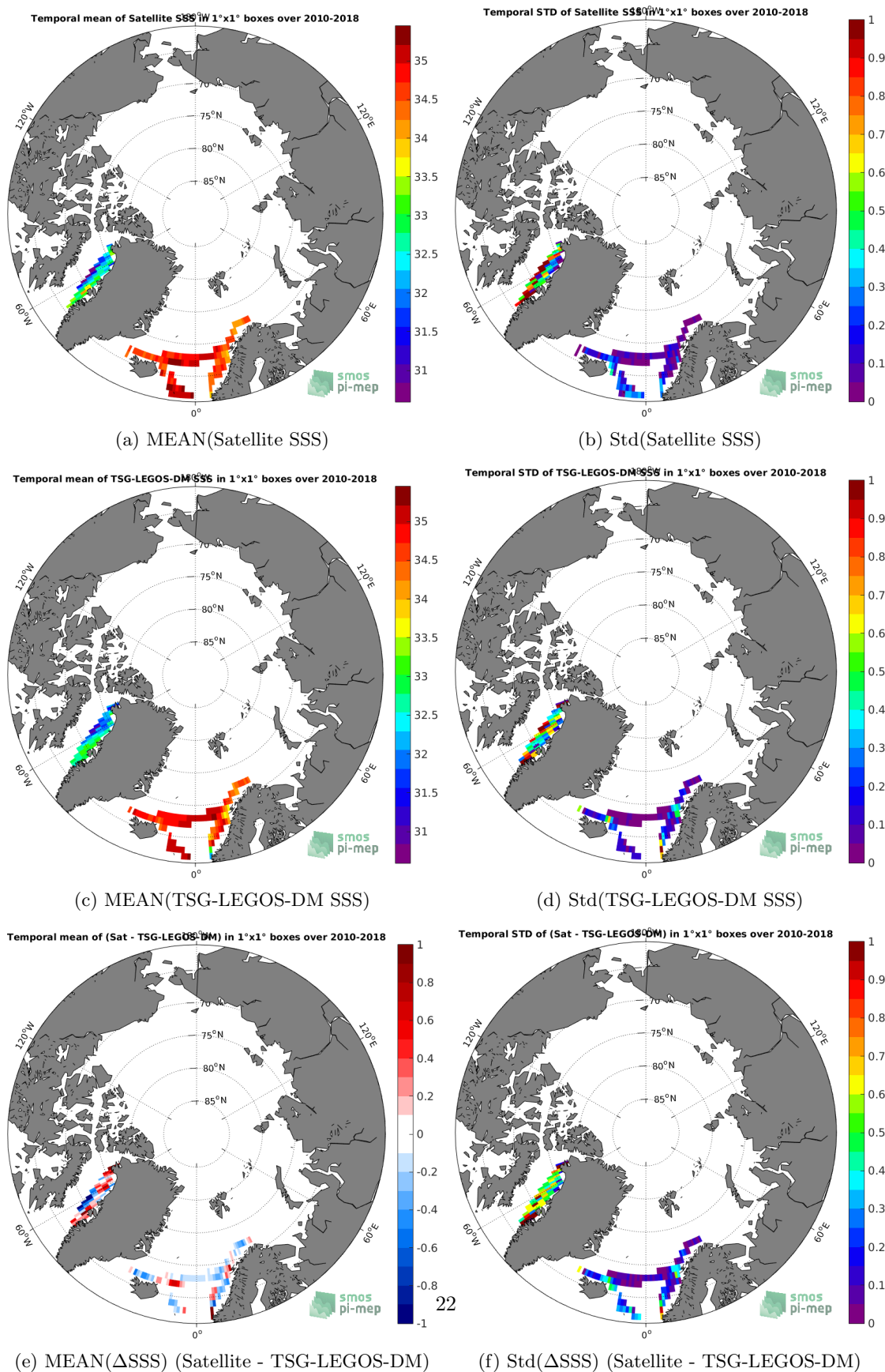
Figure 6: Temporal mean (left) and Std (right) of SSS from SMOS-L3-CATDS-CECOS-LOCEAN-V4-18DAYS-25KM (top), TSG-LEGOS-DM (middle), and of \Delta SSS (Satellite - TSG-LEGOS-DM). Only match-up pairs are used to generate these maps.
