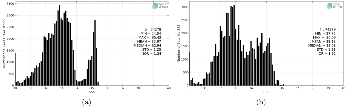
Figure 2: Histograms of SSS from TSG-LEGOS-DM (a) and SMOS-L3-CATDS-CECOS-LOCEAN-V4-18DAYS-25KM (b) considering all match-up pairs per bins of 0.1 over the Arctic Ocean Pi-MEP region and for the full satellite product period.
