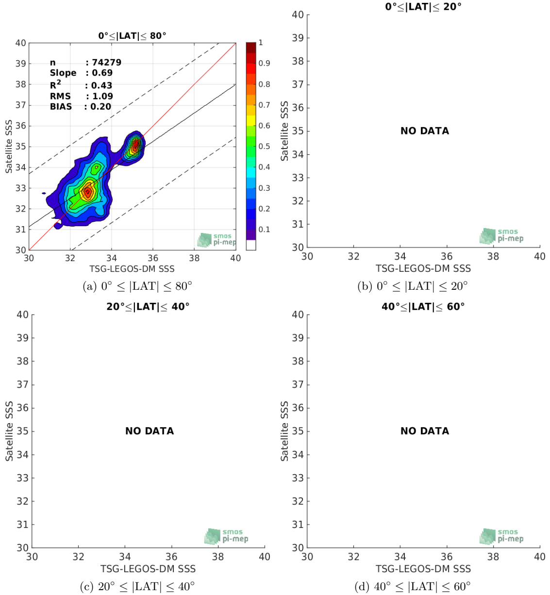
Figure 9: Contour maps of the concentration of SMOS-L3-CATDS-CECOS-LOCEAN-V4-18DAYS-25KM SSS (y-axis) versus TSG-LEGOS-DM SSS (x-axis) at match-up pairs for different latitude bands. For each plot, the red line shows x=y . The black thin and dashed lines indicate a linear fit through the data cloud and the \pm 95\% confidence levels, respectively. The number match-up pairs n , the slope and R^2 coefficient of the linear fit, the root mean square (RMS) and the mean bias between satellite and in situ data are indicated for each latitude band in each plots.
