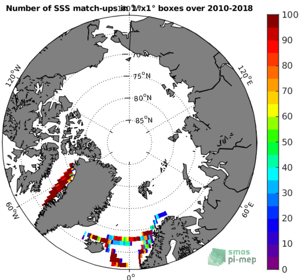
Figure 4: Number of SSS match-ups between TSG-LEGOS-DM SSS and the SMOS-L3-CATDS-CECOS-LOCEAN-V4-18DAYS-25KM SSS product for the Arctic Ocean Pi-MEP region over 1°x1° boxes and for the full satellite product period.
