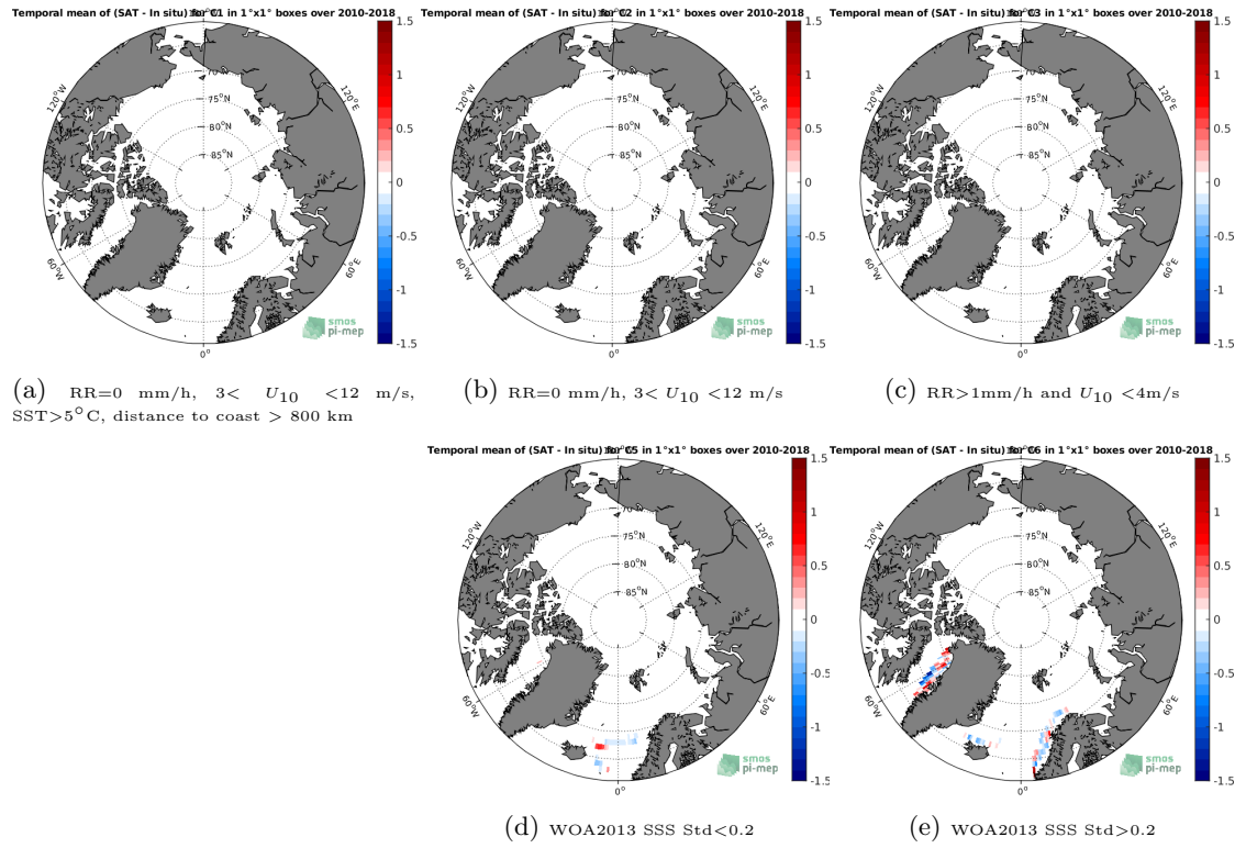
Figure 12: Temporal mean gridded over spatial boxes of size 1^\circ \times 1^\circ of \Delta SSS (SMOS-L3-CATDS-CECOS-LOCEAN-V4-18DAYS-25KM - TSG-LEGOS-DM) for 5 different subdatasets corresponding to:RR=0 mm/h, 3 < U_{10} < 12 m/s, SST >5^\circ\text{C} , distance to coast > 800 km (a), RR=0 mm/h, 3 < U_{10} < 12 m/s (b), RR >1 mm/h and U_{10} < 4 m/s (c), WOA2013 SSS Std <0.2 (d), WOA2013 SSS Std >0.2 (e).
