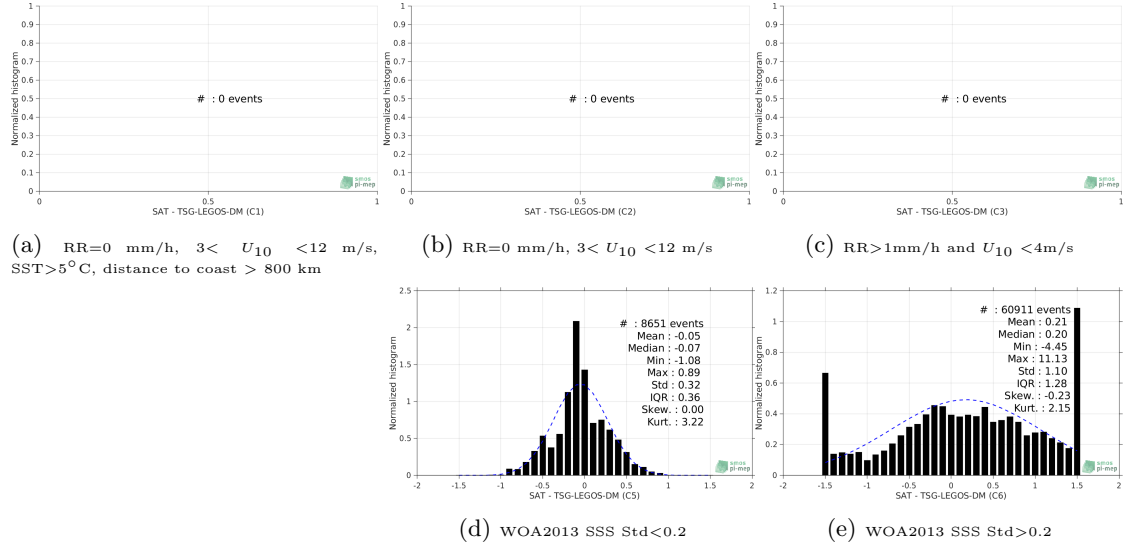
Figure 13: Normalized histogram of \Delta\text{SSS} (SMOS-L3-CATDS-CECOS-LOCEAN-V4-18DAYS-25KM - TSG-LEGOS-DM) for 5 different subdatasets corresponding to: RR=0 mm/h, 3 < U_{10} < 12 m/s, SST >5^{\circ}\text{C} , distance to coast > 800 km (a), RR=0 mm/h, 3 < U_{10} < 12 m/s (b), RR>1\text{mm/h} and U_{10} < 4\text{m/s} (c), WOA2013 SSS Std <0.2 (d), WOA2013 SSS Std >0.2 (e).
