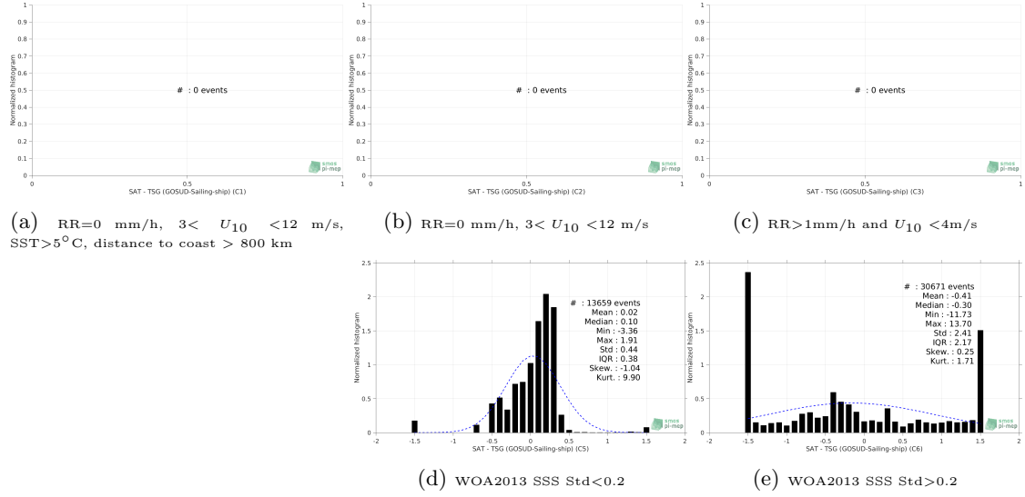
Figure 13: Normalized histogram of \Delta\text{SSS} (SMOS SSS L3 v4 - 18 Days (CATDS-CECOS-LOCEAN) - TSG (GOSUD-Sailing-ship)) for 5 different subdatasets corresponding to: RR=0 mm/h, 3 < U_{10} < 12 m/s, SST > 5^\circ\text{C} , distance to coast > 800 km (a), RR=0 mm/h, 3 < U_{10} < 12 m/s (b), RR > 1\text{mm/h} and U_{10} < 4\text{m/s} (c), WOA2013 SSS Std<0.2 (d), WOA2013 SSS Std>0.2 (e).
