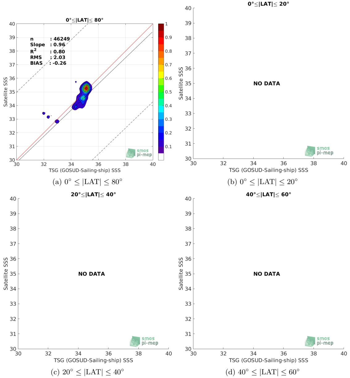
Figure 9: Contour maps of the concentration of SMOS SSS L3 v4 - 18 Days (CATDS-CECOS-LOCEAN) SSS (y-axis) versus TSG (GOSUD-Sailing-ship) SSS (x-axis) at match-up pairs for different latitude bands. For each plot, the red line shows x=y . The black thin and dashed lines indicate a linear fit through the data cloud and the \pm 95\% confidence levels, respectively. The number match-up pairs n , the slope and R^2 coefficient of the linear fit, the root mean square (RMS) and the mean bias between satellite and in situ data are indicated for each latitude band in each plots.
