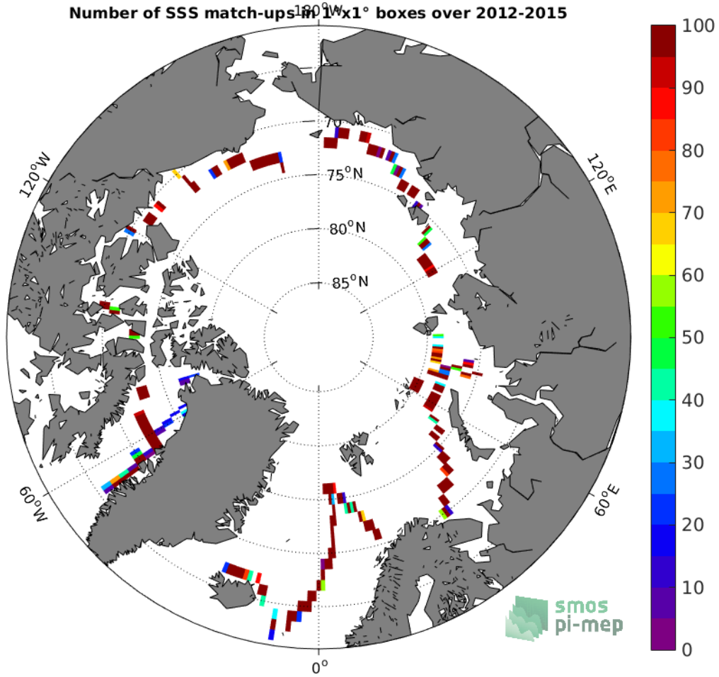
Figure 4: Number of SSS match-ups between TSG (GOSUD-Sailing-ship) SSS and the SMOS SSS L3 v4 - 18 Days (CATDS-CECOS-LOCEAN) SSS product for the Arctic Ocean Pi-MEP region over 1°x1° boxes and for the full satellite product period.
