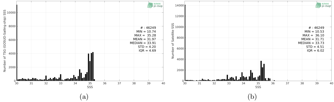
Figure 2: Histograms of SSS from TSG (GOSUD-Sailing-ship) (a) and SMOS SSS L3 v4 - 18 Days (CATDS-CECOS-LOCEAN) (b) considering all match-up pairs per bins of 0.1 over the Arctic Ocean Pi-MEP region and for the full satellite product period.
