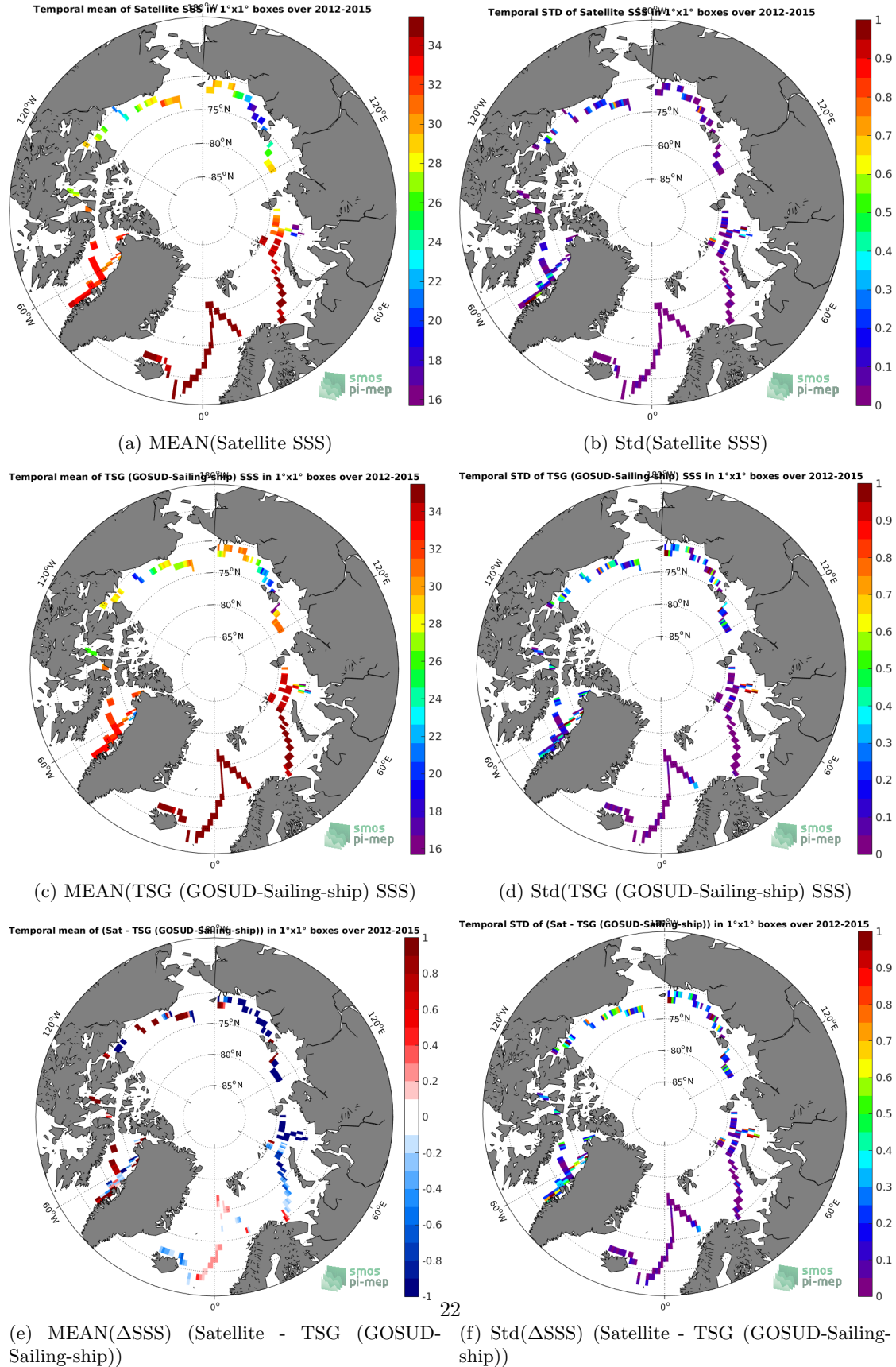
Figure 6: Temporal mean (left) and Std (right) of SSS from SMOS SSS L3 v4 - 18 Days (CATDS-CECOS-LOCEAN) (top), TSG (GOSUD-Sailing-ship) (middle), and of \Delta SSS (Satellite - TSG (GOSUD-Sailing-ship)). Only match-up pairs are used to generate these maps.
