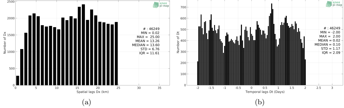
Figure 5: Histograms of the spatial (a) and temporal (b) lags between the time of the TSG (GOSUD-Sailing-ship) measurements and the date of the corresponding SMOS SSS L3 v4 - 18 Days (CATDS-CECOS-LOCEAN) SSS product.
