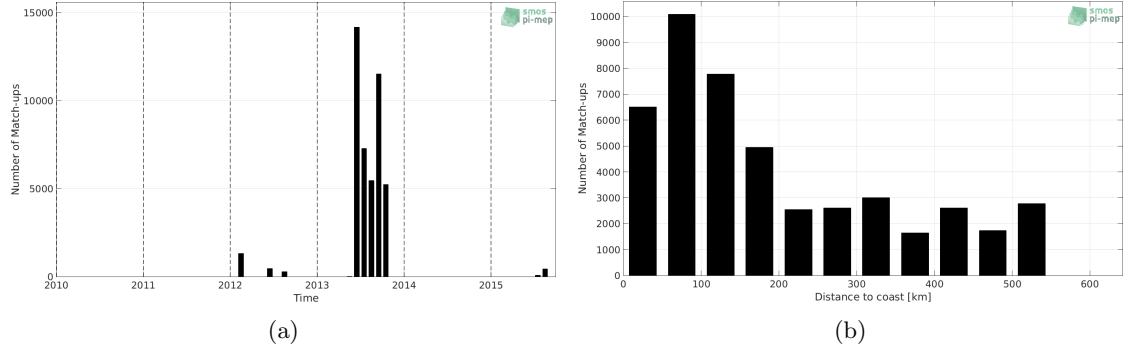
Figure 1: Number of match-ups between TSG (GOSUD-Sailing-ship) and SMOS SSS L3 v4 - 18 Days (CATDS-CECOS-LOCEAN) SSS as a function of time (a) and as function of the distance to coast (b) over the Arctic Ocean Pi-MEP region and for the full satellite product period.
