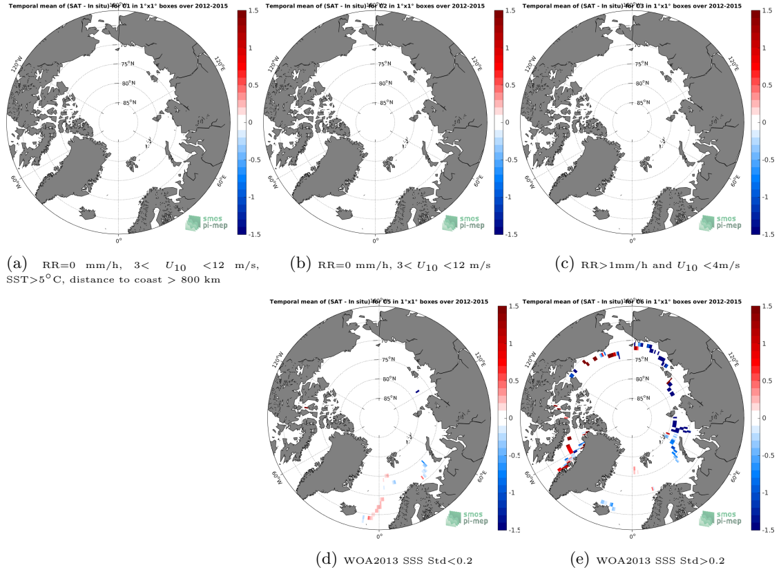
Figure 12: Temporal mean gridded over spatial boxes of size 1^{\circ} \times 1^{\circ} of \Delta\text{SSS} (SMOS SSS L3 v4 - 18 Days (CATDS-CECOS-LOCEAN) - TSG (GOSUD-Sailing-ship)) for 5 different subdatasets corresponding to: RR=0 mm/h, 3 < U_{10} < 12 m/s, SST > 5^{\circ}\text{C} , distance to coast > 800 km (a), RR=0 mm/h, 3 < U_{10} < 12 m/s (b), RR > 1\text{mm/h} and U_{10} < 4\text{m/s} (c), WOA2013 SSS Std < 0.2 (d), WOA2013 SSS Std > 0.2 (e).
