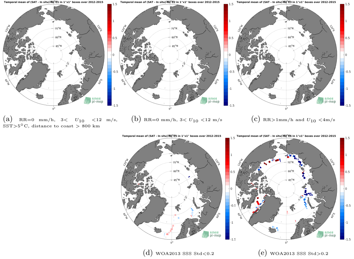
Figure 12: Temporal mean gridded over spatial boxes of size 1°x1° of \Delta SSS (SMOS-L3-CATDS-CECOS-LOCEAN-V4-18DAYS-25KM - TSG-GOSUD-Sailing-ship) for 5 different subdatasets corresponding to:RR=0 mm/h, 3 < U_{10} < 12 m/s, SST>5°C, distance to coast > 800 km (a), RR=0 mm/h, 3 < U_{10} < 12 m/s (b), RR>1mm/h and U_{10} < 4 m/s (c), WOA2013 SSS Std<0.2 (d), WOA2013 SSS Std>0.2 (e).
