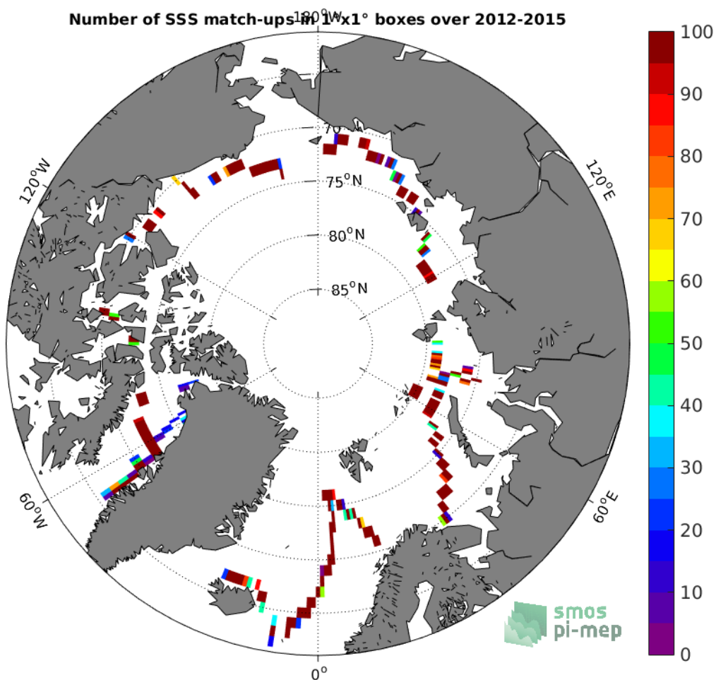
Figure 4: Number of SSS match-ups between TSG-GOSUD-Sailing-ship SSS and the SMOS-L3-CATDS-CECOS-LOCEAN-V4-18DAYS-25KM SSS product for the Arctic Ocean Pi-MEP region over 1^\circ \times 1^\circ boxes and for the full satellite product period.
