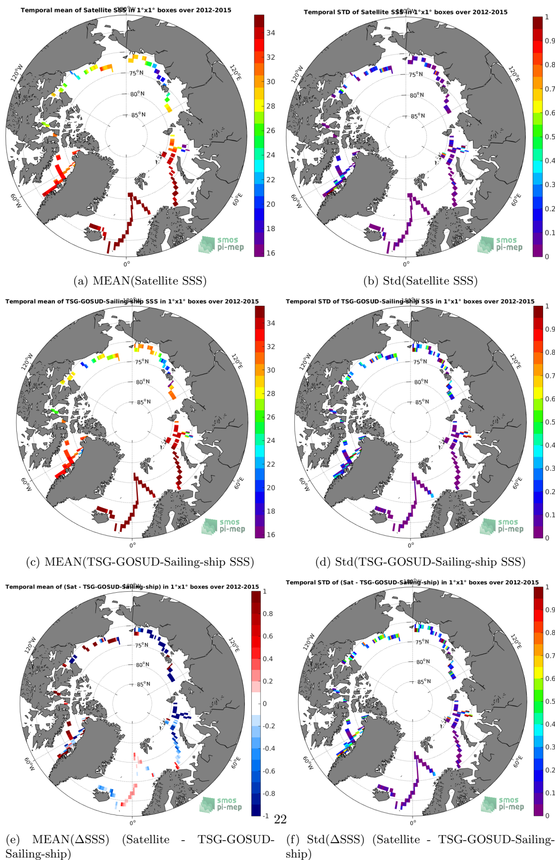
Figure 6: Temporal mean (left) and Std (right) of SSS from SMOS-L3-CATDS-CECOS-LOCEAN-V4-18DAYS-25KM (top), TSG-GOSUD-Sailing-ship (middle), and of \Delta SSS (Satellite - TSG-GOSUD-Sailing-ship). Only match-up pairs are used to generate these maps.
