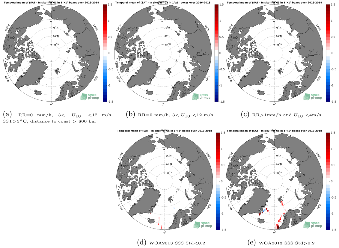
Figure 12: Temporal mean gridded over spatial boxes of size 1°x1° of \Delta SSS (SMOS SSS L3 v4 - 18 Days (CATDS-CECOS-LOCEAN) - TSG (GOSUD-Research-vessel)) for 5 different subdatasets corresponding to: RR=0 mm/h, 3 < U_{10} < 12 m/s, SST>5°C, distance to coast > 800 km (a), RR=0 mm/h, 3 < U_{10} < 12 m/s (b), RR>1mm/h and U_{10} < 4 m/s (c), WOA2013 SSS Std<0.2 (d), WOA2013 SSS Std>0.2 (e).
