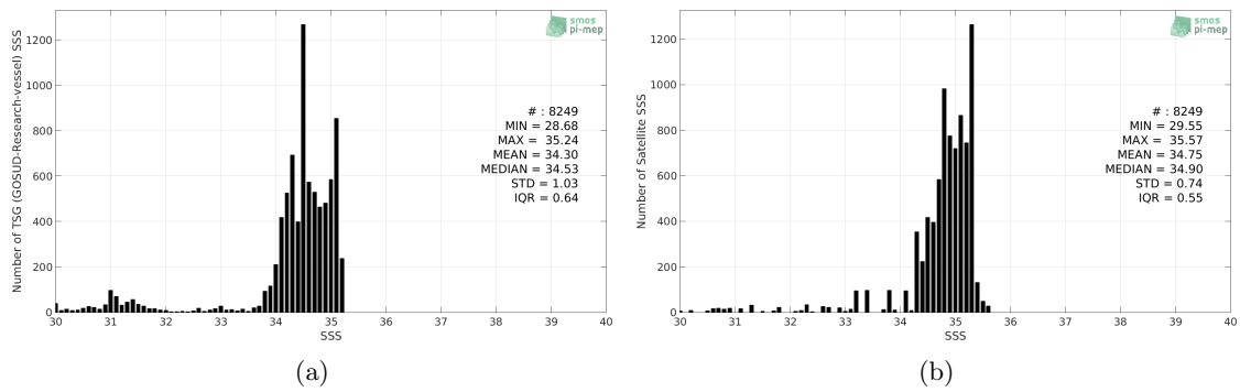
Figure 2: Histograms of SSS from TSG (GOSUD-Research-vessel) (a) and SMOS SSS L3 v4 - 18 Days (CATDS-CECOS-LOCEAN) (b) considering all match-up pairs per bins of 0.1 over the Arctic Ocean Pi-MEP region and for the full satellite product period.
