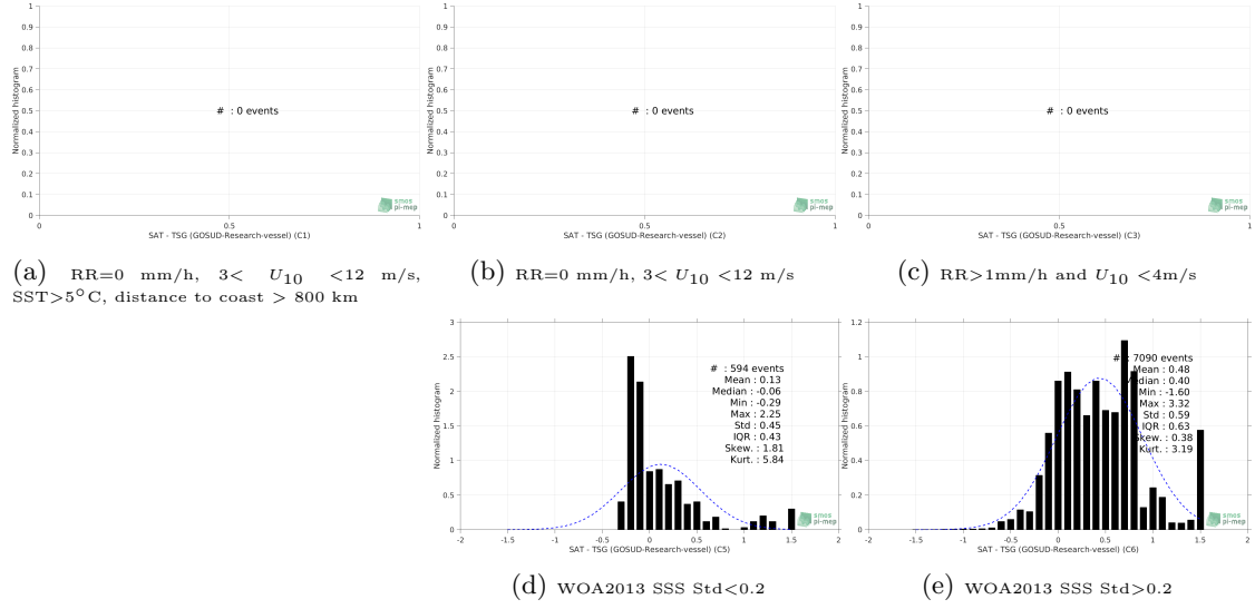
Figure 13: Normalized histogram of \Delta\text{SSS} (SMOS SSS L3 v4 - 18 Days (CATDS-CECOS-LOCEAN) - TSG (GOSUD-Research-vessel)) for 5 different subdatasets corresponding to: RR=0 mm/h, 3 < U_{10} < 12 m/s, SST > 5^\circ\text{C} , distance to coast > 800 km (a), RR=0 mm/h, 3 < U_{10} < 12 m/s (b), RR > 1 mm/h and U_{10} < 4 m/s (c), WOA2013 SSS Std < 0.2 (d), WOA2013 SSS Std > 0.2 (e).
