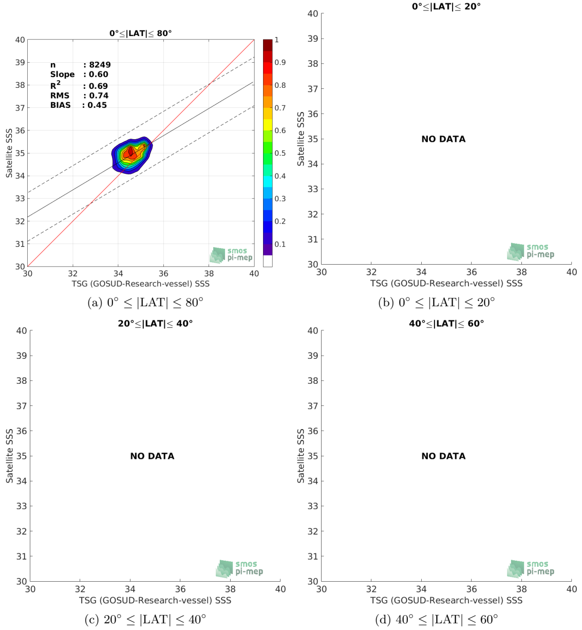
Figure 9: Contour maps of the concentration of SMOS SSS L3 v4 - 18 Days (CATDS-CECOS-LOCEAN) SSS (y-axis) versus TSG (GOSUD-Research-vessel) SSS (x-axis) at match-up pairs for different latitude bands. For each plot, the red line shows x=y . The black thin and dashed lines indicate a linear fit through the data cloud and the \pm 95\% confidence levels, respectively. The number match-up pairs n , the slope and R^2 coefficient of the linear fit, the root mean square (RMS) and the mean bias between satellite and in situ data are indicated for each latitude band in each plots.
