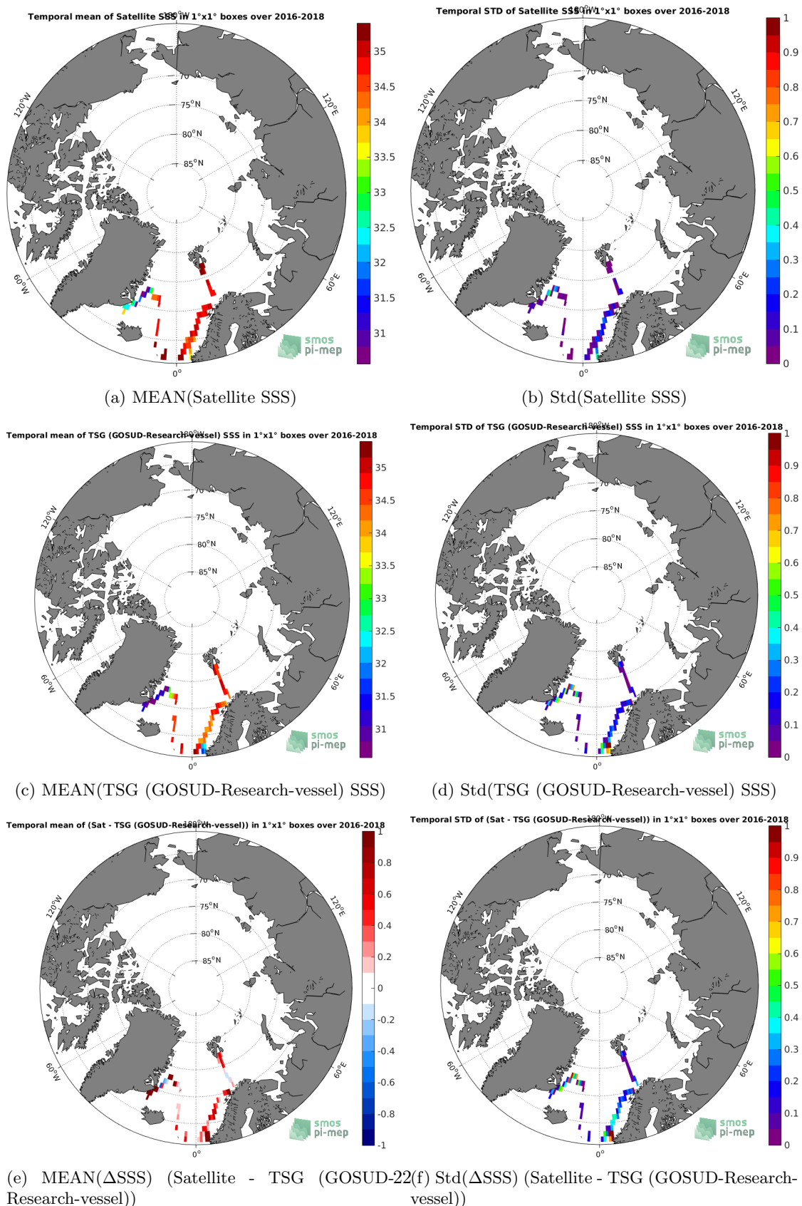
Figure 6: Temporal mean (left) and Std (right) of SSS from SMOS SSS L3 v4 - 18 Days (CATDS-CECOS-LOCEAN) (top), TSG (GOSUD-Research-vessel) (middle), and of \Delta SSS (Satellite - TSG (GOSUD-Research-vessel)). Only match-up pairs are used to generate these maps.
