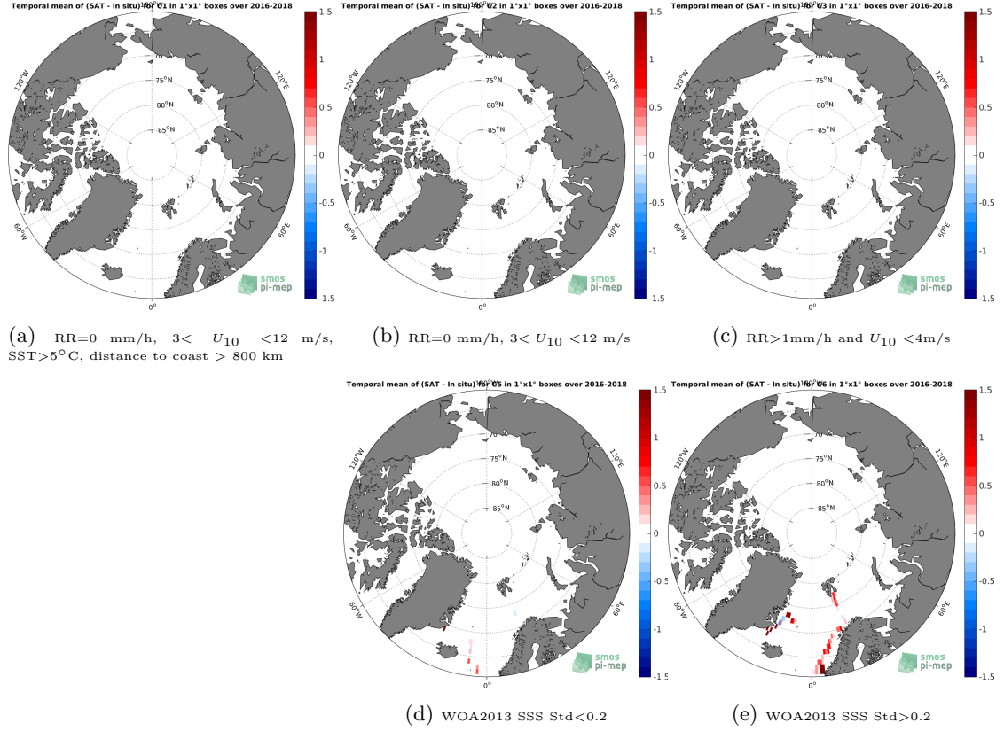
Figure 12: Temporal mean gridded over spatial boxes of size 1^\circ \times 1^\circ of \Delta SSS (SMOS-L3-CATDS-CECOS-LOCEAN-V4-18DAYS-25KM - TSG-GOSUD-Research-vessel) for 5 different subdatasets corresponding to: RR=0 mm/h, 3 < U_{10} < 12 m/s, SST > 5^\circ\text{C} , distance to coast > 800 km (a), RR=0 mm/h, 3 < U_{10} < 12 m/s (b), RR > 1 mm/h and U_{10} < 4 m/s (c), WOA2013 SSS Std < 0.2 (d), WOA2013 SSS Std > 0.2 (e).
