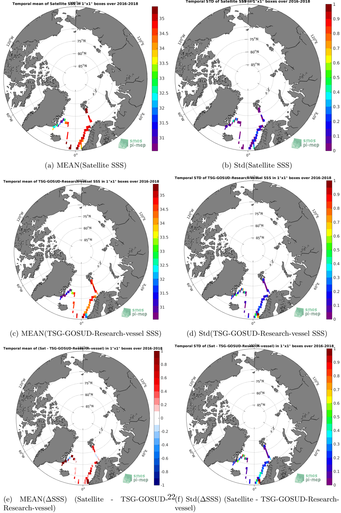
Figure 6: Temporal mean (left) and Std (right) of SSS from SMOS-L3-CATDS-CECOS-LOCEAN-V4-18DAYS-25KM (top), TSG-GOSUD-Research-vessel (middle), and of \Delta SSS (Satellite - TSG-GOSUD-Research-vessel). Only match-up pairs are used to generate these maps.
