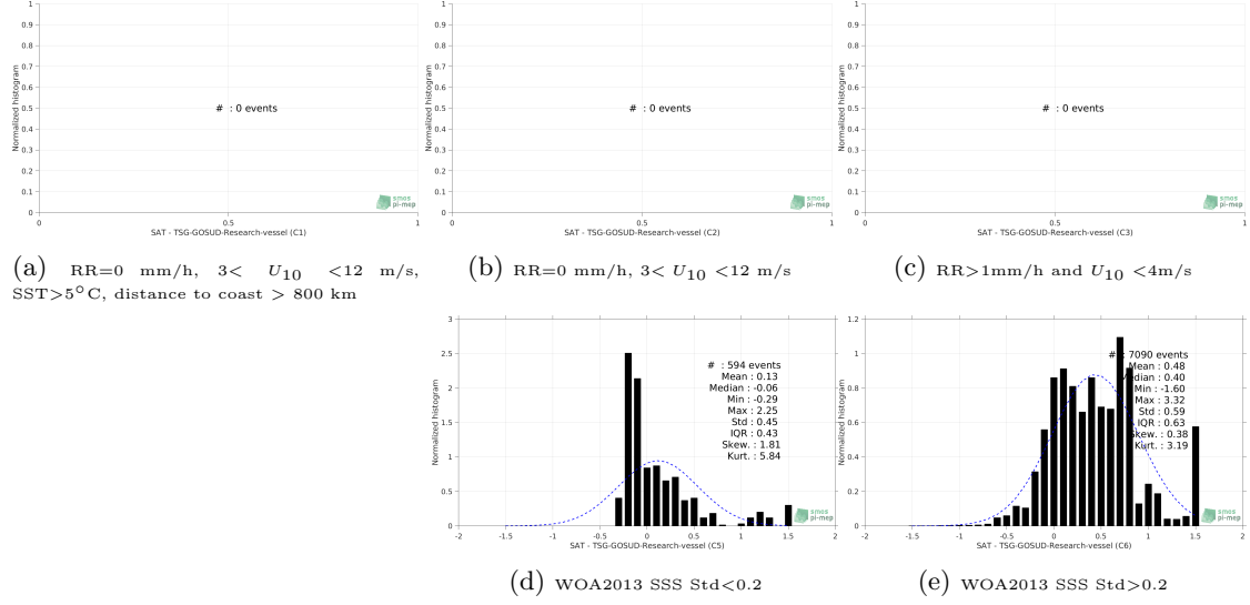
Figure 13: Normalized histogram of \Delta\text{SSS} (SMOS-L3-CATDS-CECOS-LOCEAN-V4-18DAYS-25KM - TSG-GOSUD-Research-vessel) for 5 different subdatasets corresponding to: RR=0 mm/h, 3 < U_{10} < 12 m/s, SST > 5^\circ\text{C} , distance to coast > 800 km (a), RR=0 mm/h, 3 < U_{10} < 12 m/s (b), RR > 1\text{mm/h} and U_{10} < 4\text{m/s} (c), WOA2013 SSS Std<0.2 (d), WOA2013 SSS Std>0.2 (e).
