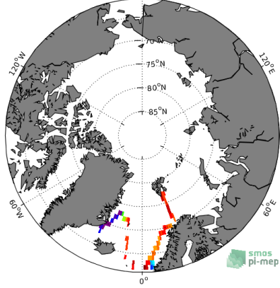
(c) MEAN(TSG-GOSUD-Research-vessel SSS)
