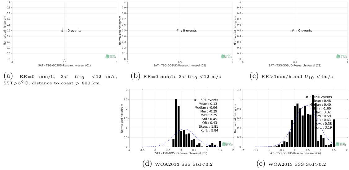
Figure 13: Normalized histogram of \Delta\text{SSS} (SMOS-L3-CATDS-CECOS-LOCEAN-V4-18DAYS-25KM - TSG-GOSUD-Research-vessel) for 5 different subdatasets corresponding to: RR=0 mm/h, 3 < U_{10} < 12 m/s, SST >5^{\circ}\text{C} , distance to coast > 800 km (a), RR=0 mm/h, 3 < U_{10} < 12 m/s (b), RR>1\text{mm/h} and U_{10} < 4\text{m/s} (c), WOA2013 SSS Std <0.2 (d), WOA2013 SSS Std >0.2 (e).
