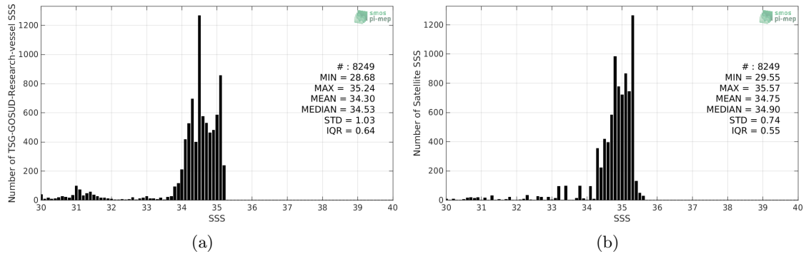
Figure 2: Histograms of SSS from TSG-GOSUD-Research-vessel (a) and SMOS-L3-CATDS-CECOS-LOCEAN-V4-18DAYS-25KM (b) considering all match-up pairs per bins of 0.1 over the Arctic Ocean Pi-MEP region and for the full satellite product period.
