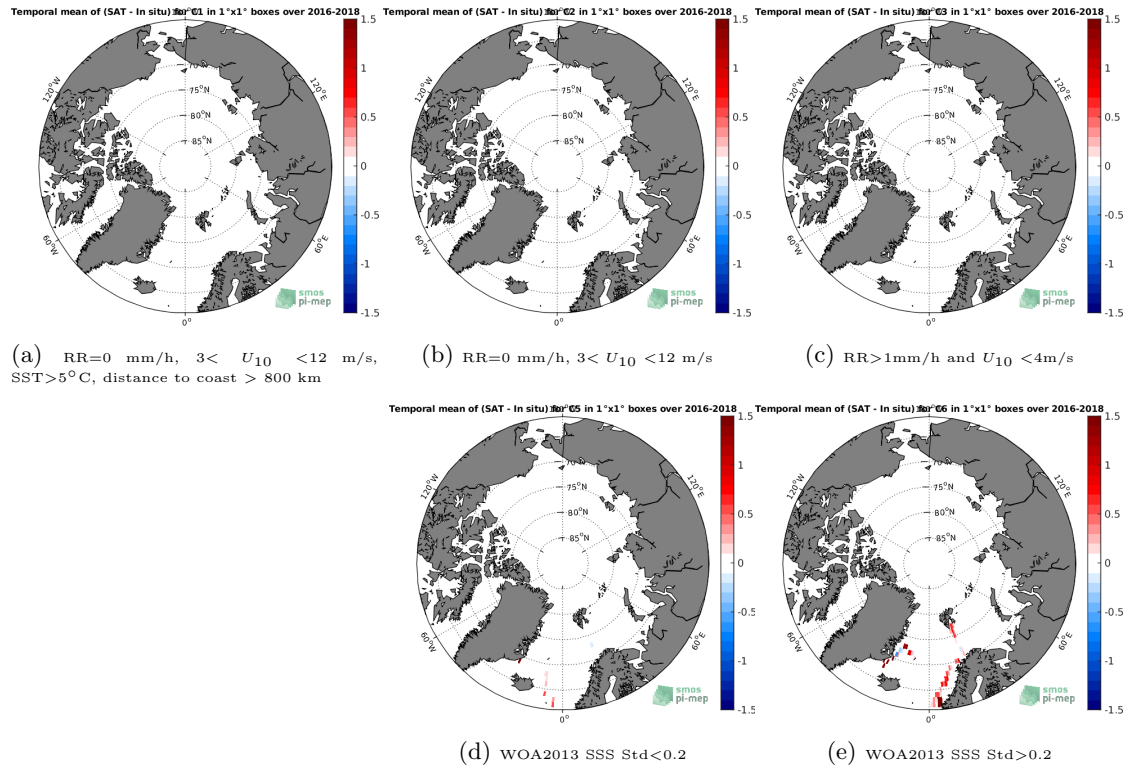
Figure 12: Temporal mean gridded over spatial boxes of size 1^\circ \times 1^\circ of \Delta SSS (SMOS-L3-CATDS-CECOS-LOCEAN-V4-18DAYS-25KM - TSG-GOSUD-Research-vessel) for 5 different subdatasets corresponding to: RR=0 mm/h, 3 < U_{10} < 12 m/s, SST > 5^\circ\text{C} , distance to coast > 800 km (a), RR=0 mm/h, 3 < U_{10} < 12 m/s (b), RR > 1 mm/h and U_{10} < 4 m/s (c), WOA2013 SSS Std < 0.2 (d), WOA2013 SSS Std > 0.2 (e).
