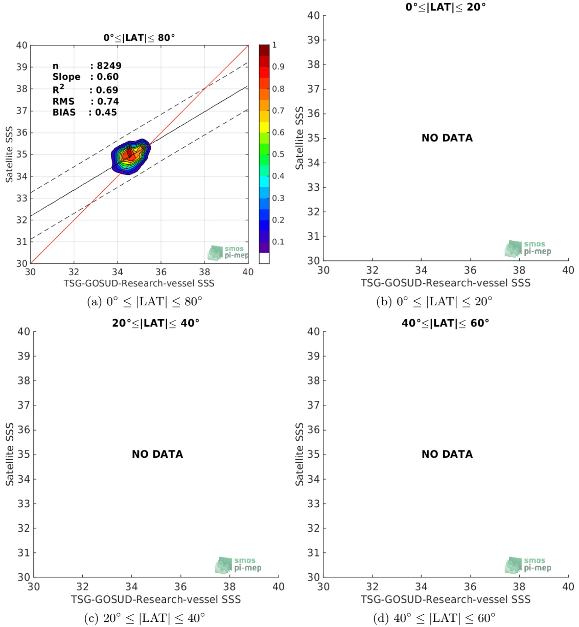
Figure 9: Contour maps of the concentration of SMOS-L3-CATDS-CECOS-LOCEAN-V4-18DAYS-25KM SSS (y-axis) versus TSG-GOSUD-Research-vessel SSS (x-axis) at match-up pairs for different latitude bands. For each plot, the red line shows x=y . The black thin and dashed lines indicate a linear fit through the data cloud and the \pm 95\% confidence levels, respectively. The number match-up pairs n , the slope and R^2 coefficient of the linear fit, the root mean square (RMS) and the mean bias between satellite and in situ data are indicated for each latitude band in each plots.
