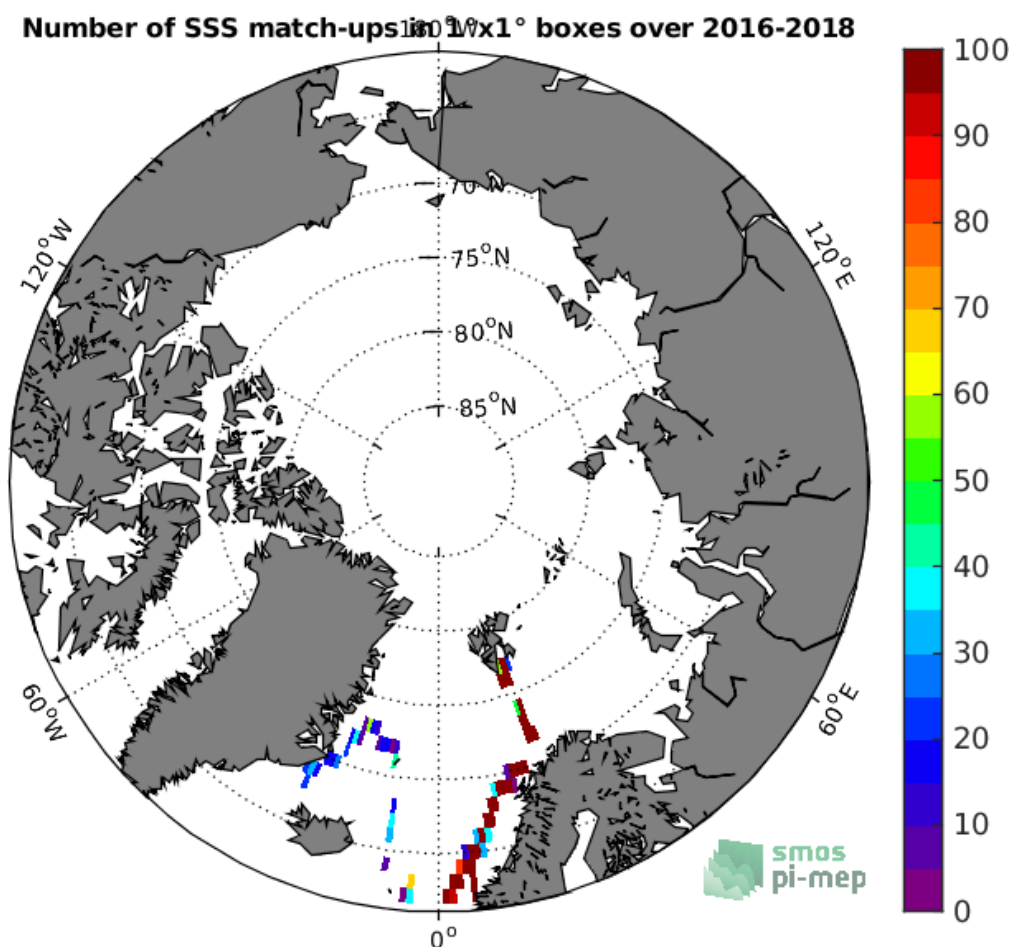
Figure 4: Number of SSS match-ups between TSG-GOSUD-Research-vessel SSS and the SMOS-L3-CATDS-CECOS-LOCEAN-V4-18DAYS-25KM SSS product for the Arctic Ocean Pi-MEP region over 1°x1° boxes and for the full satellite product period.
