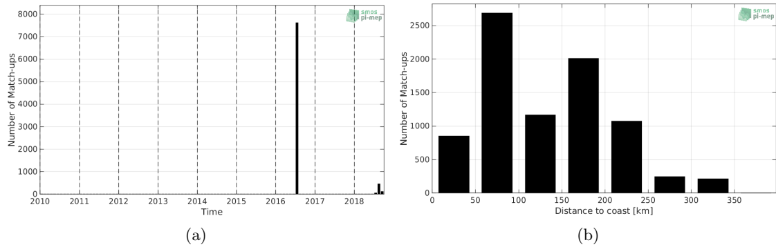
Figure 1: Number of match-ups between TSG-GOSUD-Research-vessel and SMOS-L3-CATDS-CECOS-LOCEAN-V4-18DAYS-25KM SSS as a function of time (a) and as function of the distance to coast (b) over the Arctic Ocean Pi-MEP region and for the full satellite product period.
