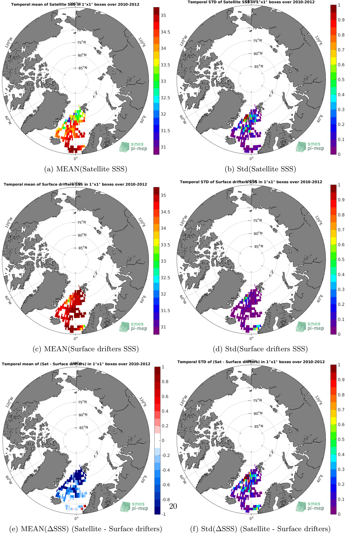
Figure 5: Temporal mean (left) and Std (right) of SSS from SMOS SSS L3 v4 - 18 Days (CATDS-CECOS-LOCEAN) (top), Surface drifters (middle), and of \Delta SSS (Satellite - Surface drifters). Only match-up pairs are used to generate these maps.
