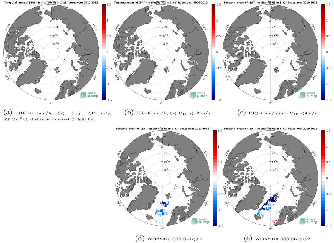
Figure 11: Temporal mean gridded over spatial boxes of size 1^{\circ}\times 1^{\circ} of \Delta\text{SSS} (SMOS SSS L3 v4 - 18 Days (CATDS-CECOS-LOCEAN) - Surface drifters) for 5 different subdatasets corresponding to: RR=0 mm/h, 3 < U_{10} < 12 m/s, SST >5^{\circ}\text{C} , distance to coast > 800 km (a), RR=0 mm/h, 3 < U_{10} < 12 m/s (b), RR >1 mm/h and U_{10} < 4 m/s (c), WOA2013 SSS Std <0.2 (d), WOA2013 SSS Std >0.2 (e).
