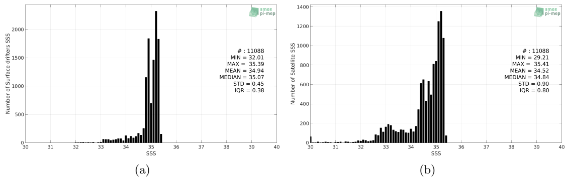
Figure 2: Histograms of SSS from Surface drifters (a) and SMOS SSS L3 v4 - 18 Days (CATDS-CECOS-LOCEAN) (b) considering all match-up pairs per bins of 0.1 over the Arctic Ocean Pi-MEP region and for the full satellite product period.
