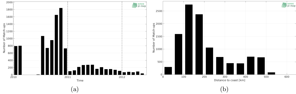
Figure 1: Number of match-ups between Surface drifters and SMOS SSS L3 v4 - 18 Days (CATDS-CECOS-LOCEAN) SSS as a function of time (a) and as function of the distance to coast (b) over the Arctic Ocean Pi-MEP region and for the full satellite product period.
