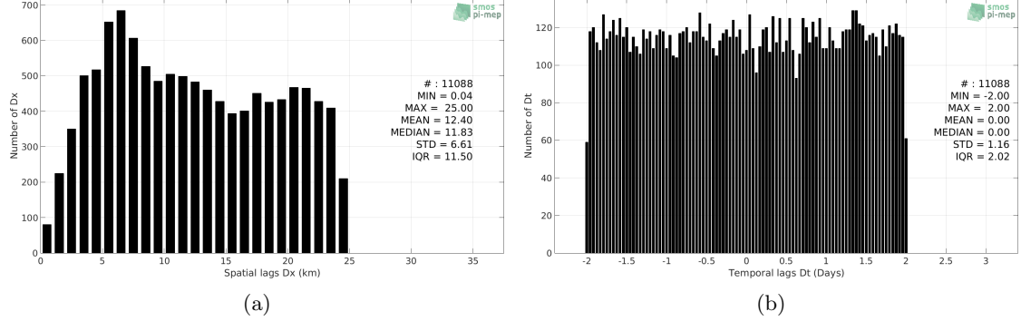
Figure 4: Histograms of the spatial (a) and temporal (b) lags between the time of the Surface drifters measurements and the date of the corresponding SMOS SSS L3 v4 - 18 Days (CATDS-CECOS-LOCEAN) SSS product.
