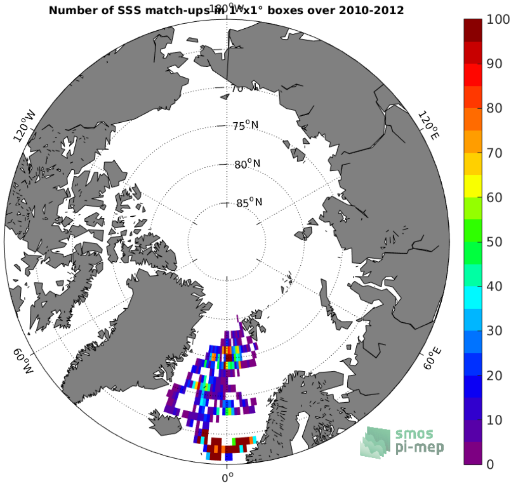
Figure 3: Number of SSS match-ups between Surface drifters SSS and the SMOS-L3-CATDS-CECOS-LOCEAN-V4-18DAYS-25KM SSS product for the Arctic Ocean Pi-MEP region over 1^\circ \times 1^\circ boxes and for the full satellite product period.
