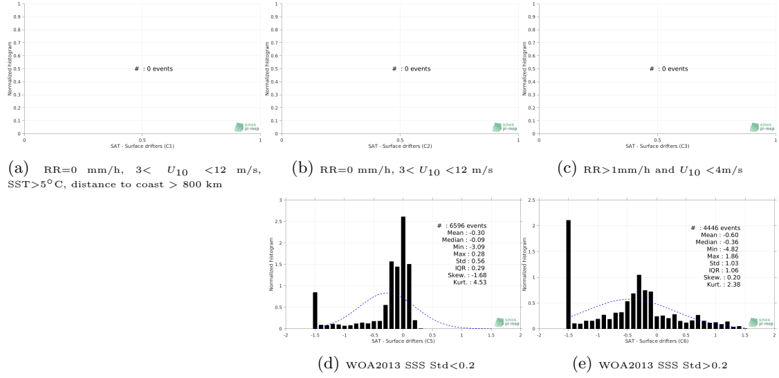
Figure 12: Normalized histogram of \Delta\text{SSS} (SMOS-L3-CATDS-CECOS-LOCEAN-V4-18DAYS-25KM - Surface drifters) for 5 different subdatasets corresponding to: RR=0 mm/h, 3 < U_{10} < 12 m/s, SST > 5^{\circ}\text{C} , distance to coast > 800 km (a), RR=0 mm/h, 3 < U_{10} < 12 m/s (b), RR > 1\text{mm/h} and U_{10} < 4\text{m/s} (c), WOA2013 SSS Std<0.2 (d), WOA2013 SSS Std>0.2 (e).
