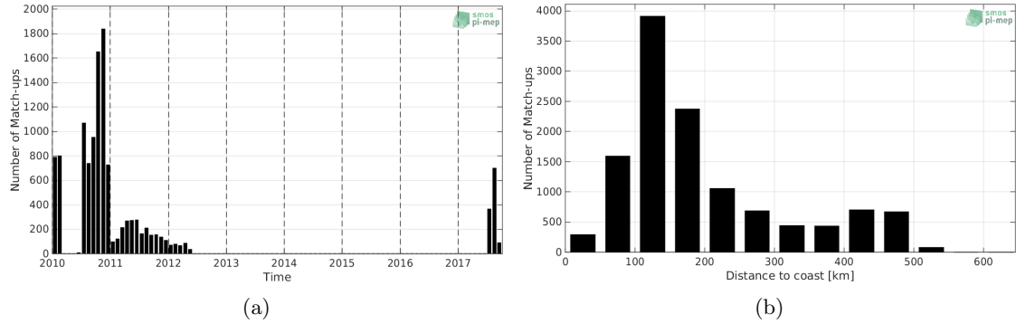
Figure 1: Number of match-ups between Surface drifters and SMOS-L3-CATDS-CECOS-LOCEAN-V4-18DAYS-25KM SSS as a function of time (a) and as function of the distance to coast (b) over the Arctic Ocean Pi-MEP region and for the full satellite product period.
