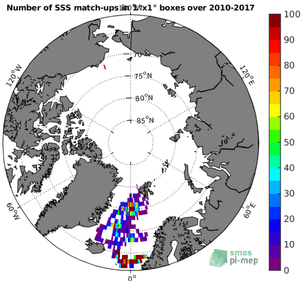
Figure 3: Number of SSS match-ups between Surface drifters SSS and the SMOS-L3-CATDS-CECOS-LOCEAN-V4-18DAYS-25KM SSS product for the Arctic Ocean Pi-MEP region over 1°x1° boxes and for the full satellite product period.
