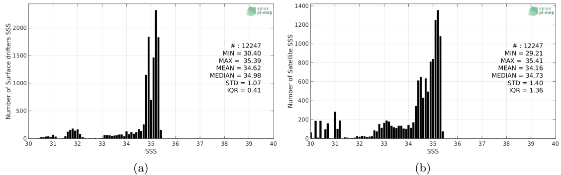
Figure 2: Histograms of SSS from Surface drifters (a) and SMOS-L3-CATDS-CECOS-LOCEAN-V4-18DAYS-25KM (b) considering all match-up pairs per bins of 0.1 over the Arctic Ocean Pi-MEP region and for the full satellite product period.
