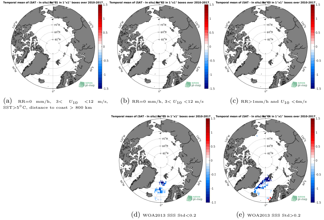
Figure 11: Temporal mean gridded over spatial boxes of size 1^\circ \times 1^\circ of \Delta SSS (SMOS-L3-CATDS-CECOS-LOCEAN-V4-18DAYS-25KM - Surface drifters) for 5 different subdatasets corresponding to: RR=0 mm/h, 3 < U_{10} < 12 m/s, SST >5^\circ C, distance to coast > 800 km (a), RR=0 mm/h, 3 < U_{10} < 12 m/s (b), RR >1 mm/h and U_{10} < 4 m/s (c), WOA2013 SSS Std <0.2 (d), WOA2013 SSS Std >0.2 (e).
