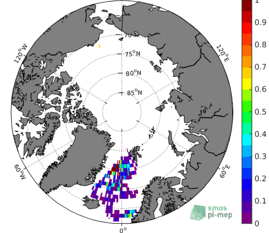
(f) Std( \Delta SSS) (Satellite - Surface drifters)
