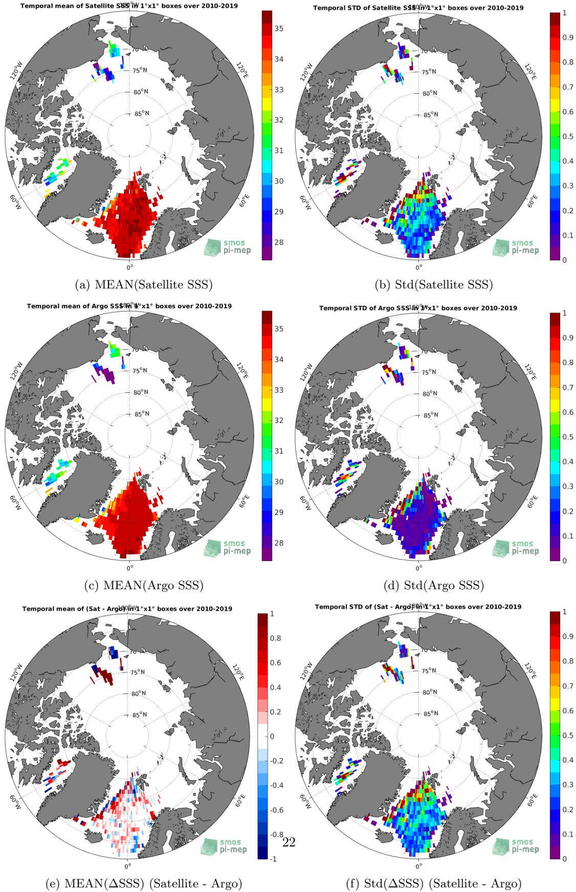
Figure 6: Temporal mean (left) and Std (right) of SSS from SMOS-L3-CATDS-CECOS-LOCEAN-V4-18DAYS-25KM (top), Argo (middle), and of \Delta SSS (Satellite - Argo). Only match-up pairs are used to generate these maps.
