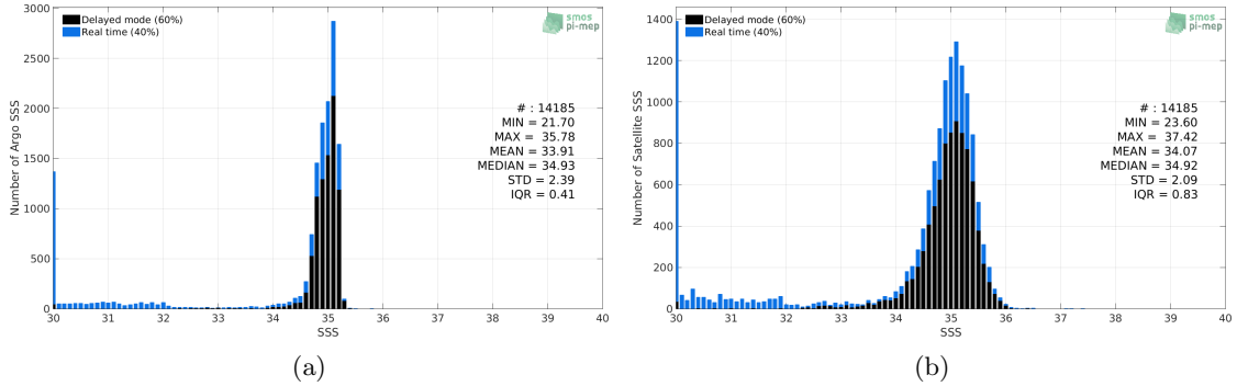
Figure 2: Histograms of SSS from Argo (a) and SMOS-L3-CATDS-CECOS-LOCEAN-V4-18DAYS-25KM (b) considering all match-up pairs per bins of 0.1 over the Arctic Ocean Pi-MEP region and for the full satellite product period.
