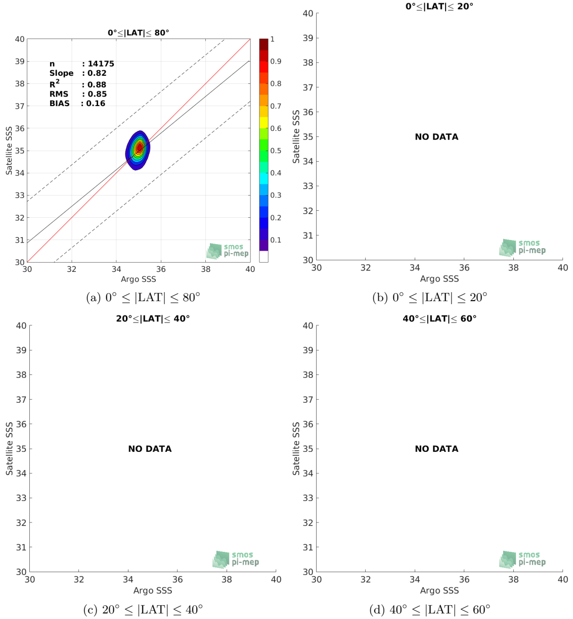
Figure 9: Contour maps of the concentration of SMOS-L3-CATDS-CECOS-LOCEAN-V4-18DAYS-25KM SSS (y-axis) versus Argo SSS (x-axis) at match-up pairs for different latitude bands. For each plot, the red line shows x=y . The black thin and dashed lines indicate a linear fit through the data cloud and the \pm 95\% confidence levels, respectively. The number match-up pairs n , the slope and R^2 coefficient of the linear fit, the root mean square (RMS) and the mean bias between satellite and in situ data are indicated for each latitude band in each plots.
