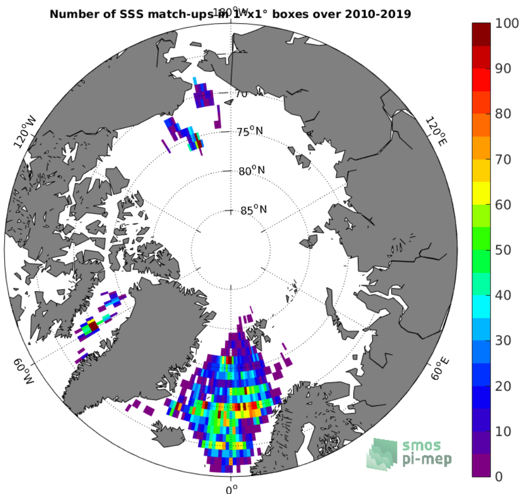
Figure 4: Number of SSS match-ups between Argo SSS and the SMOS-L3-CATDS-CECOS-LOCEAN-V4-18DAYS-25KM SSS product for the Arctic Ocean Pi-MEP region over 1^\circ \times 1^\circ boxes and for the full satellite product period.
