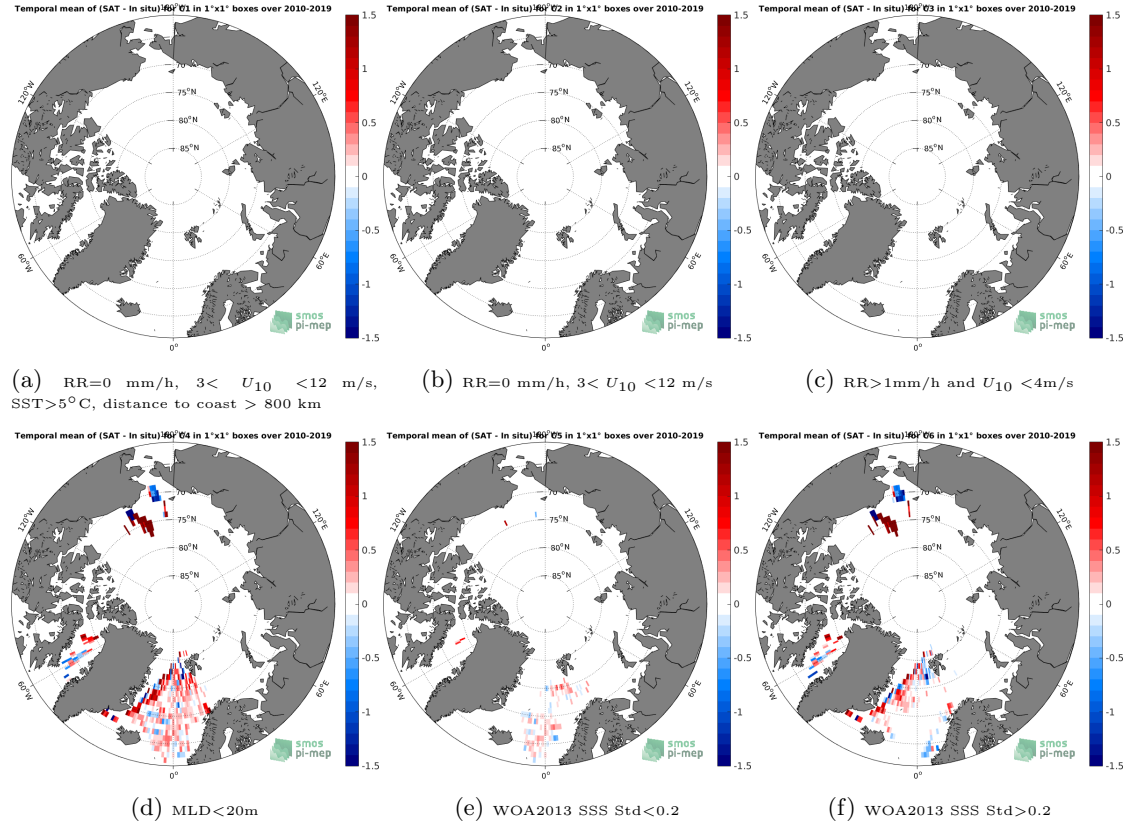
Figure 12: Temporal mean gridded over spatial boxes of size 1^{\circ}\times 1^{\circ} of \Delta\text{SSS} (SMOS-L3-CATDS-CECOS-LOCEAN-V4-18DAYS-25KM - Argo) for 6 different subdatasets corresponding to: RR=0 mm/h, 3 < U_{10} < 12 m/s, SST >5^{\circ}\text{C} , distance to coast > 800 km (a), RR=0 mm/h, 3 < U_{10} < 12 m/s (b), RR >1 mm/h and U_{10} < 4 m/s (c),MLD <20 m (d),WOA2013 SSS Std <0.2 (e),WOA2013 SSS Std >0.2 (f).
