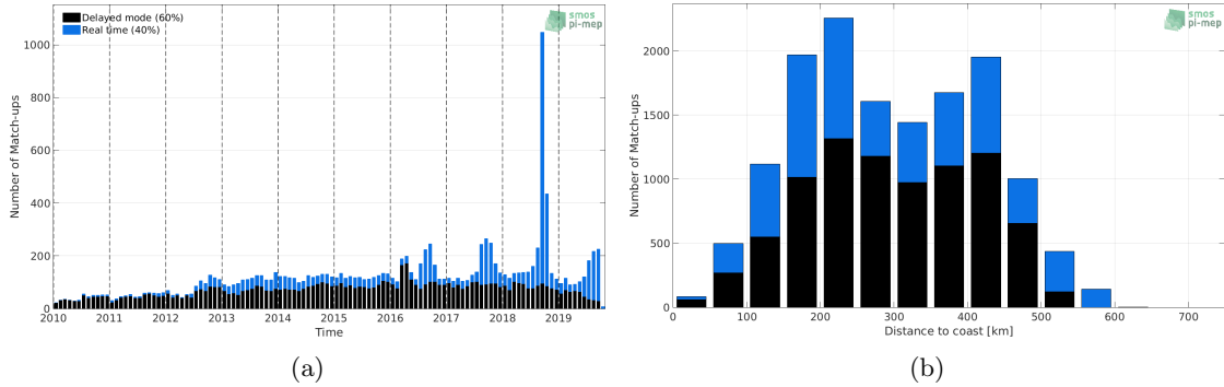
Figure 1: Number of match-ups between Argo and SMOS-L3-CATDS-CECOS-LOCEAN-V4-18DAYS-25KM SSS as a function of time (a) and as function of the distance to coast (b) over the Arctic Ocean Pi-MEP region and for the full satellite product period.
