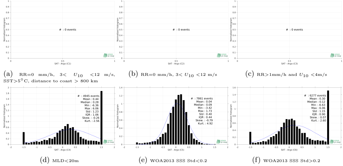
Figure 13: Normalized histogram of \Delta\text{SSS} (SMOS-L3-CATDS-CECOS-LOCEAN-V4-18DAYS-25KM - Argo) for 6 different subdatasets corresponding to: RR=0 mm/h, 3 < U_{10} < 12 m/s, SST > 5^{\circ}\text{C} , distance to coast > 800 km (a), RR=0 mm/h, 3 < U_{10} < 12 m/s (b), RR > 1\text{mm/h} and U_{10} < 4\text{m/s} (c), MLD < 20\text{m} (d), WOA2013 SSS Std < 0.2 (e), WOA2013 SSS Std > 0.2 (f).
