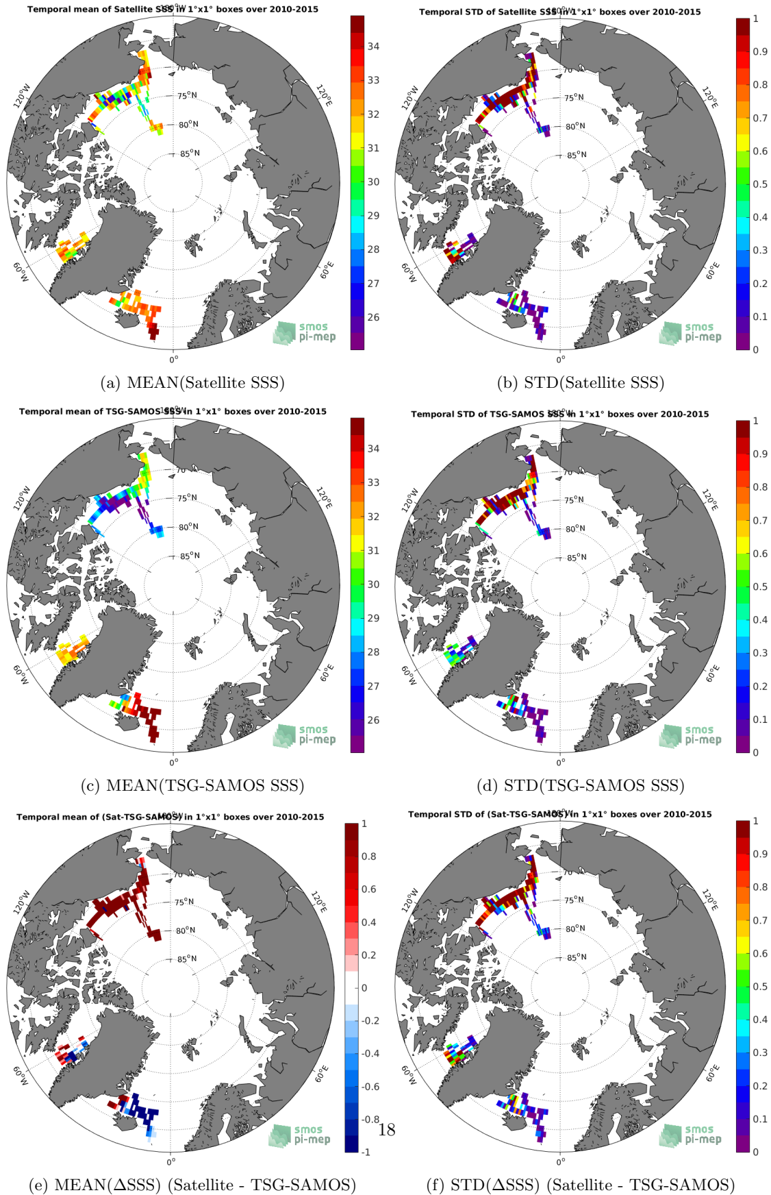
Figure 6: Temporal mean (left) and STD (right) of SSS from SMOS-L3-CATDS-CECOS-LOCEAN-V3-9DAYS-25KM (top), TSG-SAMOS (middle), and of \Delta SSS (Satellite - TSG-SAMOS). Only match-up pairs are used to generate these maps.
