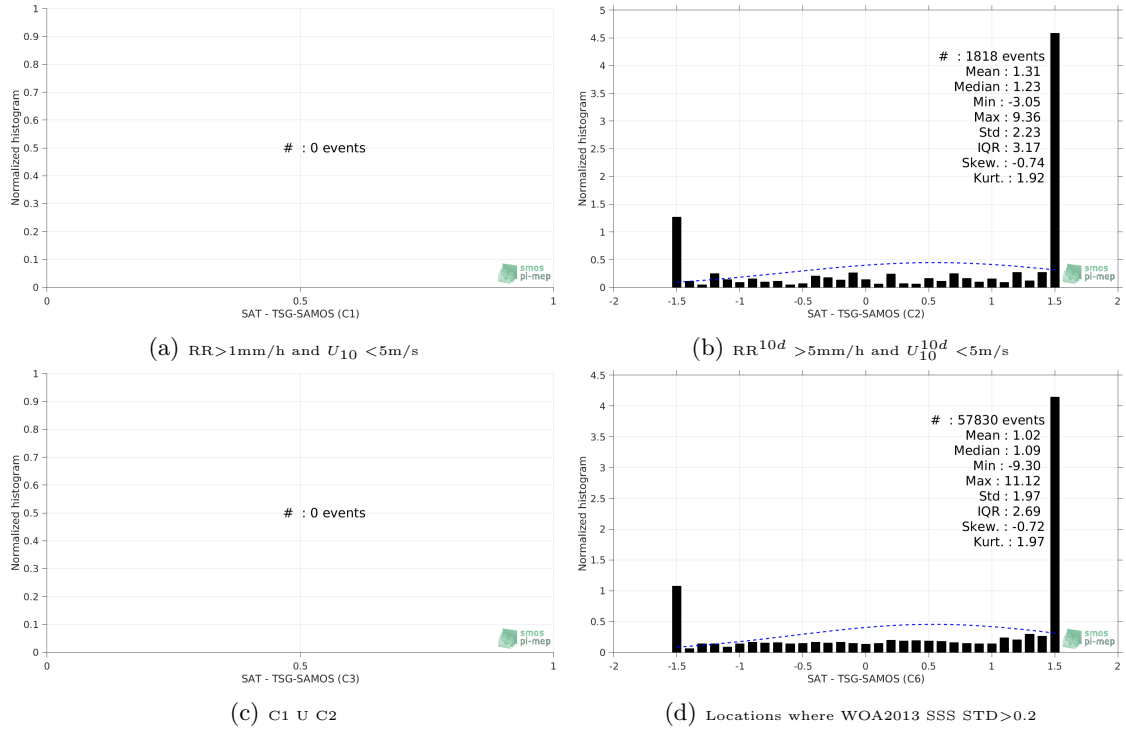
Figure 13: Normalized histogram of \Delta\text{SSS} (SMOS-L3-CATDS-CECOS-LOCEAN-V3-9DAYS-25KM - TSG-SAMOS) for 6 different subdatasets corresponding to: RR > 1\text{mm/h} and U_{10} < 5\text{m/s} (a), RR^{10d} > 5\text{mm/h} and U_{10}^{10d} < 5\text{m/s} (b), C1 \cup C2 (c), Locations where WOA2013 SSS STD > 0.2 (d).
