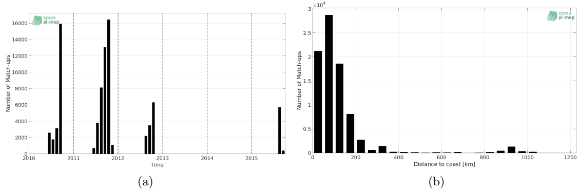
Figure 1: Number of match-ups between TSG-SAMOS and SMOS-L3-CATDS-CECOS-LOCEAN-V3-9DAYS-25KM SSS as a function of time (a) and as function of the distance to coast (b) over the Arctic Ocean Pi-MEP region and for the full satellite product period.
