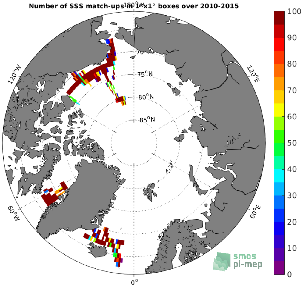
Figure 4: Number of SSS match-ups between TSG-SAMOS SSS and the SMOS-L3-CATDS-CECOS-LOCEAN-V3-9DAYS-25KM SSS product for the Arctic Ocean Pi-MEP region over 1°x1° boxes and for the full satellite product period.
