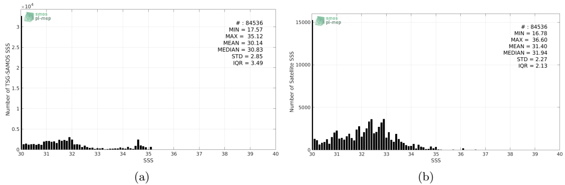
Figure 2: Histograms of SSS from TSG-SAMOS (a) and SMOS-L3-CATDS-CECOS-LOCEAN-V3-9DAYS-25KM (b) considering all match-up pairs per bins of 0.1 over the Arctic Ocean Pi-MEP region and for the full satellite product period.
