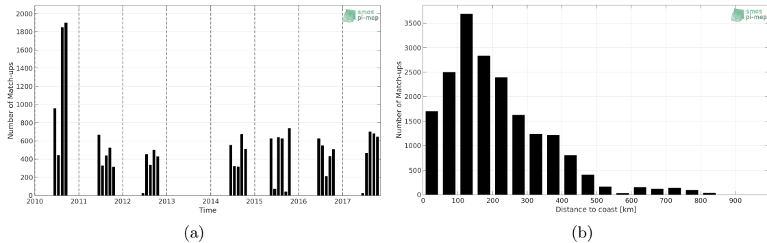
Figure 1: Number of match-ups between TSG-POLARSTERN and SMOS-L3-CATDS-CECOS-LOCEAN-V3-9DAYS-25KM SSS as a function of time (a) and as function of the distance to coast (b) over the Arctic Ocean Pi-MEP region and for the full satellite product period.
