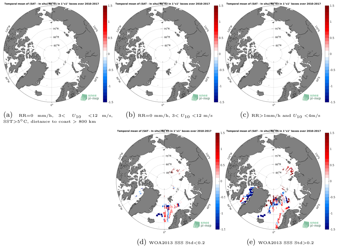
Figure 12: Temporal mean gridded over spatial boxes of size 1^\circ \times 1^\circ of \Delta SSS (SMOS-L3-CATDS-CECOS-LOCEAN-V3-9DAYS-25KM - TSG-POLARSTERN) for 5 different subdatasets corresponding to:RR=0 mm/h, 3 < U_{10} < 12 m/s, SST > 5^\circ\text{C} , distance to coast > 800 km (a), RR=0 mm/h, 3 < U_{10} < 12 m/s (b), RR > 1 mm/h and U_{10} < 4 m/s (c), WOA2013 SSS Std < 0.2 (d), WOA2013 SSS Std > 0.2 (e).
