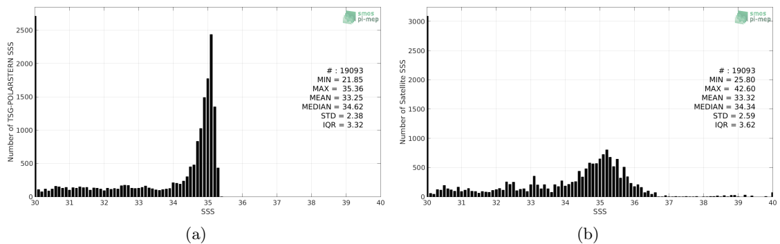
Figure 2: Histograms of SSS from TSG-POLARSTERN (a) and SMOS-L3-CATDS-CECOS-LOCEAN-V3-9DAYS-25KM (b) considering all match-up pairs per bins of 0.1 over the Arctic Ocean Pi-MEP region and for the full satellite product period.
