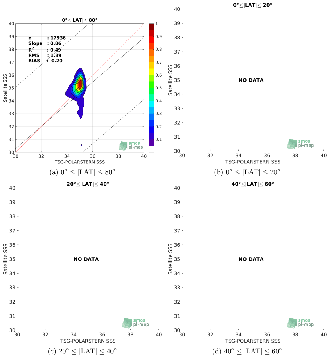
Figure 9: Contour maps of the concentration of SMOS-L3-CATDS-CECOS-LOCEAN-V3-9DAYS-25KM SSS ( y -axis) versus TSG-POLARSTERN SSS ( x -axis) at match-up pairs for different latitude bands. For each plot, the red line shows x=y . The black thin and dashed lines indicate a linear fit through the data cloud and the \pm 95\% confidence levels, respectively. The number match-up pairs n , the slope and R^2 coefficient of the linear fit, the root mean square (RMS) and the mean bias between satellite and in situ data are indicated for each latitude band in each plots.
