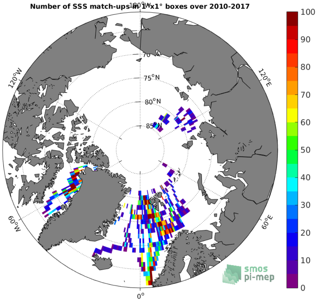
Figure 4: Number of SSS match-ups between TSG-POLARSTERN SSS and the SMOS-L3-CATDS-CECOS-LOCEAN-V3-9DAYS-25KM SSS product for the Arctic Ocean Pi-MEP region over 1°x1° boxes and for the full satellite product period.
