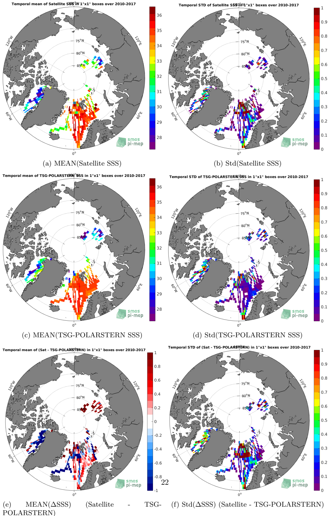
Figure 6: Temporal mean (left) and Std (right) of SSS from SMOS-L3-CATDS-CECOS-LOCEAN-V3-9DAYS-25KM (top), TSG-POLARSTERN (middle), and of \Delta SSS (Satellite - TSG-POLARSTERN). Only match-up pairs are used to generate these maps.
