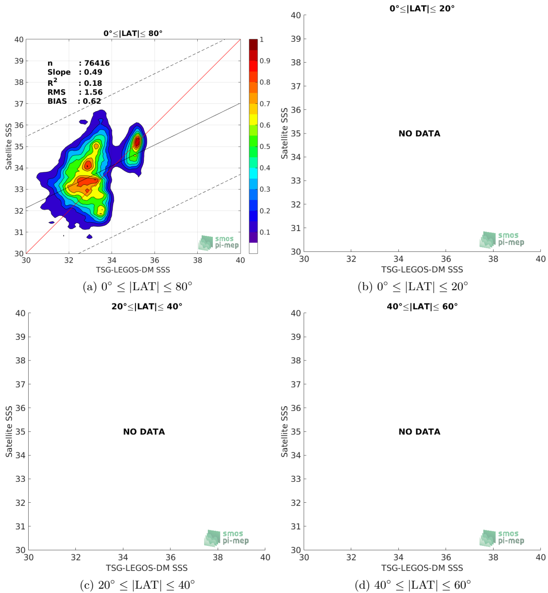
Figure 9: Contour maps of the concentration of SMOS-L3-CATDS-CECOS-LOCEAN-V3-9DAYS-25KM SSS (y-axis) versus TSG-LEGOS-DM SSS (x-axis) at match-up pairs for different latitude bands. For each plot, the red line shows x=y . The black thin and dashed lines indicate a linear fit through the data cloud and the \pm 95\% confidence levels, respectively. The number match-up pairs n , the slope and R^2 coefficient of the linear fit, the root mean square (RMS) and the mean bias between satellite and in situ data are indicated for each latitude band in each plots.
