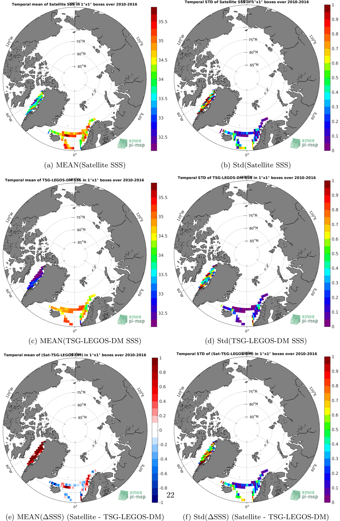
Figure 6: Temporal mean (left) and Std (right) of SSS from SMOS-L3-CATDS-CECOS-LOCEAN-V3-9DAYS-25KM (top), TSG-LEGOS-DM (middle), and of \Delta SSS (Satellite - TSG-LEGOS-DM). Only match-up pairs are used to generate these maps.
