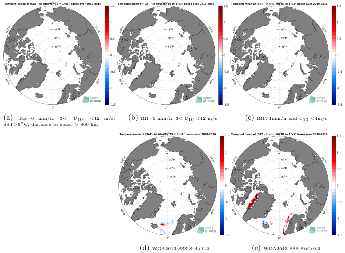
Figure 12: Temporal mean gridded over spatial boxes of size 1^\circ \times 1^\circ of \Delta SSS (SMOS-L3-CATDS-CECOS-LOCEAN-V3-9DAYS-25KM - TSG-LEGOS-DM) for 5 different subdatasets corresponding to:RR=0 mm/h, 3 < U_{10} < 12 m/s, SST >5^\circ C, distance to coast > 800 km (a), RR=0 mm/h, 3 < U_{10} < 12 m/s (b), RR >1 mm/h and U_{10} < 4 m/s (c), WOA2013 SSS Std <0.2 (d), WOA2013 SSS Std >0.2 (e).
