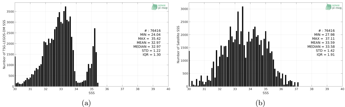
Figure 2: Histograms of SSS from TSG-LEGOS-DM (a) and SMOS-L3-CATDS-CECOS-LOCEAN-V3-9DAYS-25KM (b) considering all match-up pairs per bins of 0.1 over the Arctic Ocean Pi-MEP region and for the full satellite product period.
