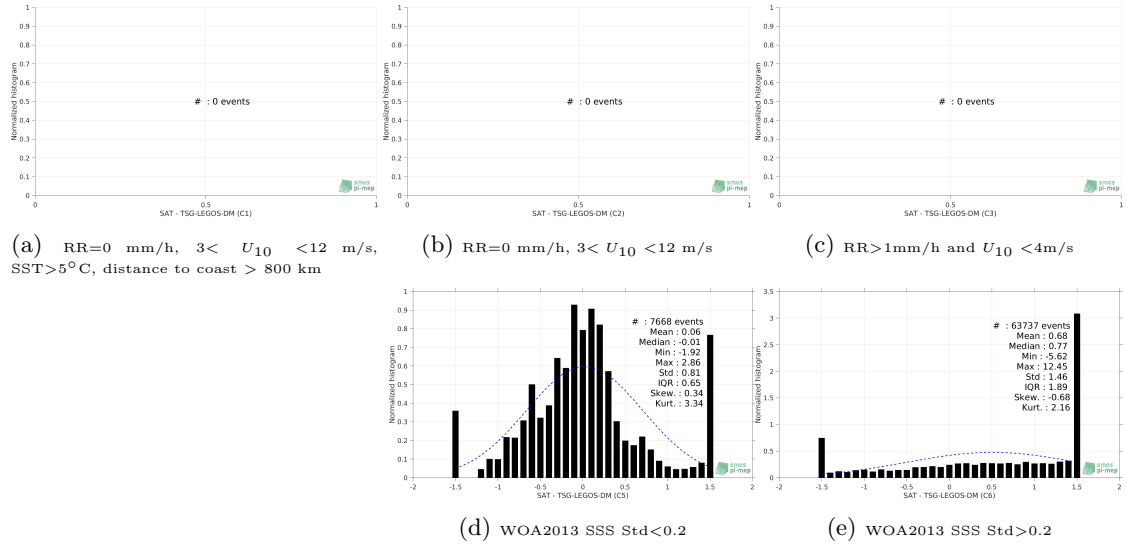
Figure 13: Normalized histogram of \Delta SSS (SMOS-L3-CATDS-CECOS-LOCEAN-V3-9DAYS-25KM - TSG-LEGOS-DM) for 5 different subdatasets corresponding to: RR=0 mm/h, 3 < U_{10} < 12 m/s, SST > 5°C, distance to coast > 800 km (a), RR=0 mm/h, 3 < U_{10} < 12 m/s (b), RR > 1mm/h and U_{10} < 4 m/s (c), WOA2013 SSS Std < 0.2 (d), WOA2013 SSS Std > 0.2 (e).
