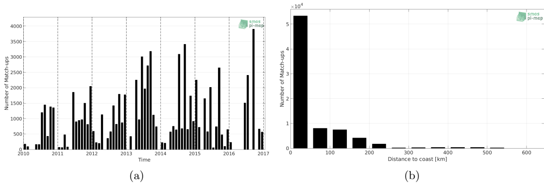
Figure 1: Number of match-ups between TSG-LEGOS-DM and SMOS-L3-CATDS-CECOS-LOCEAN-V3-9DAYS-25KM SSS as a function of time (a) and as function of the distance to coast (b) over the Arctic Ocean Pi-MEP region and for the full satellite product period.
