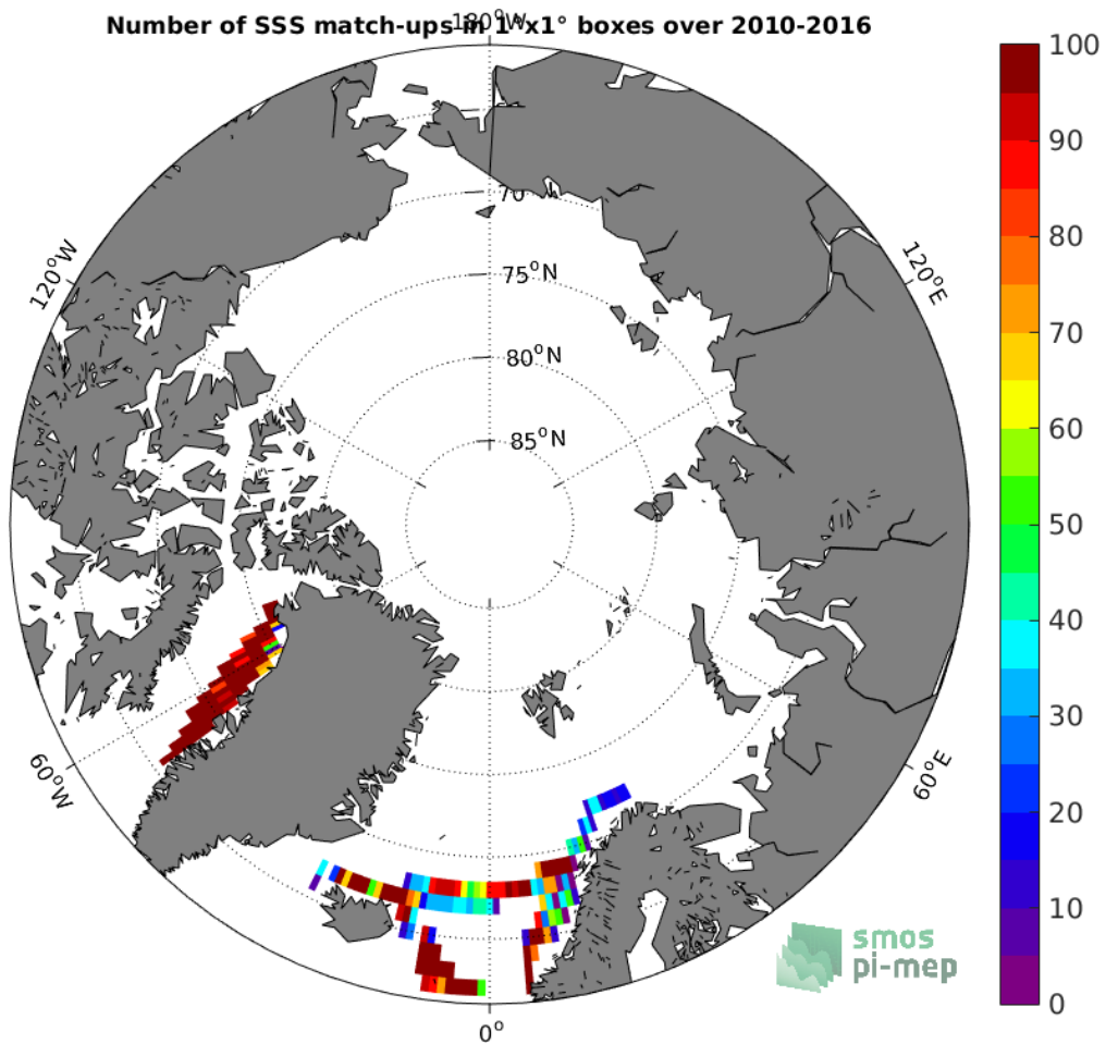
Figure 4: Number of SSS match-ups between TSG-LEGOS-DM SSS and the SMOS-L3-CATDS-CECOS-LOCEAN-V3-9DAYS-25KM SSS product for the Arctic Ocean Pi-MEP region over 1^\circ \times 1^\circ boxes and for the full satellite product period.
