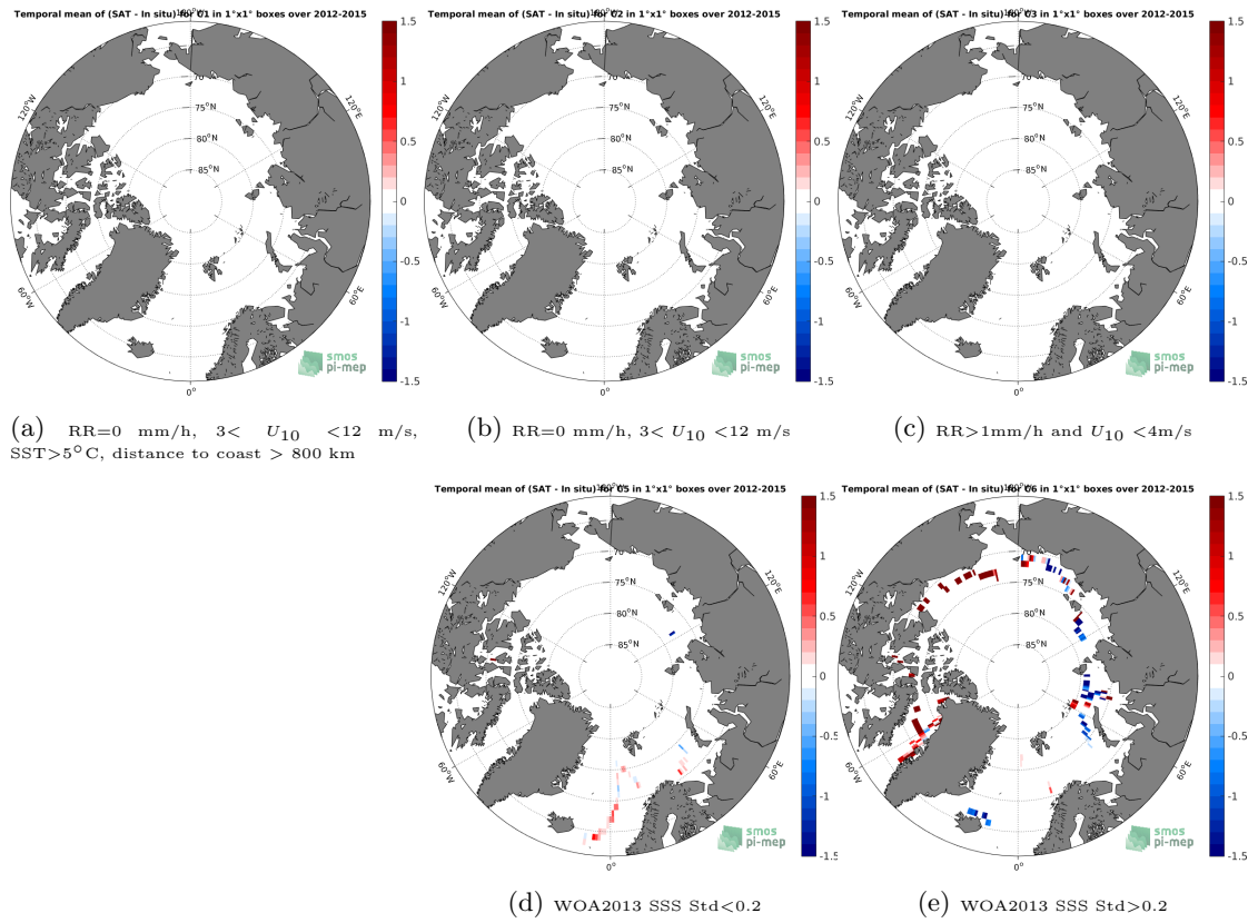
Figure 12: Temporal mean gridded over spatial boxes of size 1^\circ \times 1^\circ of \Delta SSS (SMOS-L3-CATDS-CECOS-LOCEAN-V3-9DAYS-25KM - TSG-GOSUD-Sailing-ship) for 5 different subdatasets corresponding to:RR=0 mm/h, 3 < U_{10} < 12 m/s, SST>5°C, distance to coast > 800 km (a), RR=0 mm/h, 3 < U_{10} < 12 m/s (b), RR>1mm/h and U_{10} < 4 m/s (c), WOA2013 SSS Std<0.2 (d), WOA2013 SSS Std>0.2 (e).
