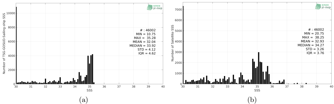
Figure 2: Histograms of SSS from TSG-GOSUD-Sailing-ship (a) and SMOS-L3-CATDS-CECOS-LOCEAN-V3-9DAYS-25KM (b) considering all match-up pairs per bins of 0.1 over the Arctic Ocean Pi-MEP region and for the full satellite product period.
