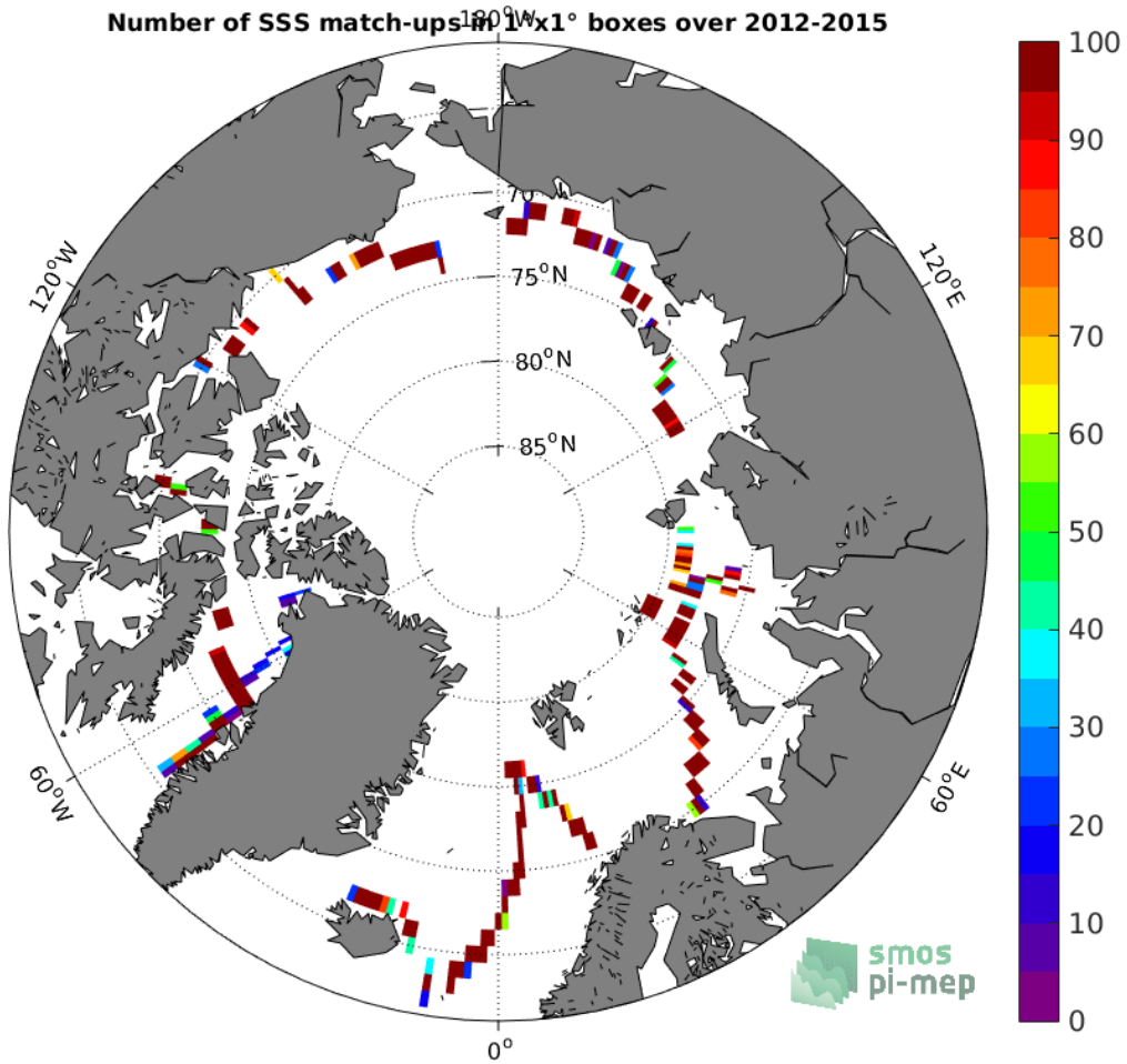
Figure 4: Number of SSS match-ups between TSG-GOSUD-Sailing-ship SSS and the SMOS-L3-CATDS-CECOS-LOCEAN-V3-9DAYS-25KM SSS product for the Arctic Ocean Pi-MEP region over 1°x1° boxes and for the full satellite product period.
