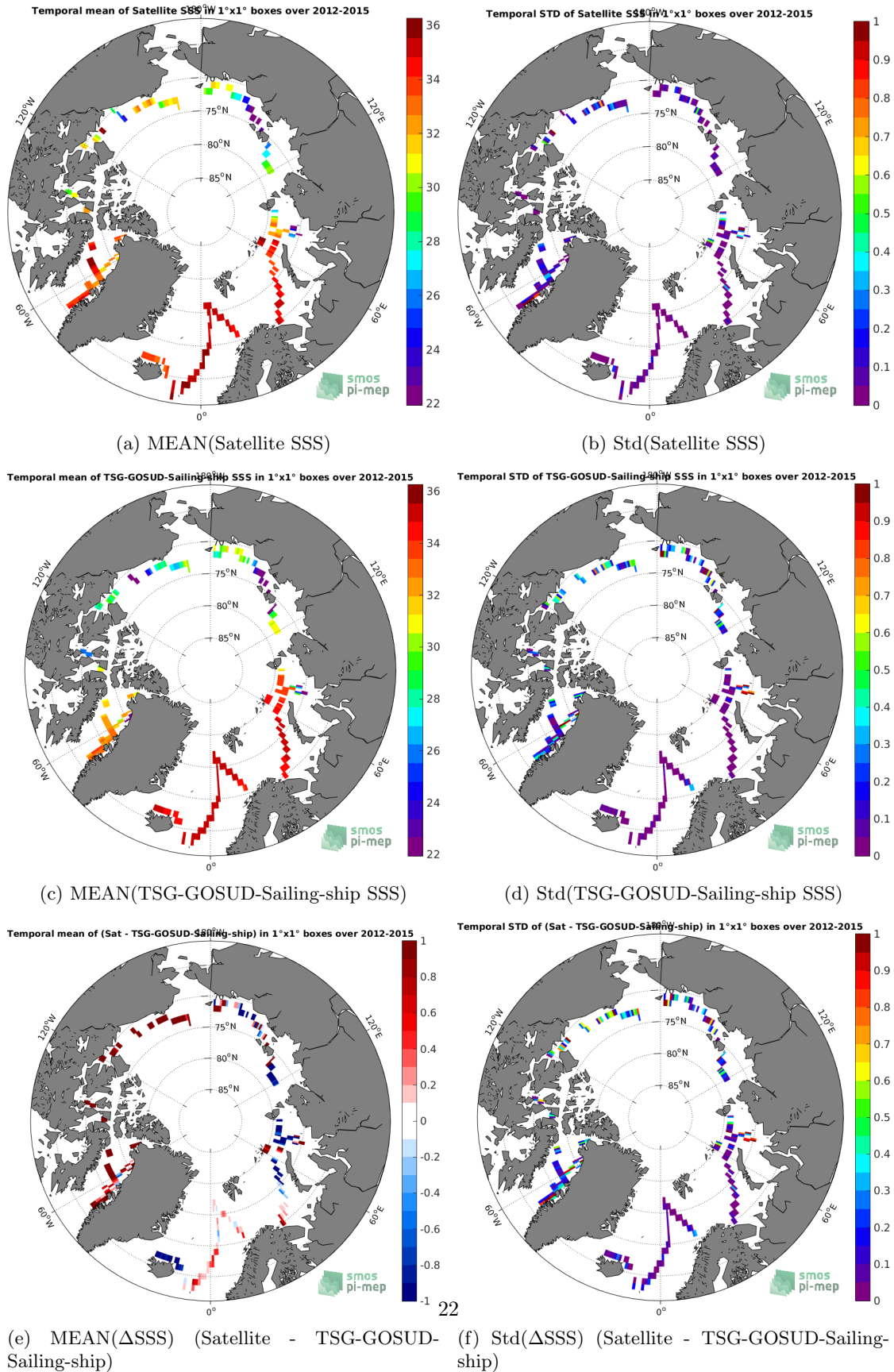
Figure 6: Temporal mean (left) and Std (right) of SSS from SMOS-L3-CATDS-CECOS-LOCEAN-V3-9DAYS-25KM (top), TSG-GOSUD-Sailing-ship (middle), and of \Delta SSS (Satellite - TSG-GOSUD-Sailing-ship). Only match-up pairs are used to generate these maps.
