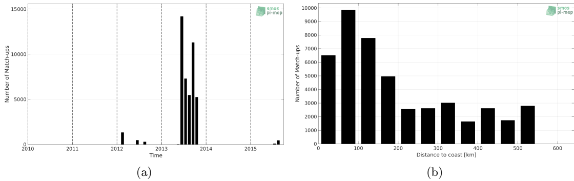
Figure 1: Number of match-ups between TSG-GOSUD-Sailing-ship and SMOS-L3-CATDS-CECOS-LOCEAN-V3-9DAYS-25KM SSS as a function of time (a) and as function of the distance to coast (b) over the Arctic Ocean Pi-MEP region and for the full satellite product period.
