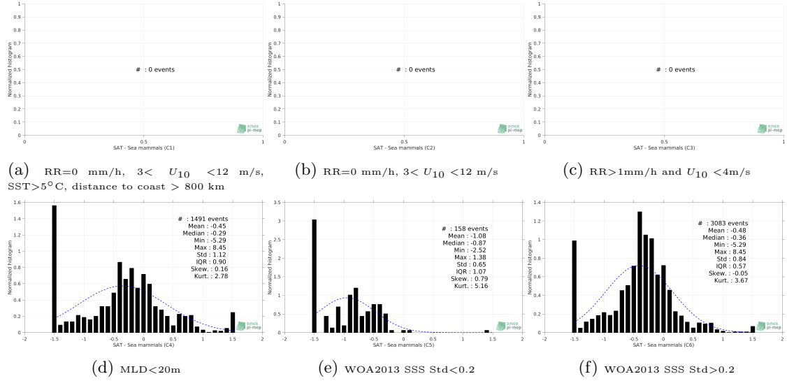
Figure 13: Normalized histogram of \Delta\text{SSS} (SMOS-L3-CATDS-CECOS-LOCEAN-V3-9DAYS-25KM - Sea mammals) for 6 different subdatasets corresponding to: RR=0 mm/h, 3 < U_{10} < 12 m/s, SST > 5^\circ\text{C} , distance to coast > 800 km (a), RR=0 mm/h, 3 < U_{10} < 12 m/s (b), RR > 1\text{mm/h} and U_{10} < 4\text{m/s} (c), MLD < 20\text{m} (d), WOA2013 SSS Std < 0.2 (e), WOA2013 SSS Std > 0.2 (f).
