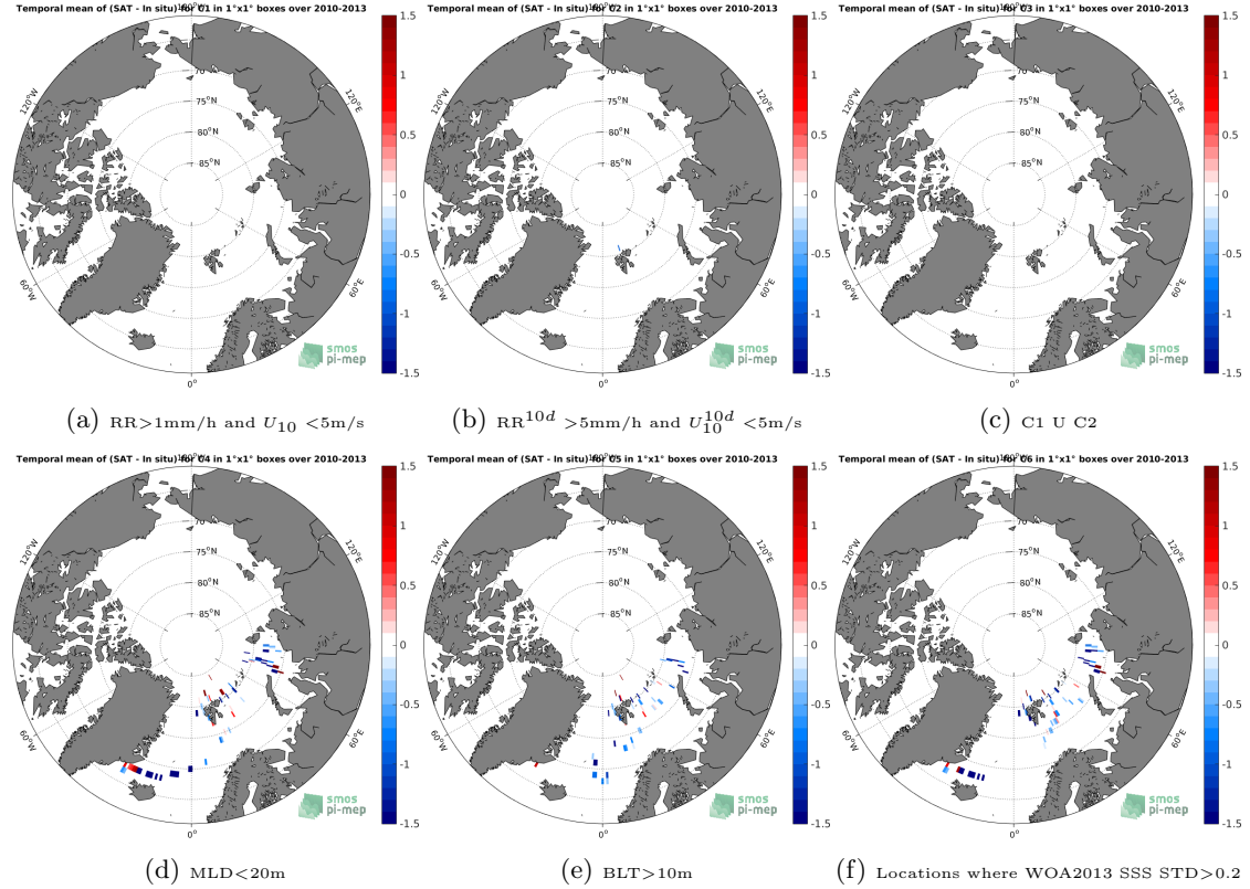
Figure 12: Temporal mean gridded over spatial boxes of size 1^\circ \times 1^\circ of \Delta\text{SSS} (SMOS-L3-CATDS-CECOS-LOCEAN-V3-9DAYS-25KM - Sea mammals) for 6 different subdatasets corresponding to: \text{RR} > 1\text{mm/h} and U_{10} < 5\text{m/s} (a), \text{RR}^{10d} > 5\text{mm/h} and U_{10}^{10d} < 5\text{m/s} (b), C1 U C2 (c), \text{MLD} < 20\text{m} (d), \text{BLT} > 10\text{m} (e), Locations where WOA2013 SSS STD > 0.2 (f).
