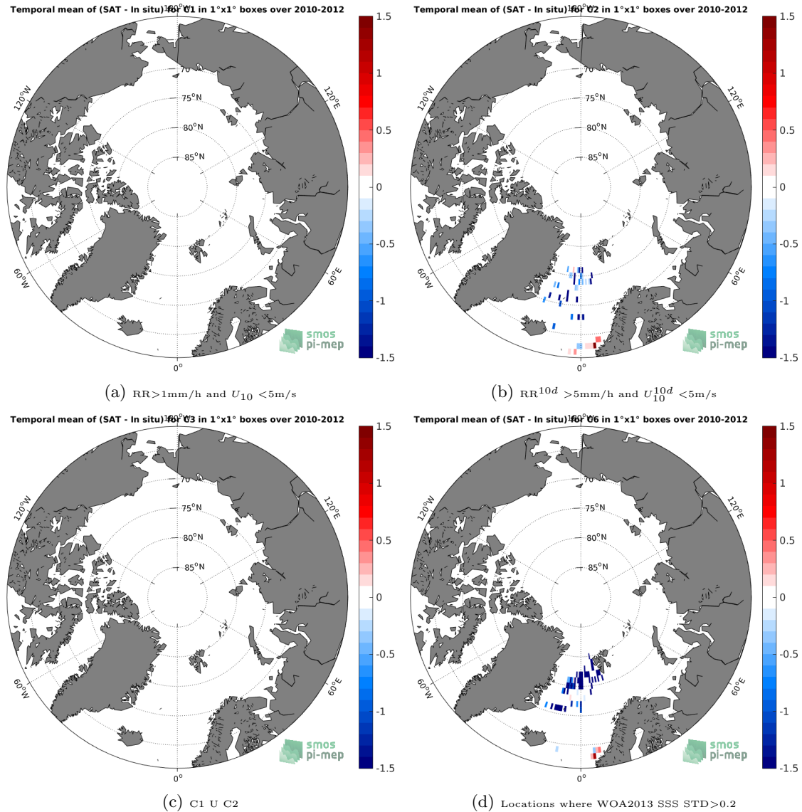
Figure 11: Temporal mean gridded over spatial boxes of size 1^\circ \times 1^\circ of \Delta SSS (SMOS-L3-CATDS-CECOS-LOCEAN-V3-9DAYS-25KM - Surface drifters) for 4 different subdatasets corresponding to: RR > 1\text{mm/h} and U_{10} < 5\text{m/s} (a), RR^{10d} > 5\text{mm/h} and U_{10}^{10d} < 5\text{m/s} (b), C1 U C2 (c), Locations where WOA2013 SSS STD > 0.2 (d).
