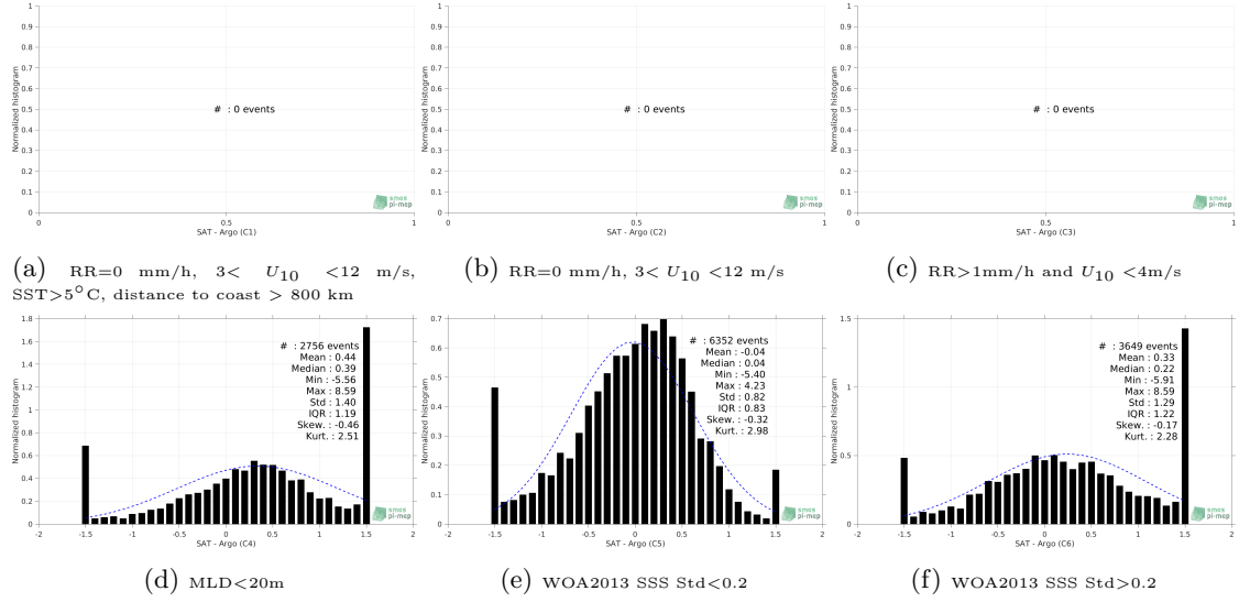
Figure 13: Normalized histogram of \Delta\text{SSS} (SMOS-L3-CATDS-CECOS-LOCEAN-V3-9DAYS-25KM - Argo) for 6 different subdatasets corresponding to: RR=0 mm/h, 3 < U_{10} < 12 m/s, SST > 5^\circ\text{C} , distance to coast > 800 km (a), RR=0 mm/h, 3 < U_{10} < 12 m/s (b), RR > 1 mm/h and U_{10} < 4 m/s (c), MLD < 20 m (d), WOA2013 SSS Std < 0.2 (e), WOA2013 SSS Std > 0.2 (f).
