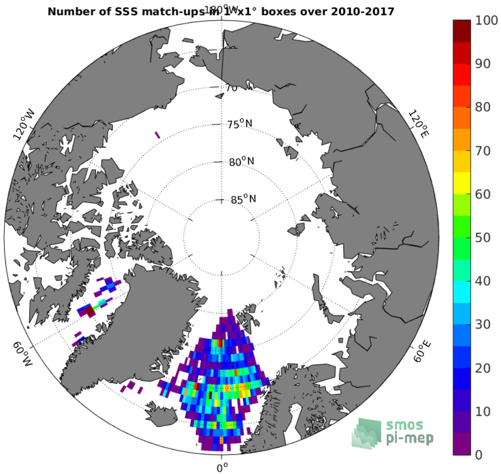
Figure 4: Number of SSS match-ups between Argo SSS and the SMOS-L3-CATDS-CECOS-LOCEAN-V3-9DAYS-25KM SSS product for the Arctic Ocean Pi-MEP region over 1^\circ \times 1^\circ boxes and for the full satellite product period.
