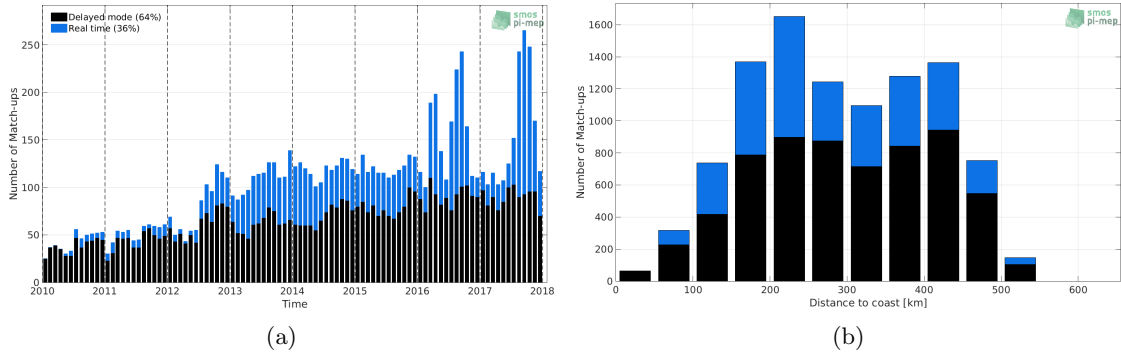
Figure 1: Number of match-ups between Argo and SMOS-L3-CATDS-CECOS-LOCEAN-V3-9DAYS-25KM SSS as a function of time (a) and as function of the distance to coast (b) over the Arctic Ocean Pi-MEP region and for the full satellite product period.
