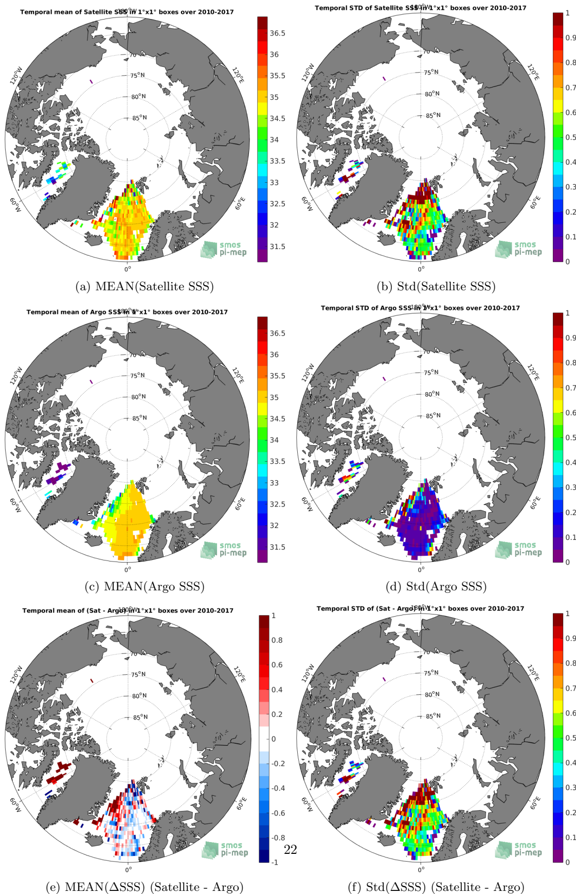
Figure 6: Temporal mean (left) and Std (right) of SSS from SMOS-L3-CATDS-CECOS-LOCEAN-V3-9DAYS-25KM (top), Argo (middle), and of \Delta SSS (Satellite - Argo). Only match-up pairs are used to generate these maps.
