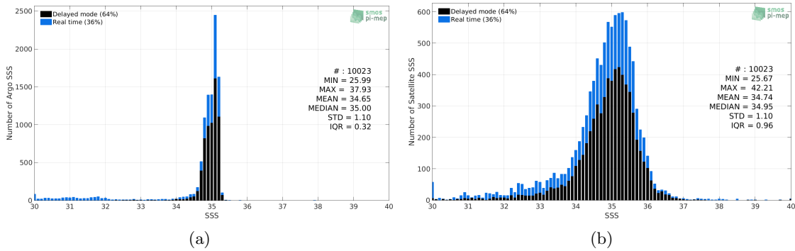
Figure 2: Histograms of SSS from Argo (a) and SMOS-L3-CATDS-CECOS-LOCEAN-V3-9DAYS-25KM (b) considering all match-up pairs per bins of 0.1 over the Arctic Ocean Pi-MEP region and for the full satellite product period.
