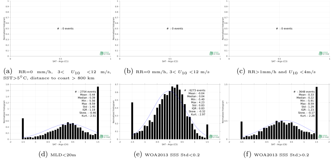
Figure 13: Normalized histogram of \Delta\text{SSS} (SMOS-L3-CATDS-CECOS-LOCEAN-V3-9DAYS-25KM - Argo) for 6 different subdatasets corresponding to: RR=0 mm/h, 3 < U_{10} < 12 m/s, SST > 5^{\circ}\text{C} , distance to coast > 800 km (a), RR=0 mm/h, 3 < U_{10} < 12 m/s (b), RR > 1\text{mm/h} and U_{10} < 4\text{m/s} (c), MLD < 20\text{m} (d), WOA2013 SSS Std < 0.2 (e), WOA2013 SSS Std > 0.2 (f).
