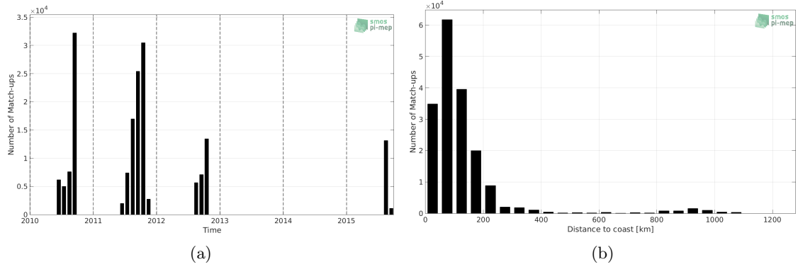
Figure 1: Number of match-ups between TSG-SAMOS and SMOS-L3-CATDS-CECOS-LOCEAN-V3-18DAYS-25KM SSS as a function of time (a) and as function of the distance to coast (b) over the Arctic Ocean Pi-MEP region and for the full satellite product period.
