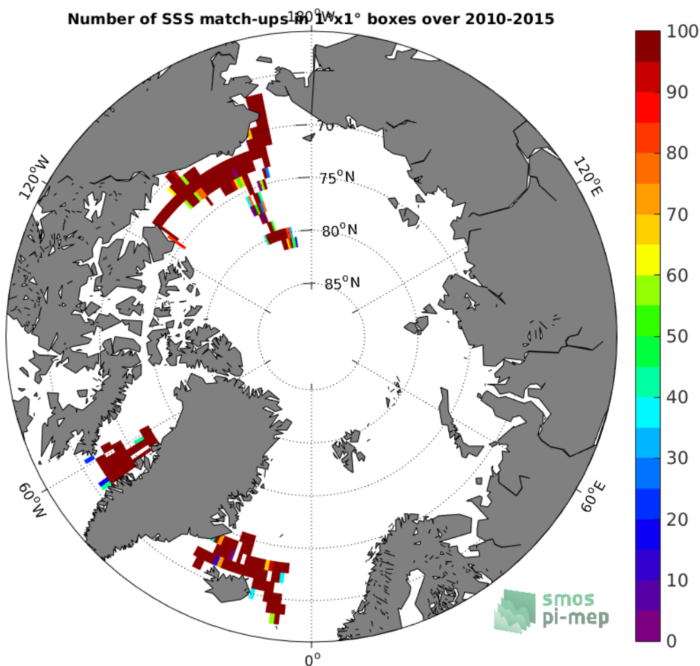
Figure 4: Number of SSS match-ups between TSG-SAMOS SSS and the SMOS-L3-CATDS-CECOS-LOCEAN-V3-18DAYS-25KM SSS product for the Arctic Ocean Pi-MEP region over 1^\circ \times 1^\circ boxes and for the full satellite product period.
