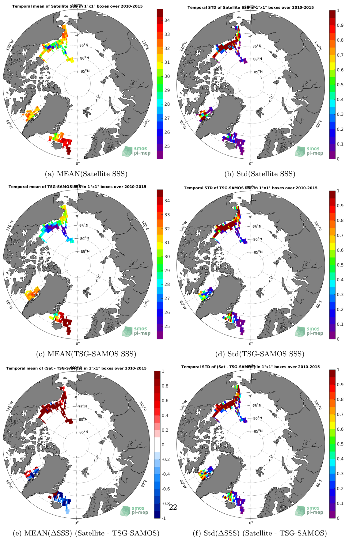
Figure 6: Temporal mean (left) and Std (right) of SSS from SMOS-L3-CATDS-CECOS-LOCEAN-V3-18DAYS-25KM (top), TSG-SAMOS (middle), and of \Delta SSS (Satellite - TSG-SAMOS). Only match-up pairs are used to generate these maps.
