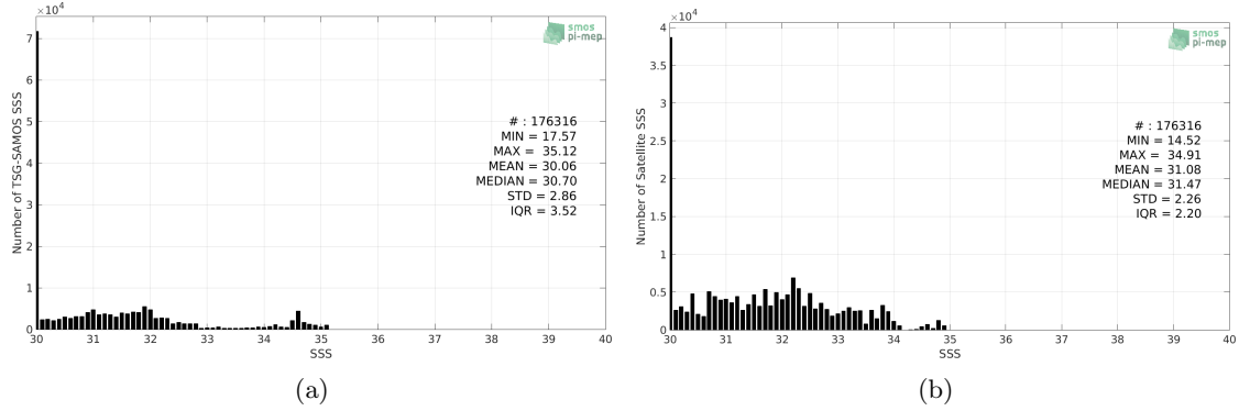
Figure 2: Histograms of SSS from TSG-SAMOS (a) and SMOS-L3-CATDS-CECOS-LOCEAN-V3-18DAYS-25KM (b) considering all match-up pairs per bins of 0.1 over the Arctic Ocean Pi-MEP region and for the full satellite product period.
