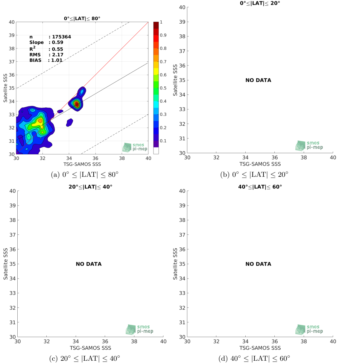
Figure 9: Contour maps of the concentration of SMOS-L3-CATDS-CECOS-LOCEAN-V3-18DAYS-25KM SSS (y-axis) versus TSG-SAMOS SSS (x-axis) at match-up pairs for different latitude bands. For each plot, the red line shows x=y . The black thin and dashed lines indicate a linear fit through the data cloud and the \pm 95\% confidence levels, respectively. The number match-up pairs n , the slope and R^2 coefficient of the linear fit, the root mean square (RMS) and the mean bias between satellite and in situ data are indicated for each latitude band in each plots.
