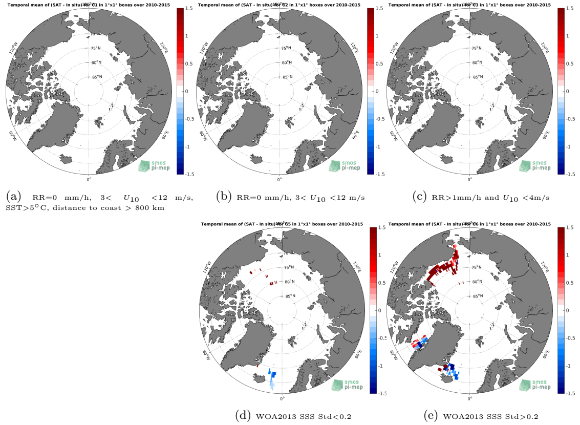
Figure 12: Temporal mean gridded over spatial boxes of size 1^\circ \times 1^\circ of \Delta SSS (SMOS-L3-CATDS-CECOS-LOCEAN-V3-18DAYS-25KM - TSG-SAMOS) for 5 different subdatasets corresponding to: RR=0 mm/h, 3 < U_{10} < 12 m/s, SST > 5^\circ C , distance to coast > 800 km (a), RR=0 mm/h, 3 < U_{10} < 12 m/s (b), RR > 1 mm/h and U_{10} < 4 m/s (c), WOA2013 SSS Std < 0.2 (d), WOA2013 SSS Std > 0.2 (e).
