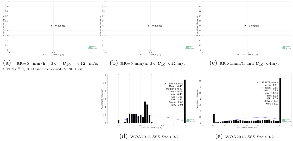
Figure 13: Normalized histogram of \Delta\text{SSS} (SMOS-L3-CATDS-CECOS-LOCEAN-V3-18DAYS-25KM - TSG-SAMOS) for 5 different subdatasets corresponding to: RR=0 mm/h, 3 < U_{10} < 12 m/s, SST > 5^{\circ}\text{C} , distance to coast > 800 km (a), RR=0 mm/h, 3 < U_{10} < 12 m/s (b), RR > 1\text{mm/h} and U_{10} < 4\text{m/s} (c), WOA2013 SSS Std<0.2 (d), WOA2013 SSS Std>0.2 (e).
