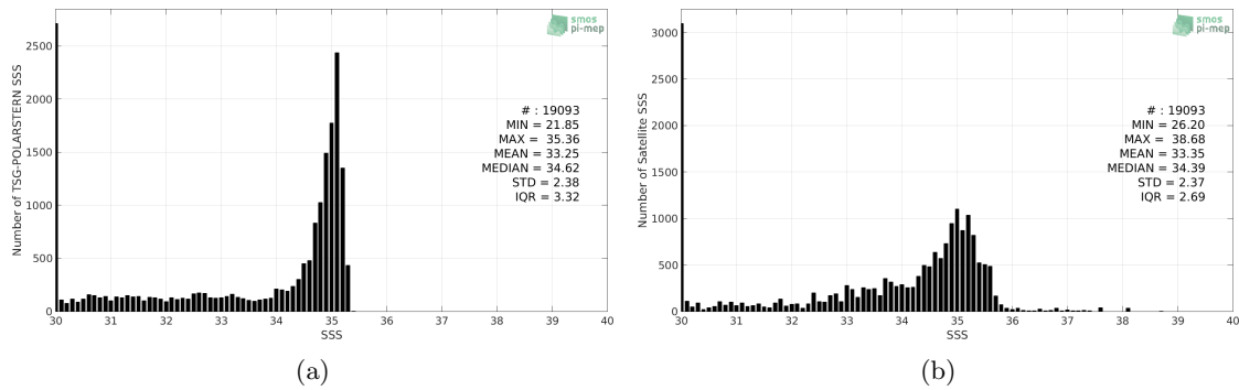
Figure 2: Histograms of SSS from TSG-POLARSTERN (a) and SMOS-L3-CATDS-CECOS-LOCEAN-V3-18DAYS-25KM (b) considering all match-up pairs per bins of 0.1 over the Arctic Ocean Pi-MEP region and for the full satellite product period.
