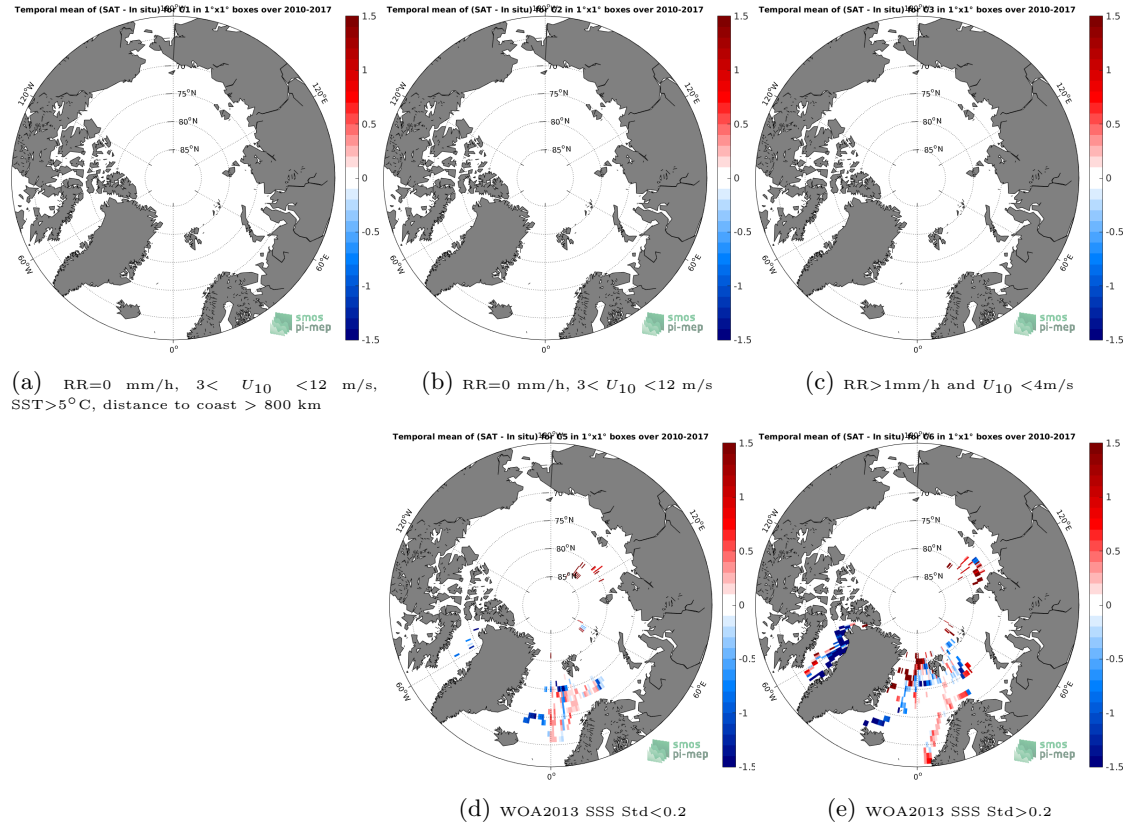
Figure 12: Temporal mean gridded over spatial boxes of size 1^\circ \times 1^\circ of \Delta SSS (SMOS-L3-CATDS-CECOS-LOCEAN-V3-18DAYS-25KM - TSG-POLARSTERN) for 5 different subdatasets corresponding to: RR=0 mm/h, 3 < U_{10} < 12 m/s, SST > 5^\circ\text{C} , distance to coast > 800 km (a), RR=0 mm/h, 3 < U_{10} < 12 m/s (b), RR > 1 mm/h and U_{10} < 4 m/s (c), WOA2013 SSS Std < 0.2 (d), WOA2013 SSS Std > 0.2 (e).
