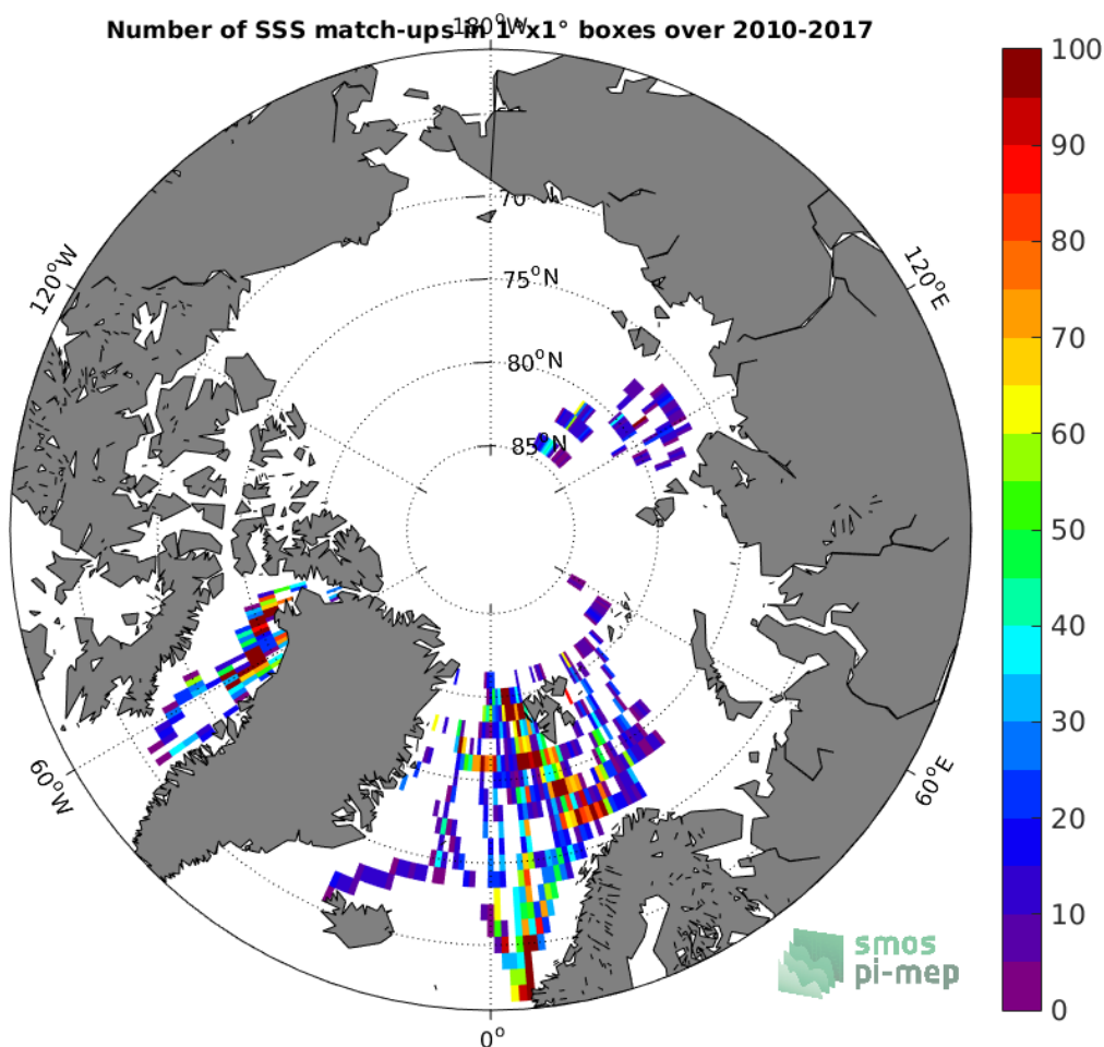
Figure 4: Number of SSS match-ups between TSG-POLARSTERN SSS and the SMOS-L3-CATDS-CECOS-LOCEAN-V3-18DAYS-25KM SSS product for the Arctic Ocean Pi-MEP region over 1°x1° boxes and for the full satellite product period.
