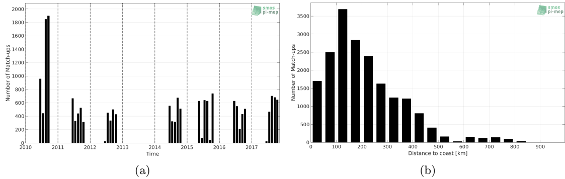
Figure 1: Number of match-ups between TSG-POLARSTERN and SMOS-L3-CATDS-CECOS-LOCEAN-V3-18DAYS-25KM SSS as a function of time (a) and as function of the distance to coast (b) over the Arctic Ocean Pi-MEP region and for the full satellite product period.
