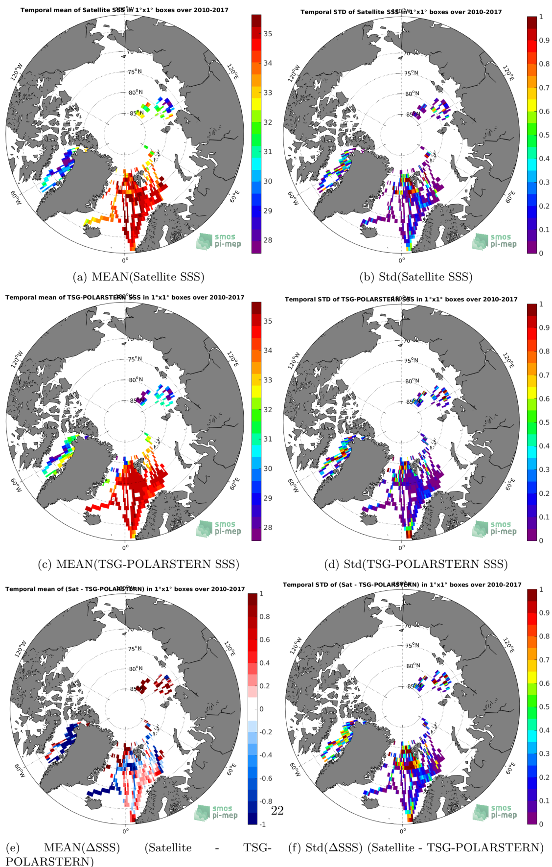
Figure 6: Temporal mean (left) and Std (right) of SSS from SMOS-L3-CATDS-CECOS-LOCEAN-V3-18DAYS-25KM (top), TSG-POLARSTERN (middle), and of \Delta SSS (Satellite - TSG-POLARSTERN). Only match-up pairs are used to generate these maps.
