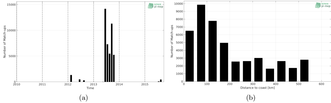
Figure 1: Number of match-ups between TSG-GOSUD-Sailing-ship and SMOS-L3-CATDS-CECOS-LOCEAN-V3-18DAYS-25KM SSS as a function of time (a) and as function of the distance to coast (b) over the Arctic Ocean Pi-MEP region and for the full satellite product period.
