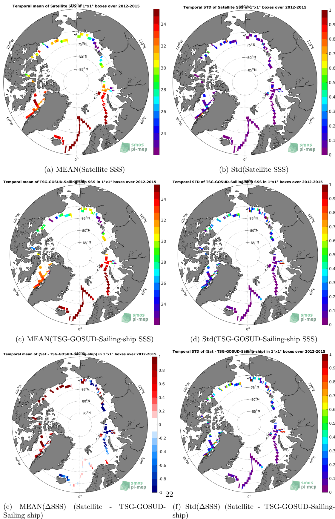
Figure 6: Temporal mean (left) and Std (right) of SSS from SMOS-L3-CATDS-CECOS-LOCEAN-V3-18DAYS-25KM (top), TSG-GOSUD-Sailing-ship (middle), and of \Delta SSS (Satellite - TSG-GOSUD-Sailing-ship). Only match-up pairs are used to generate these maps.
