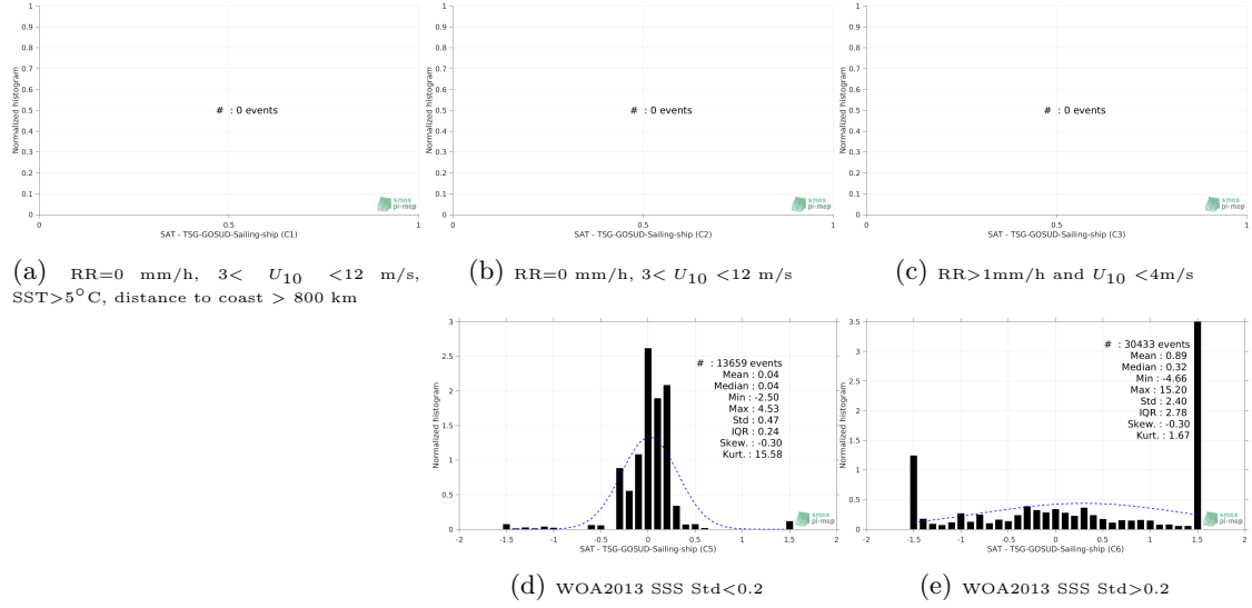
Figure 13: Normalized histogram of \Delta SSS (SMOS-L3-CATDS-CECOS-LOCEAN-V3-18DAYS-25KM - TSG-GOSUD-Sailing-ship) for 5 different subdatasets corresponding to: RR=0 mm/h, 3 < U_{10} < 12 m/s, SST>5°C, distance to coast > 800 km (a), RR=0 mm/h, 3 < U_{10} < 12 m/s (b), RR>1 mm/h and U_{10} < 4 m/s (c), WOA2013 SSS Std<0.2 (d), WOA2013 SSS Std>0.2 (e).
