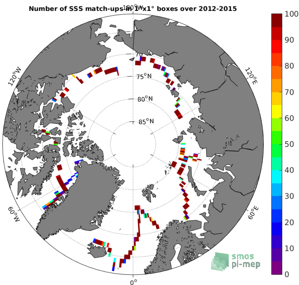
Figure 4: Number of SSS match-ups between TSG-GOSUD-Sailing-ship SSS and the SMOS-L3-CATDS-CECOS-LOCEAN-V3-18DAYS-25KM SSS product for the Arctic Ocean Pi-MEP region over 1^\circ \times 1^\circ boxes and for the full satellite product period.
