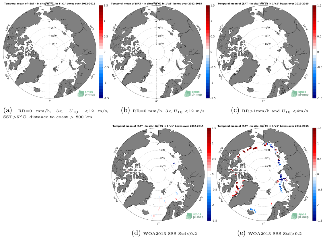
Figure 12: Temporal mean gridded over spatial boxes of size 1^\circ \times 1^\circ of \Delta SSS (SMOS-L3-CATDS-CECOS-LOCEAN-V3-18DAYS-25KM - TSG-GOSUD-Sailing-ship) for 5 different subdatasets corresponding to:RR=0 mm/h, 3 < U_{10} < 12 m/s, SST >5^\circ\text{C} , distance to coast > 800 km (a), RR=0 mm/h, 3 < U_{10} < 12 m/s (b), RR >1 mm/h and U_{10} < 4 m/s (c), WOA2013 SSS Std <0.2 (d), WOA2013 SSS Std >0.2 (e).
