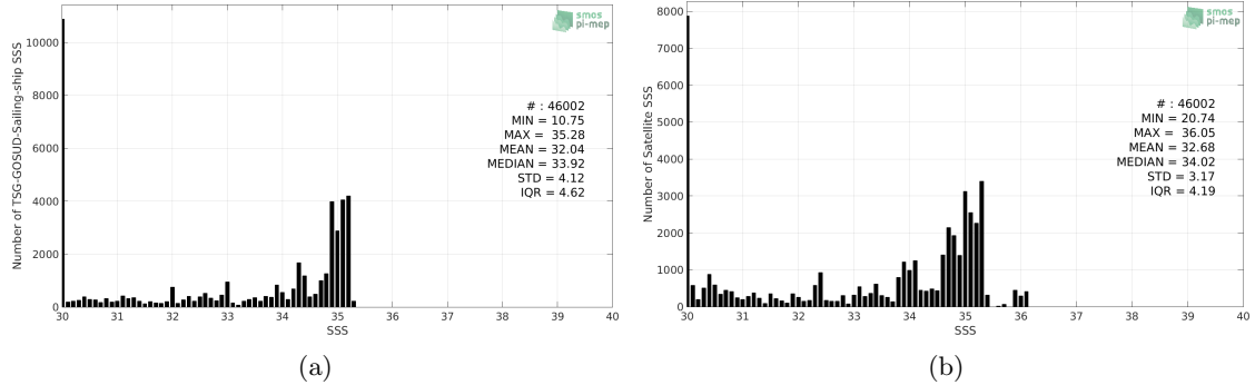
Figure 2: Histograms of SSS from TSG-GOSUD-Sailing-ship (a) and SMOS-L3-CATDS-CECOS-LOCEAN-V3-18DAYS-25KM (b) considering all match-up pairs per bins of 0.1 over the Arctic Ocean Pi-MEP region and for the full satellite product period.
