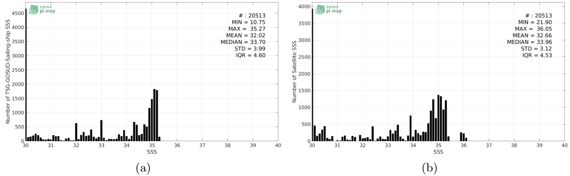
Figure 2: Histograms of SSS from TSG-GOSUD-Sailing-ship (a) and SMOS-L3-CATDS-CECOS-LOCEAN-V3-18DAYS-25KM (b) considering all match-up pairs per bins of 0.1 over the Arctic Ocean Pi-MEP region and for the full satellite product period.
