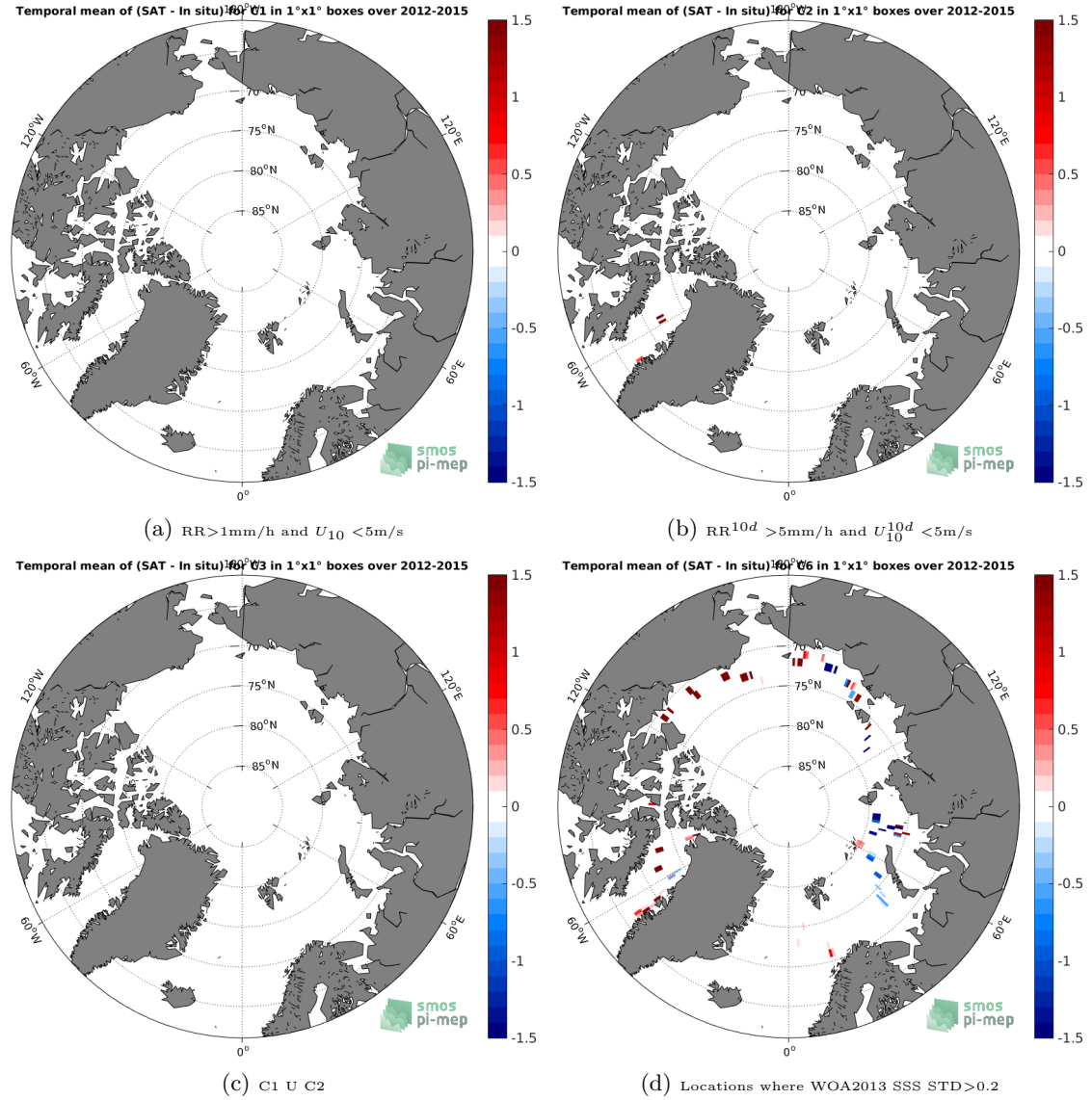
Figure 12: Temporal mean gridded over spatial boxes of size 1^\circ \times 1^\circ of \Delta SSS (SMOS-L3-CATDS-CECOS-LOCEAN-V3-18DAYS-25KM - TSG-GOSUD-Sailing-ship) for 4 different subdatasets corresponding to: RR > 1\text{mm/h} and U_{10} < 5\text{m/s} (a), RR^{10d} > 5\text{mm/h} and U_{10}^{10d} < 5\text{m/s} (b), C1 U C2 (c), Locations where WOA2013 SSS STD > 0.2 (d).
