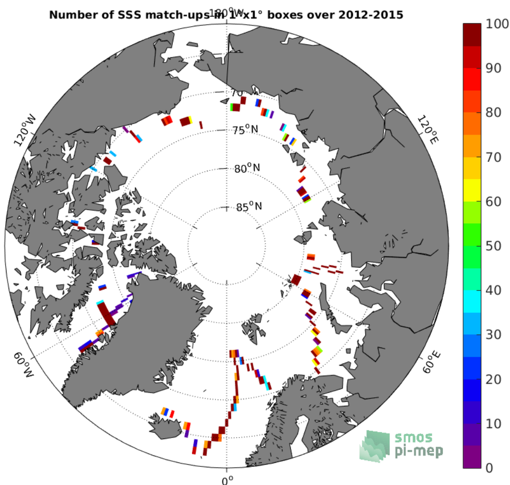
Figure 4: Number of SSS match-ups between TSG-GOSUD-Sailing-ship SSS and the SMOS-L3-CATDS-CECOS-LOCEAN-V3-18DAYS-25KM SSS product for the Arctic Ocean Pi-MEP region over 1°x1° boxes and for the full satellite product period.
