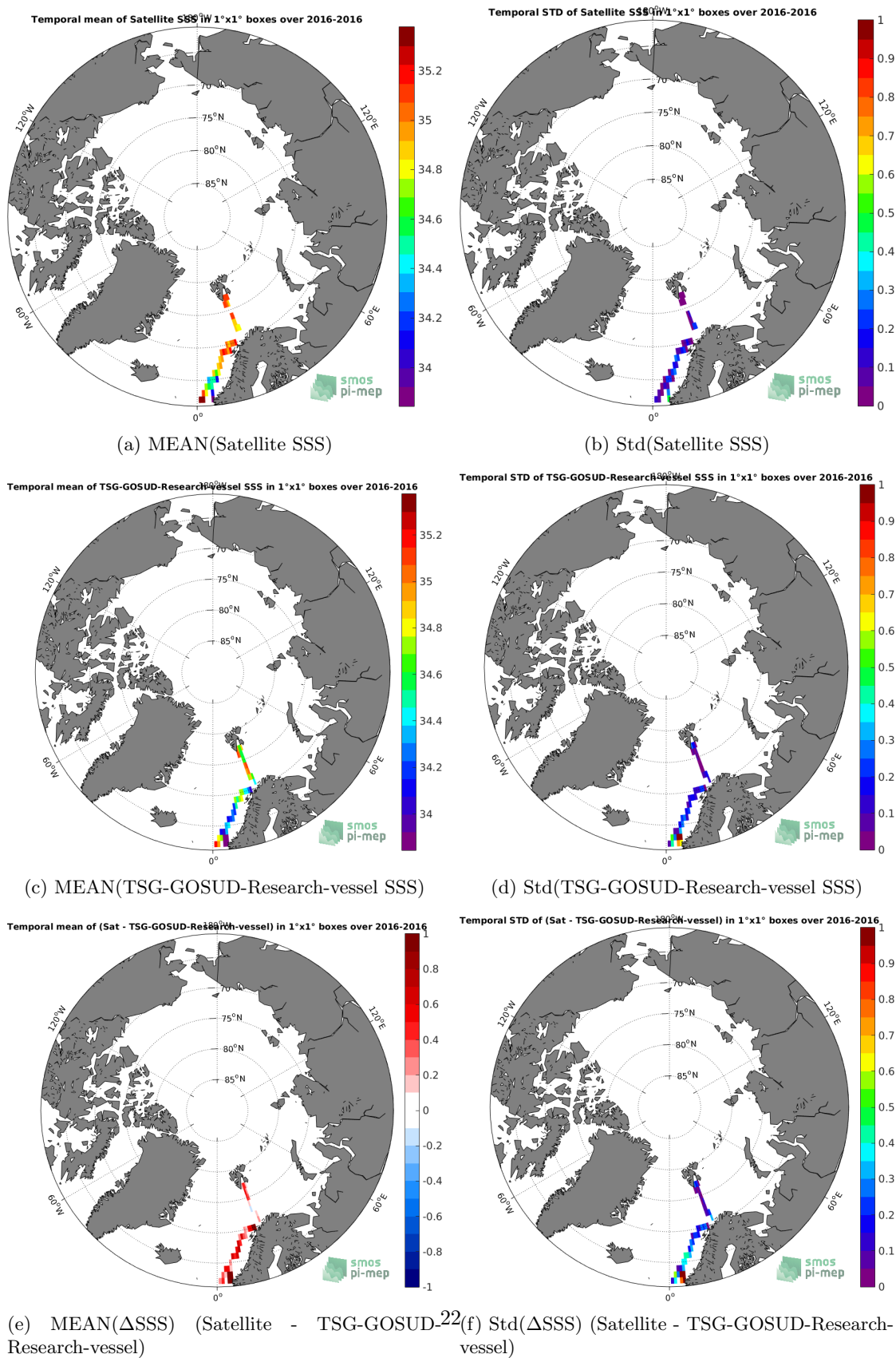
Figure 6: Temporal mean (left) and Std (right) of SSS from SMOS-L3-CATDS-CECOS-LOCEAN-V3-18DAYS-25KM (top), TSG-GOSUD-Research-vessel (middle), and of \Delta SSS (Satellite - TSG-GOSUD-Research-vessel). Only match-up pairs are used to generate these maps.
