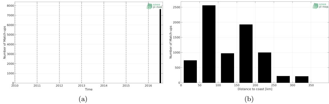
Figure 1: Number of match-ups between TSG-GOSUD-Research-vessel and SMOS-L3-CATDS-CECOS-LOCEAN-V3-18DAYS-25KM SSS as a function of time (a) and as function of the distance to coast (b) over the Arctic Ocean Pi-MEP region and for the full satellite product period.
