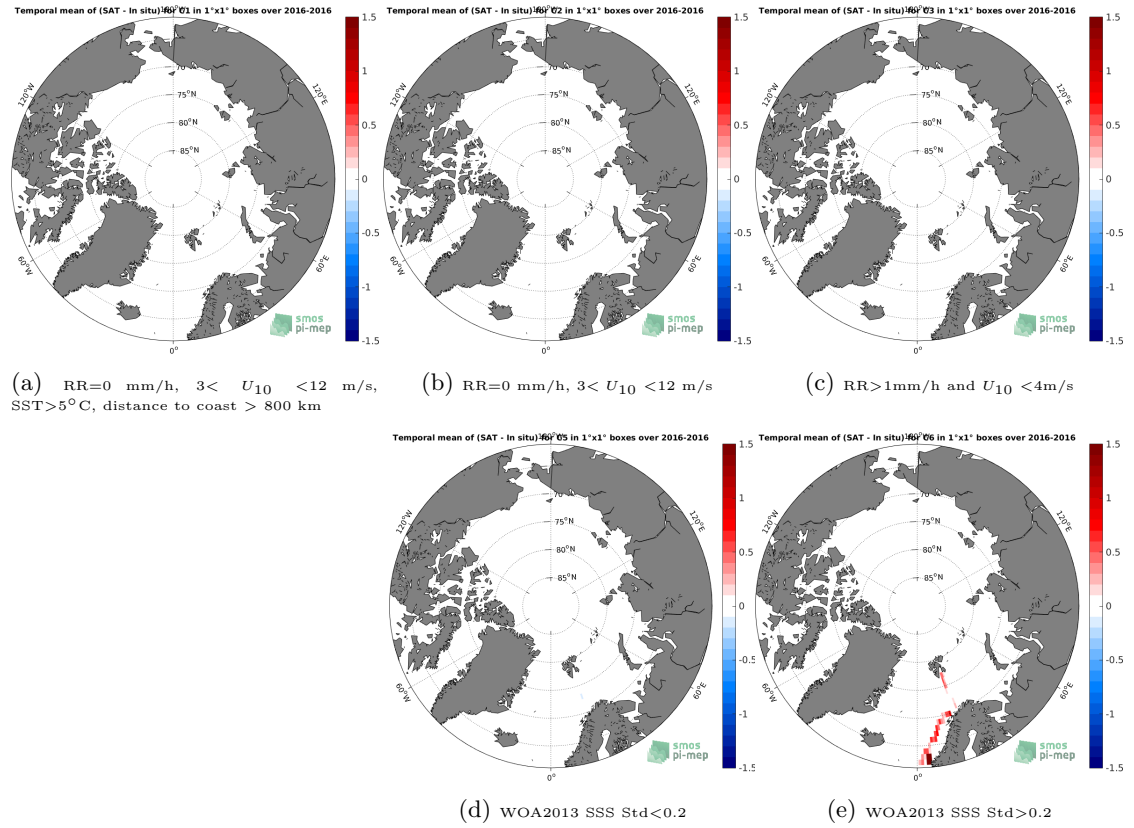
Figure 12: Temporal mean gridded over spatial boxes of size 1^\circ \times 1^\circ of \Delta SSS (SMOS-L3-CATDS-CECOS-LOCEAN-V3-18DAYS-25KM - TSG-GOSUD-Research-vessel) for 5 different subdatasets corresponding to:RR=0 mm/h, 3 < U_{10} < 12 m/s, SST >5^\circ\text{C} , distance to coast > 800 km (a), RR=0 mm/h, 3 < U_{10} < 12 m/s (b), RR >1 mm/h and U_{10} < 4 m/s (c), WOA2013 SSS Std <0.2 (d), WOA2013 SSS Std >0.2 (e).
