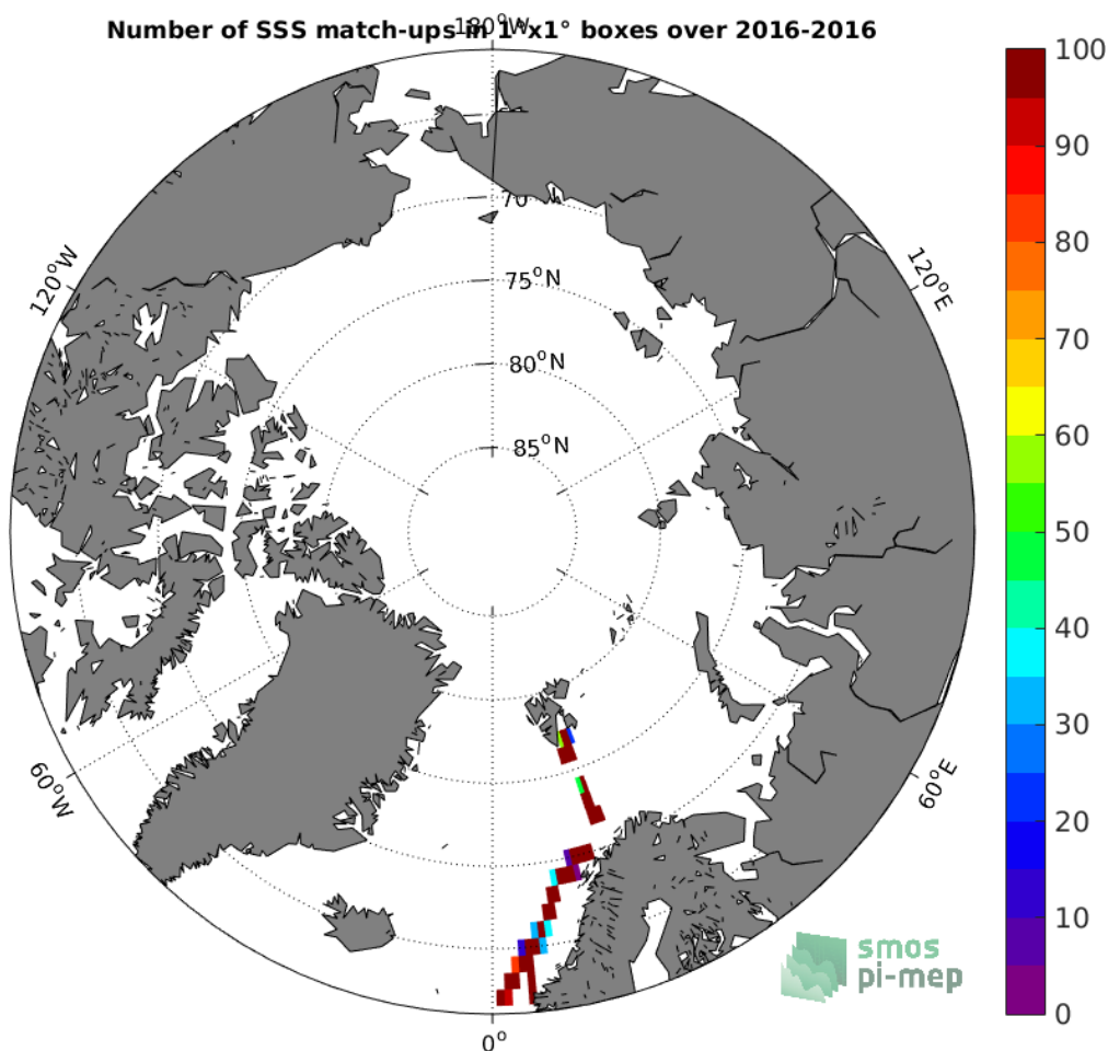
Figure 4: Number of SSS match-ups between TSG-GOSUD-Research-vessel SSS and the SMOS-L3-CATDS-CECOS-LOCEAN-V3-18DAYS-25KM SSS product for the Arctic Ocean Pi-MEP region over 1°x1° boxes and for the full satellite product period.
