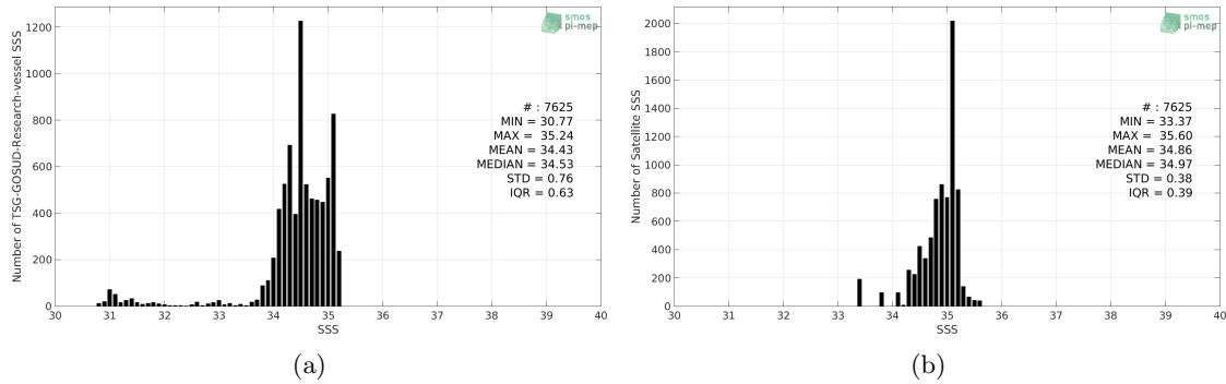
Figure 2: Histograms of SSS from TSG-GOSUD-Research-vessel (a) and SMOS-L3-CATDS-CECOS-LOCEAN-V3-18DAYS-25KM (b) considering all match-up pairs per bins of 0.1 over the Arctic Ocean Pi-MEP region and for the full satellite product period.
