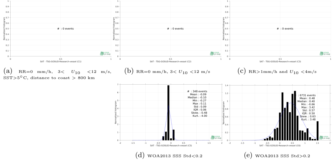
Figure 13: Normalized histogram of \Delta\text{SSS} (SMOS-L3-CATDS-CECOS-LOCEAN-V3-18DAYS-25KM - TSG-GOSUD-Research-vessel) for 5 different subdatasets corresponding to: RR=0 mm/h, 3 < U_{10} < 12 m/s, SST > 5^\circ\text{C} , distance to coast > 800 km (a), RR=0 mm/h, 3 < U_{10} < 12 m/s (b), RR > 1\text{mm/h} and U_{10} < 4\text{m/s} (c), WOA2013 SSS Std<0.2 (d), WOA2013 SSS Std>0.2 (e).
