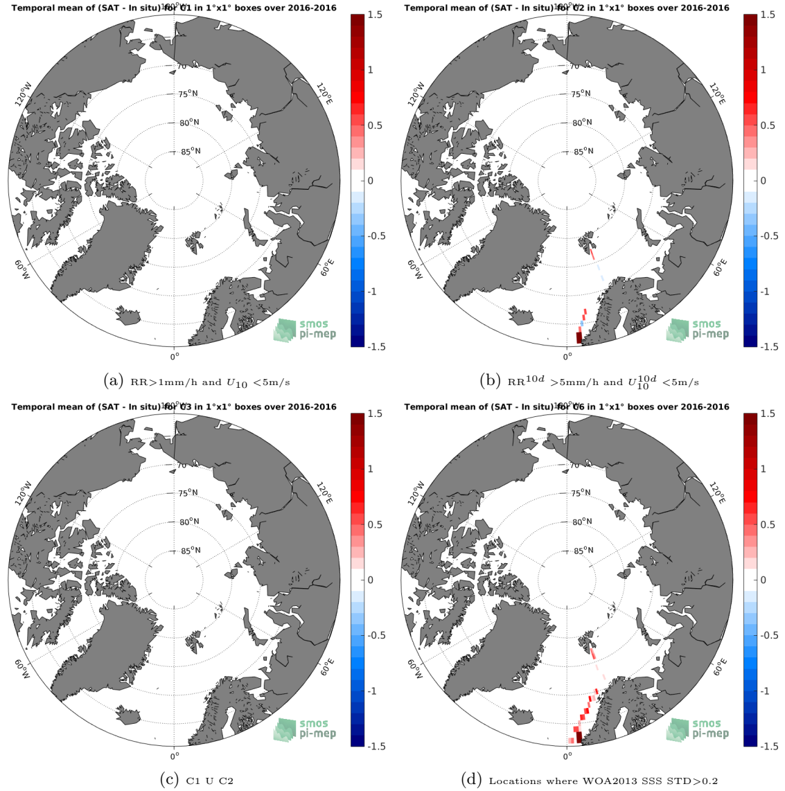
Figure 12: Temporal mean gridded over spatial boxes of size 1^\circ \times 1^\circ of \Delta SSS (SMOS-L3-CATDS-CECOS-LOCEAN-V3-18DAYS-25KM - TSG-GOSUD-Research-vessel) for 4 different subdatasets corresponding to: RR > 1\text{mm/h} and U_{10} < 5\text{m/s} (a), RR^{10d} > 5\text{mm/h} and U_{10}^{10d} < 5\text{m/s} (b), C1 U C2 (c), Locations where WOA2013 SSS STD > 0.2 (d).
