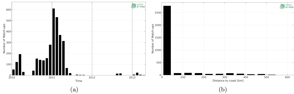
Figure 1: Number of match-ups between Sea mammals and SMOS-L3-CATDS-CECOS-LOCEAN-V3-18DAYS-25KM SSS as a function of time (a) and as function of the distance to coast (b) over the Arctic Ocean Pi-MEP region and for the full satellite product period.
