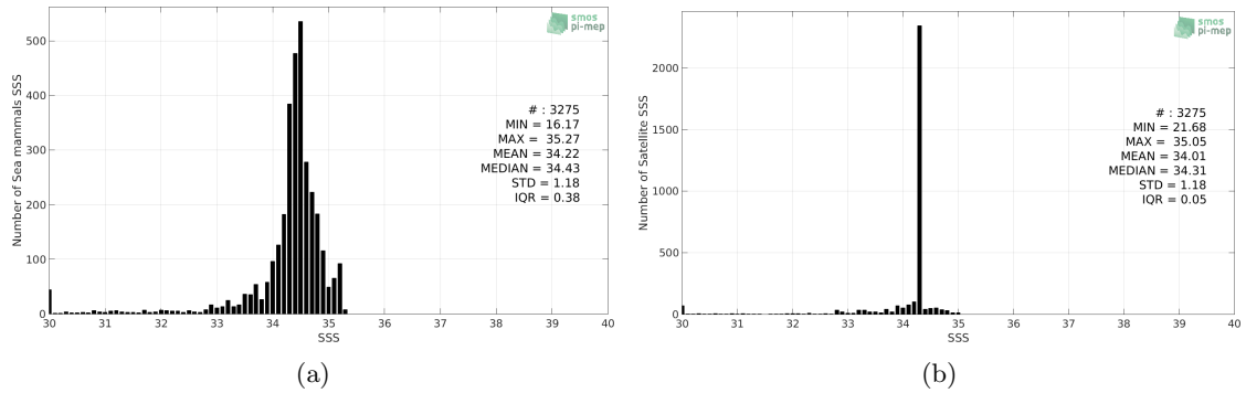
Figure 2: Histograms of SSS from Sea mammals (a) and SMOS-L3-CATDS-CECOS-LOCEAN-V3-18DAYS-25KM (b) considering all match-up pairs per bins of 0.1 over the Arctic Ocean Pi-MEP region and for the full satellite product period.
