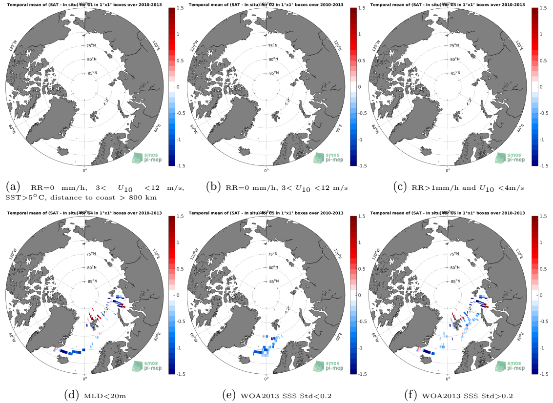
Figure 12: Temporal mean gridded over spatial boxes of size 1^\circ \times 1^\circ of \Delta SSS (SMOS-L3-CATDS-CECOS-LOCEAN-V3-18DAYS-25KM - Sea mammals) for 6 different subdatasets corresponding to: RR=0 mm/h, 3 < U_{10} < 12 m/s, SST > 5^\circ C , distance to coast > 800 km (a), RR=0 mm/h, 3 < U_{10} < 12 m/s (b), RR > 1 mm/h and U_{10} < 4 m/s (c), MLD < 20 m (d), WOA2013 SSS Std < 0.2 (e), WOA2013 SSS Std > 0.2 (f).
