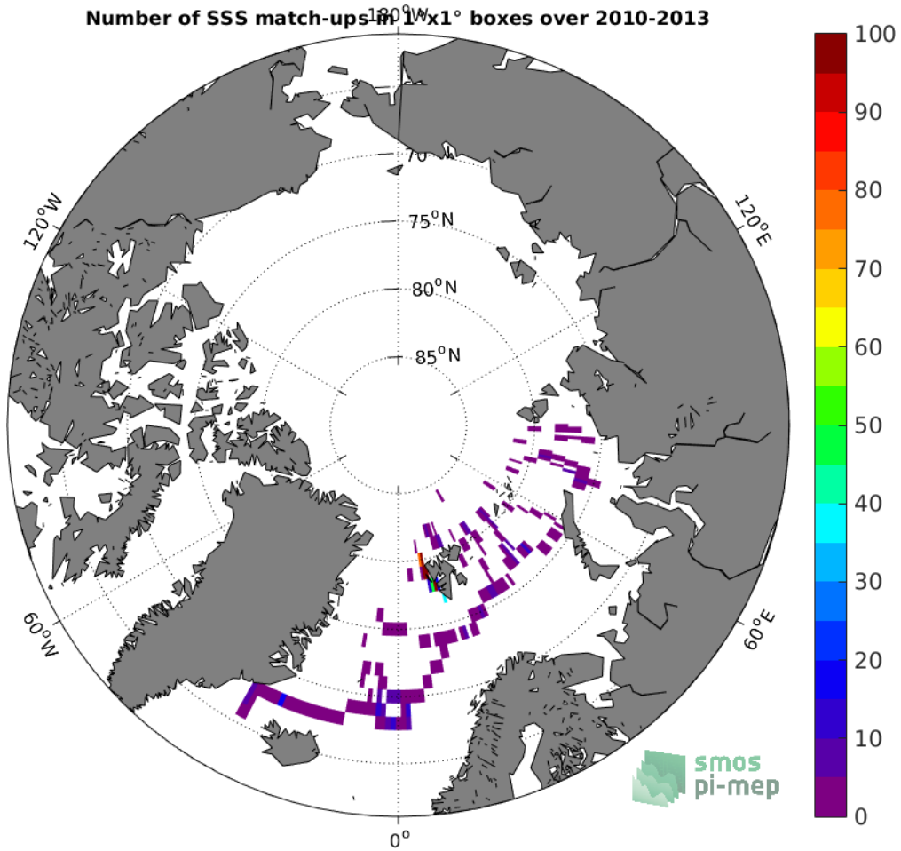
Figure 4: Number of SSS match-ups between Sea mammals SSS and the SMOS-L3-CATDS-CECOS-LOCEAN-V3-18DAYS-25KM SSS product for the Arctic Ocean Pi-MEP region over 1^\circ \times 1^\circ boxes and for the full satellite product period.
