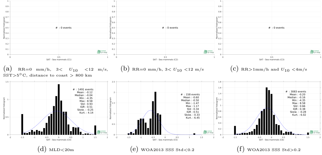
Figure 13: Normalized histogram of \Delta\text{SSS} (SMOS-L3-CATDS-CECOS-LOCEAN-V3-18DAYS-25KM - Sea mammals) for 6 different subdatasets corresponding to: RR=0 mm/h, 3 < U_{10} < 12 m/s, SST > 5^{\circ}\text{C} , distance to coast > 800 km (a), RR=0 mm/h, 3 < U_{10} < 12 m/s (b), RR > 1\text{mm/h} and U_{10} < 4\text{m/s} (c), MLD < 20\text{m} (d), WOA2013 SSS Std < 0.2 (e), WOA2013 SSS Std > 0.2 (f).
