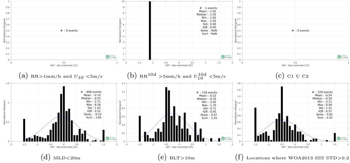
Figure 13: Normalized histogram of \Delta SSS (SMOS-L3-CATDS-CECOS-LOCEAN-V3-18DAYS-25KM - Sea mammals) for 6 different subdatasets corresponding to: RR>1mm/h and U_{10} < 5\text{m/s} (a), RR^{10d} > 5\text{mm/h} and U_{10}^{10d} < 5\text{m/s} (b), C1 U C2 (c), MLD<20m (d), BLT>10m (e), Locations where WOA2013 SSS STD>0.2 (f).
