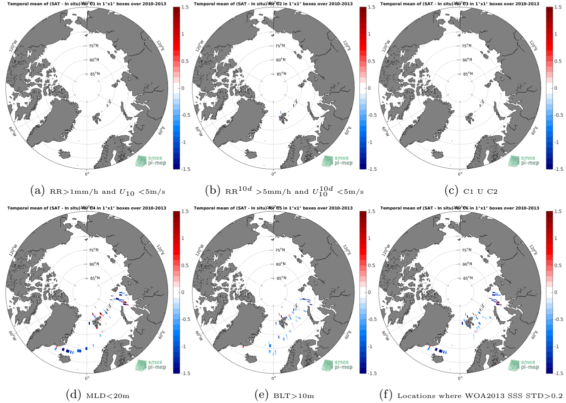
Figure 12: Temporal mean gridded over spatial boxes of size 1^\circ \times 1^\circ of \Delta\text{SSS} (SMOS-L3-CATDS-CECOS-LOCEAN-V3-18DAYS-25KM - Sea mammals) for 6 different subdatasets corresponding to: \text{RR} > 1\text{mm/h} and U_{10} < 5\text{m/s} (a), \text{RR}^{10d} > 5\text{mm/h} and U_{10}^{10d} < 5\text{m/s} (b), C1 U C2 (c), \text{MLD} < 20\text{m} (d), \text{BLT} > 10\text{m} (e), Locations where WOA2013 SSS STD > 0.2 (f).
