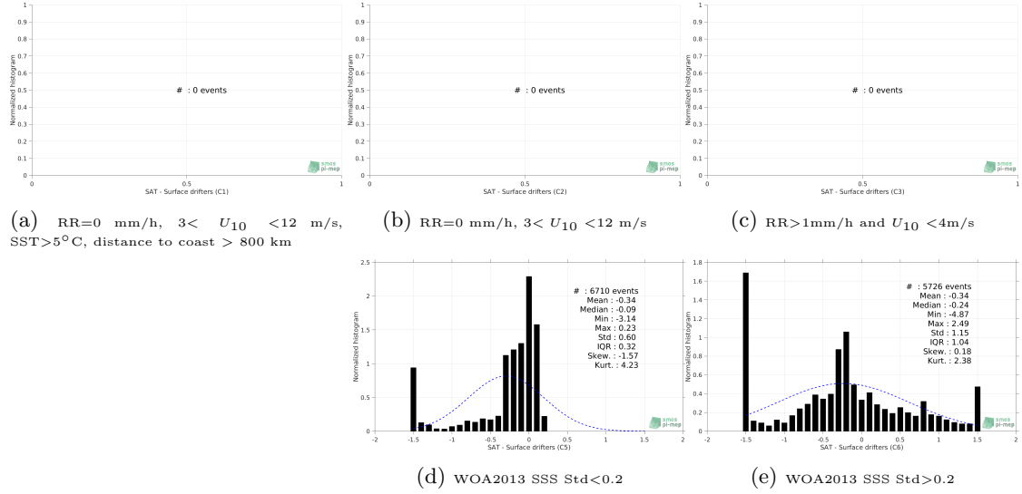
Figure 12: Normalized histogram of \Delta\text{SSS} (SMOS-L3-CATDS-CECOS-LOCEAN-V3-18DAYS-25KM - Surface drifters) for 5 different subdatasets corresponding to: RR=0 mm/h, 3 < U_{10} < 12 m/s, SST >5^{\circ}\text{C} , distance to coast > 800 km (a), RR=0 mm/h, 3 < U_{10} < 12 m/s (b), RR>1\text{mm/h} and U_{10} < 4\text{m/s} (c), WOA2013 SSS Std <0.2 (d), WOA2013 SSS Std >0.2 (e).
