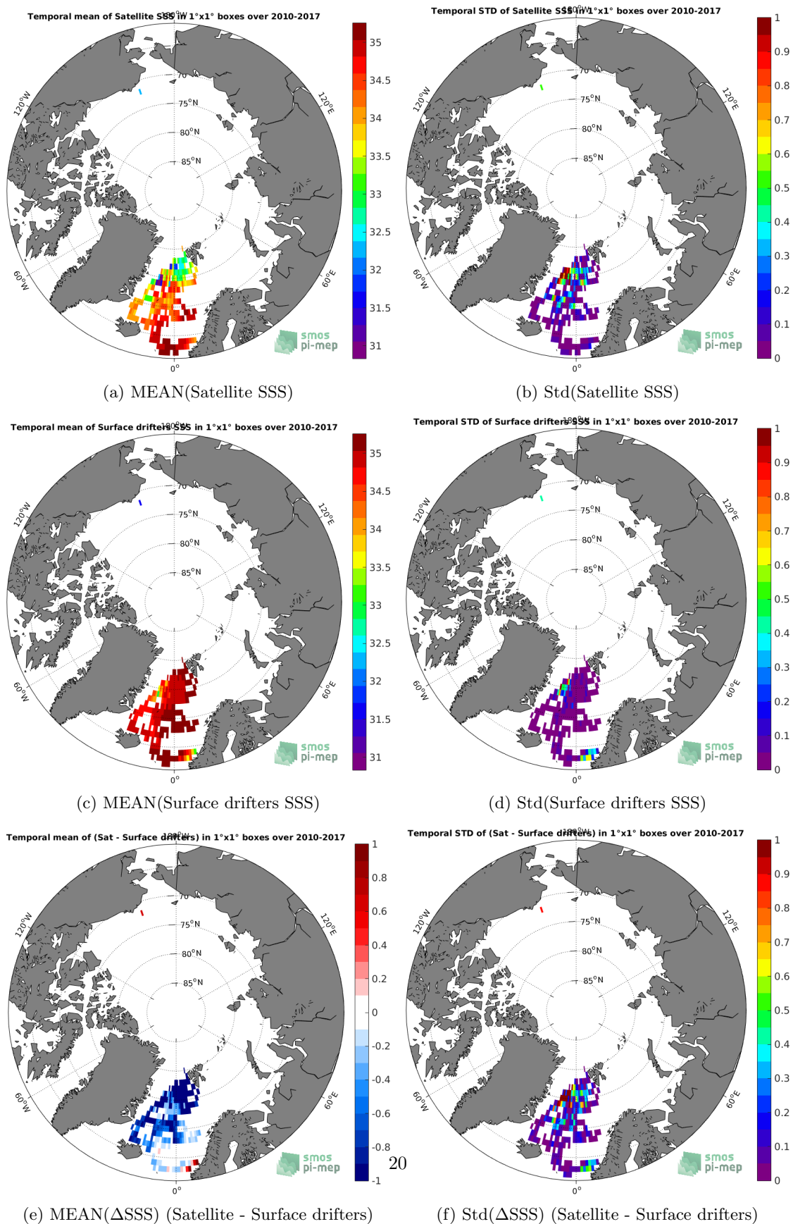
Figure 5: Temporal mean (left) and Std (right) of SSS from SMOS-L3-CATDS-CECOS-LOCEAN-V3-18DAYS-25KM (top), Surface drifters (middle), and of \Delta SSS (Satellite - Surface drifters). Only match-up pairs are used to generate these maps.
