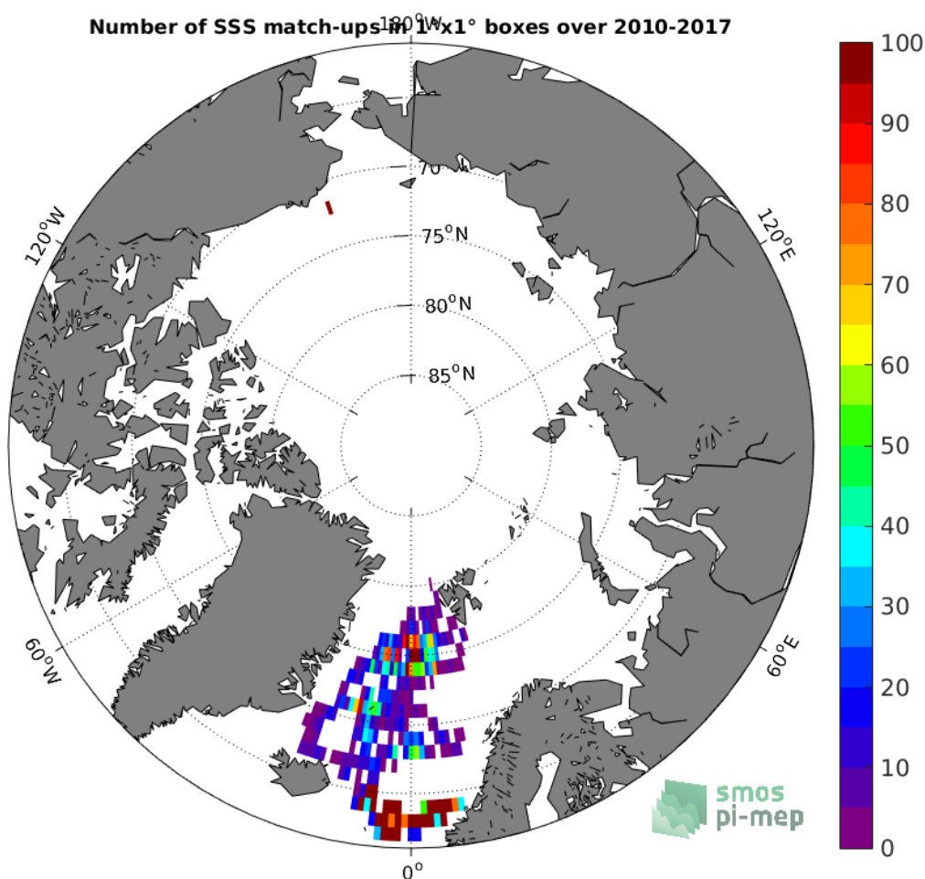
Figure 3: Number of SSS match-ups between Surface drifters SSS and the SMOS-L3-CATDS-CECOS-LOCEAN-V3-18DAYS-25KM SSS product for the Arctic Ocean Pi-MEP region over 1^\circ \times 1^\circ boxes and for the full satellite product period.
