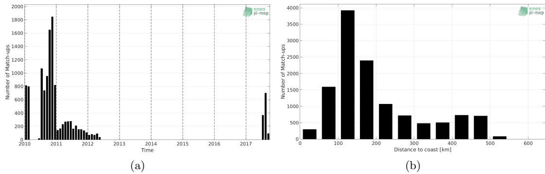
Figure 1: Number of match-ups between Surface drifters and SMOS-L3-CATDS-CECOS-LOCEAN-V3-18DAYS-25KM SSS as a function of time (a) and as function of the distance to coast (b) over the Arctic Ocean Pi-MEP region and for the full satellite product period.
