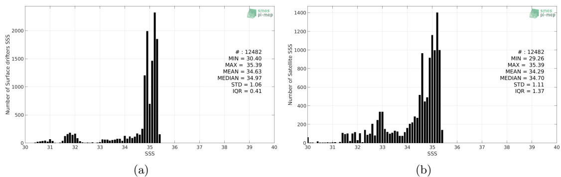
Figure 2: Histograms of SSS from Surface drifters (a) and SMOS-L3-CATDS-CECOS-LOCEAN-V3-18DAYS-25KM (b) considering all match-up pairs per bins of 0.1 over the Arctic Ocean Pi-MEP region and for the full satellite product period.
