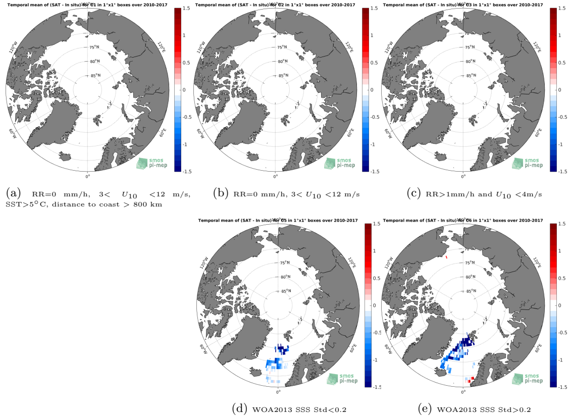
Figure 11: Temporal mean gridded over spatial boxes of size 1^\circ \times 1^\circ of \Delta SSS (SMOS-L3-CATDS-CECOS-LOCEAN-V3-18DAYS-25KM - Surface drifters) for 5 different subdatasets corresponding to: RR=0 mm/h, 3 < U_{10} < 12 m/s, SST >5^\circ\text{C} , distance to coast > 800 km (a), RR=0 mm/h, 3 < U_{10} < 12 m/s (b), RR >1 mm/h and U_{10} < 4 m/s (c), WOA2013 SSS Std <0.2 (d), WOA2013 SSS Std >0.2 (e).
