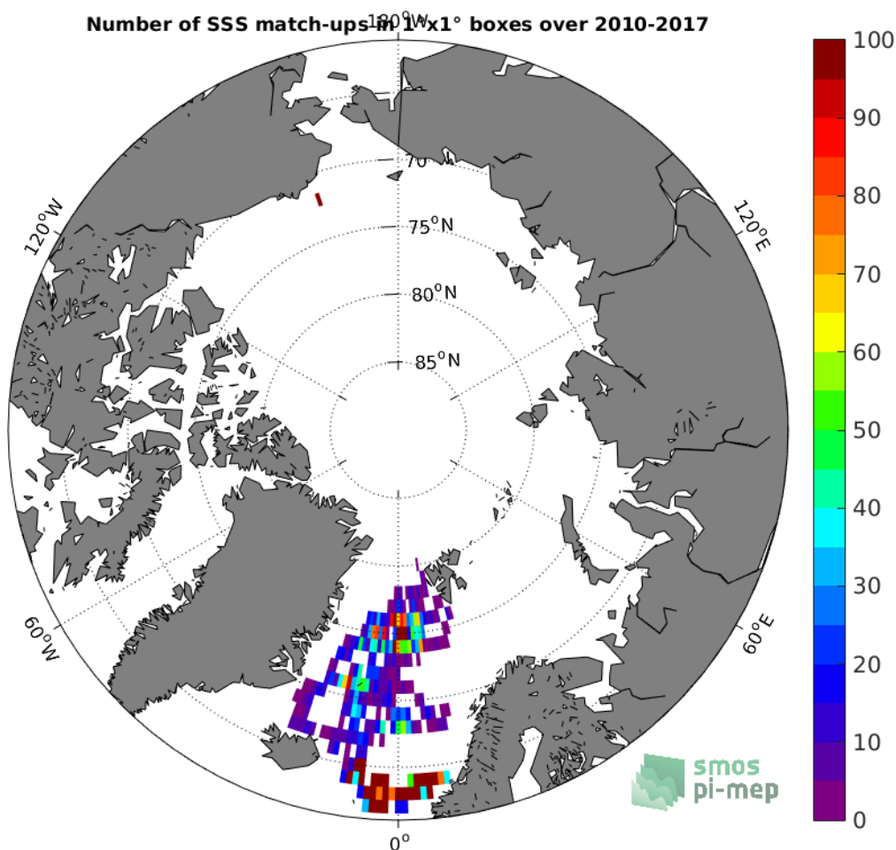
Figure 3: Number of SSS match-ups between Surface drifters SSS and the SMOS-L3-CATDS-CECOS-LOCEAN-V3-18DAYS-25KM SSS product for the Arctic Ocean Pi-MEP region over 1°x1° boxes and for the full satellite product period.
