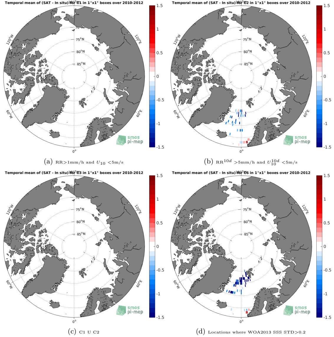
Figure 11: Temporal mean gridded over spatial boxes of size 1^\circ \times 1^\circ of \Delta SSS (SMOS-L3-CATDS-CECOS-LOCEAN-V3-18DAYS-25KM - Surface drifters) for 4 different subdatasets corresponding to: RR > 1\text{mm/h} and U_{10} < 5\text{m/s} (a), RR^{10d} > 5\text{mm/h} and U_{10}^{10d} < 5\text{m/s} (b), C1 U C2 (c), Locations where WOA2013 SSS STD > 0.2 (d).
