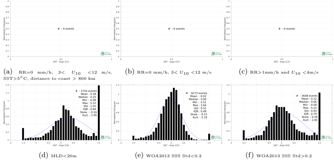
Figure 13: Normalized histogram of \Delta\text{SSS} (SMOS-L3-CATDS-CECOS-LOCEAN-V3-18DAYS-25KM - Argo) for 6 different subdatasets corresponding to: RR=0 mm/h, 3 < U_{10} < 12 m/s, SST > 5^\circ\text{C} , distance to coast > 800 km (a), RR=0 mm/h, 3 < U_{10} < 12 m/s (b), RR > 1\text{mm/h} and U_{10} < 4\text{m/s} (c), MLD < 20\text{m} (d), WOA2013 SSS Std < 0.2 (e), WOA2013 SSS Std > 0.2 (f).
