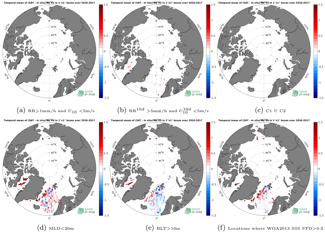
Figure 12: Temporal mean gridded over spatial boxes of size 1^\circ \times 1^\circ of \Delta SSS (SMOS-L3-CATDS-CECOS-LOCEAN-V3-18DAYS-25KM - Argo) for 6 different subdatasets corresponding to: RR > 1mm/h and U_{10} < 5 m/s (a), RR^{10d} > 5 mm/h and U_{10}^{10d} < 5 m/s (b), C1 U C2 (c), MLD < 20m (d), BLT > 10m (e), Locations where WOA2013 SSS STD > 0.2 (f).
