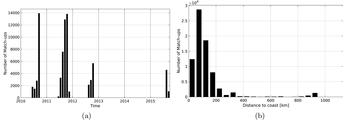
Figure 1: Number of match-ups between TSG-SAMOS and SMOS-L3-CATDS-CECOS-LOCEAN-V2-9DAYS-25KM SSS as a function of time (a) and as function of the distance to coast (b) over the Arctic Ocean Pi-MEP region and for the full satellite product period.
