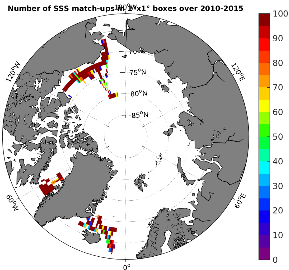
Figure 4: Number of SSS match-ups between TSG-SAMOS SSS and the SMOS-L3-CATDS-CECOS-LOCEAN-V2-9DAYS-25KM SSS product for the Arctic Ocean Pi-MEP region over 1^\circ \times 1^\circ boxes and for the full satellite product period.
