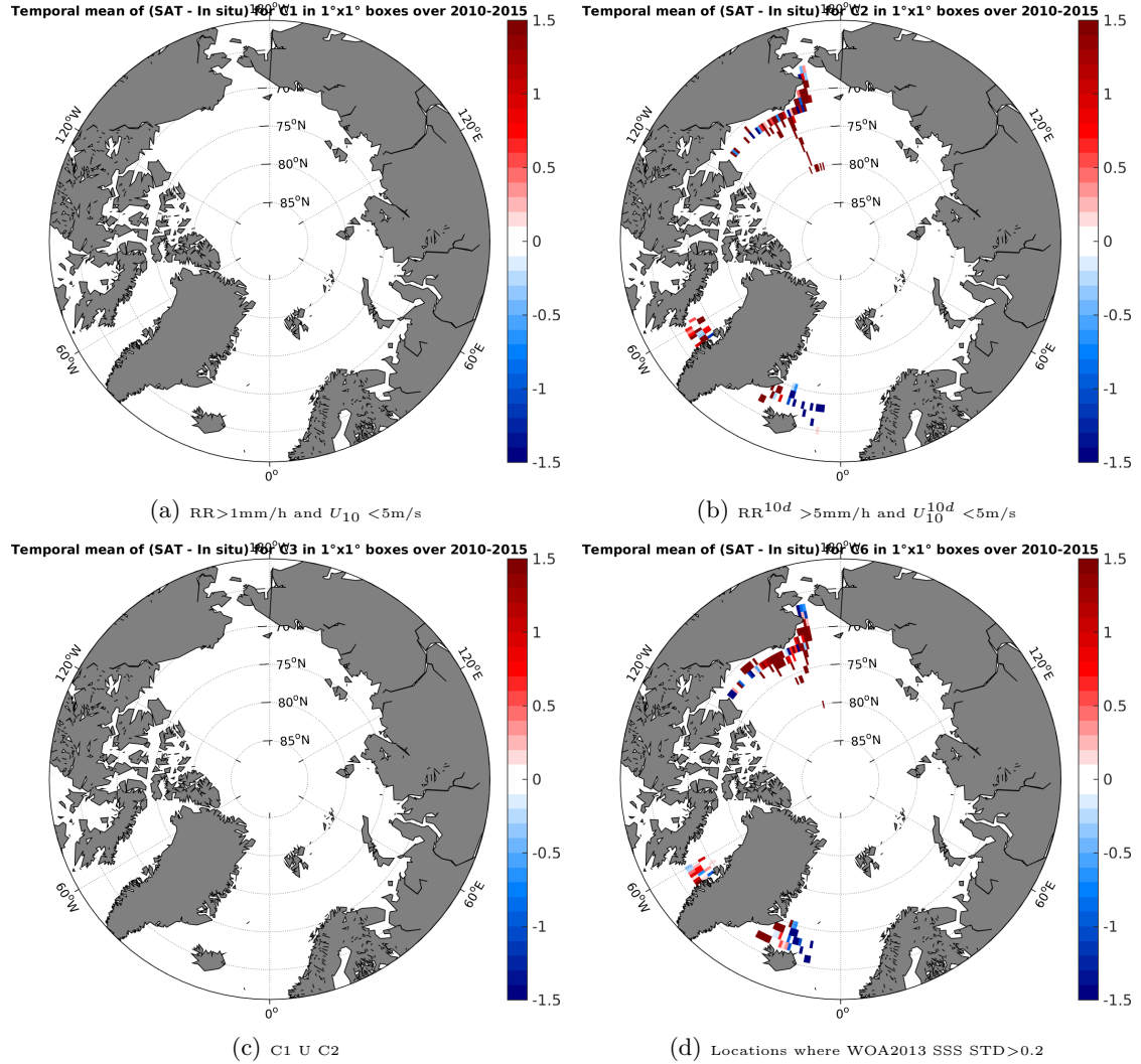
Figure 12: Temporal mean gridded over spatial boxes of size 1^\circ \times 1^\circ of \Delta SSS (SMOS-L3-CATDS-CECOS-LOCEAN-V2-9DAYS-25KM - TSG-SAMOS) for 4 different subdatasets corresponding to: RR > 1 mm/h and U_{10} < 5 m/s (a), RR^{10d} > 5 mm/h and U_{10}^{10d} < 5 m/s (b), C1 U C2 (c), Locations where WOA2013 SSS STD > 0.2 (d).
