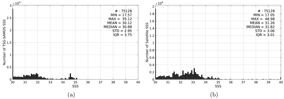
Figure 2: Histograms of SSS from TSG-SAMOS (a) and SMOS-L3-CATDS-CECOS-LOCEAN-V2-9DAYS-25KM (b) considering all match-up pairs per bins of 0.1 over the Arctic Ocean Pi-MEP region and for the full satellite product period.
